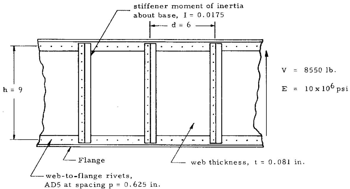
Figure 1-17. Stiffened Shear Resistant Beam
