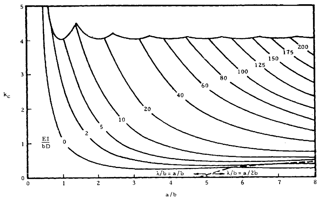
(g) Three stiffeners A/bt = 0
