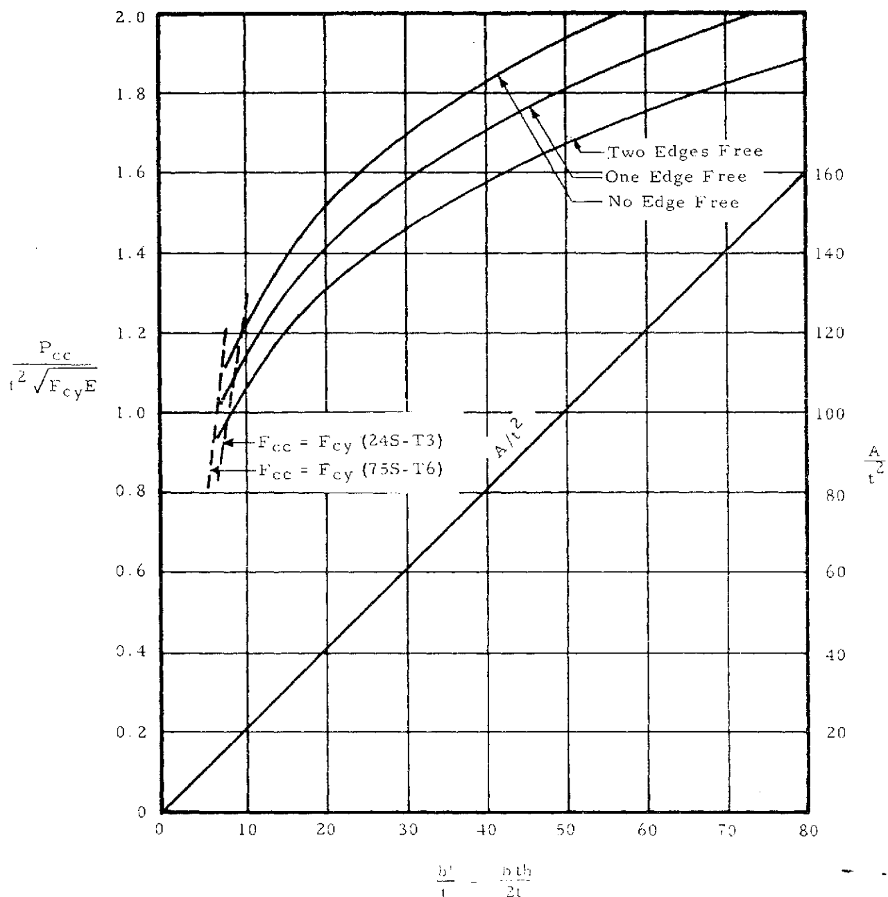
Figure 2-72. Dimensionless Crippling Load of Angle vs. b'/t
