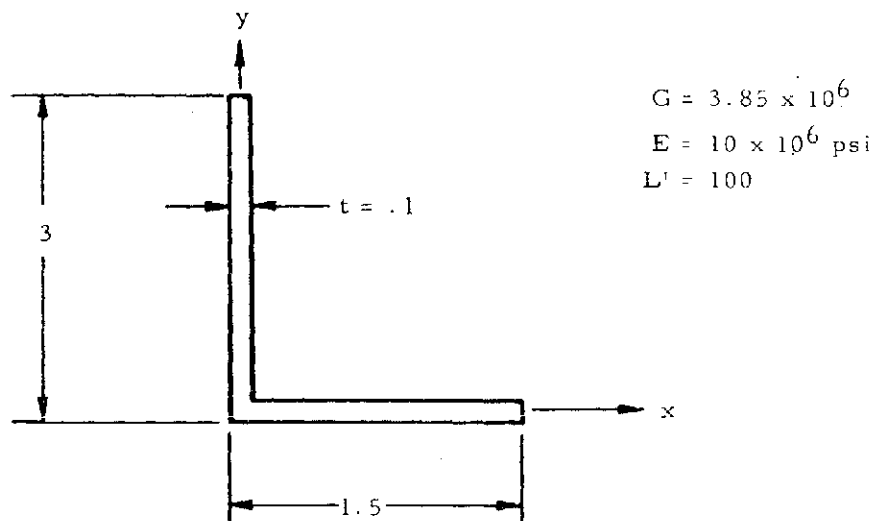
Figure 2-62. Cross Section of Column Used for Illustration of Torsional Failure
