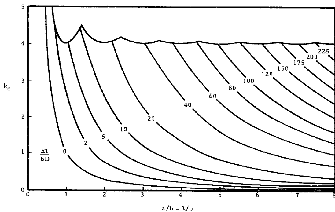
(j) Infinite number of stiffeners A/bt = 0
