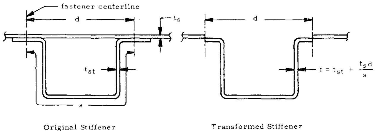
Figure 1-59. Second Method of Transforming Closed Stiffeners
