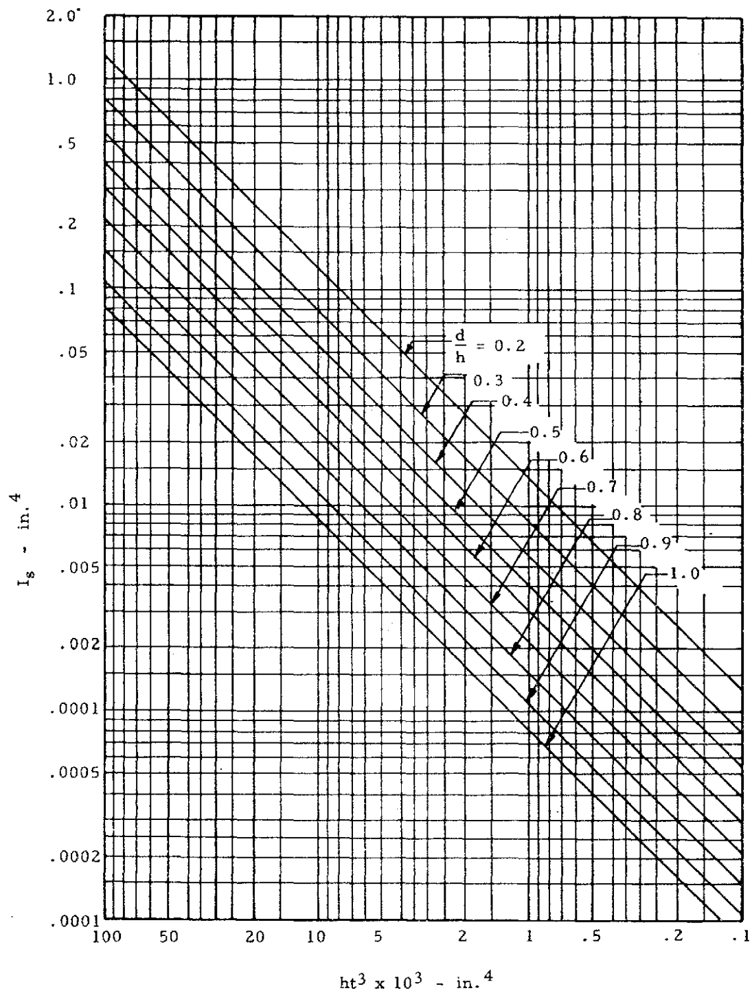
Figure 1-21. Minimum Moment of Inertia Required for Tension Field Beam Uprights Assuming Simply Supported Panels
