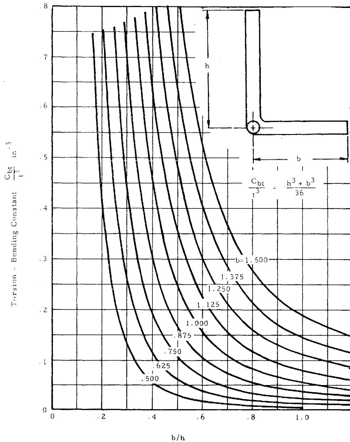
Figure 2-57. Torsion - Bending Constant of Angle - About Its Shear Center
