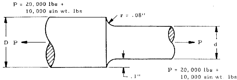
Figure 3-16. Bar Under Cyclic Tensile Load
