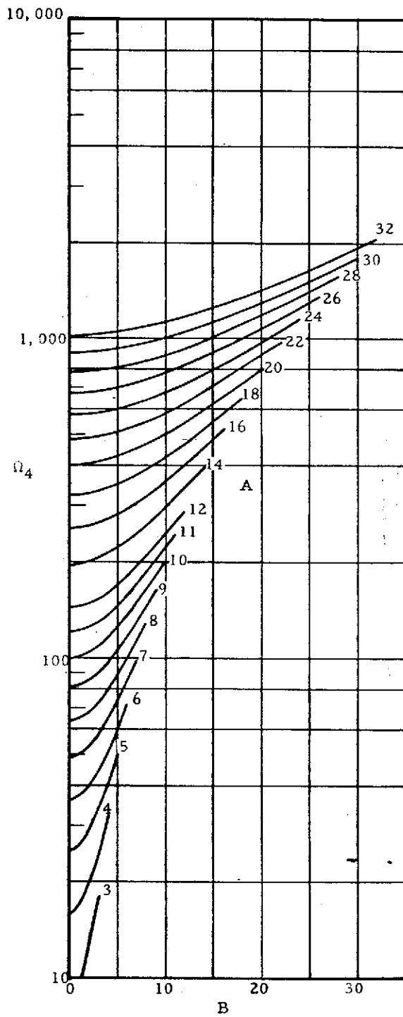
Figure 8-44. \Omega_4 as a Function of A and B
