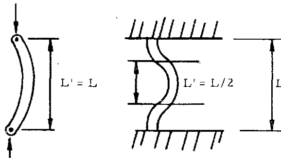
Figure 2-36. Example of Effective Length
