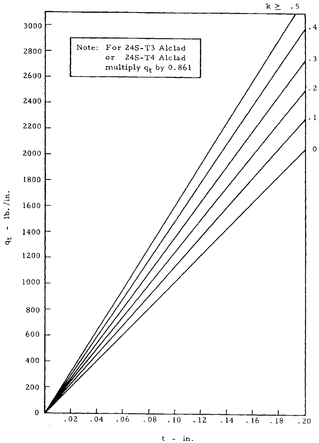
Figure 1-25. Rivet Tension Loads—Web-to-Upright 75S-T6 Alclad
