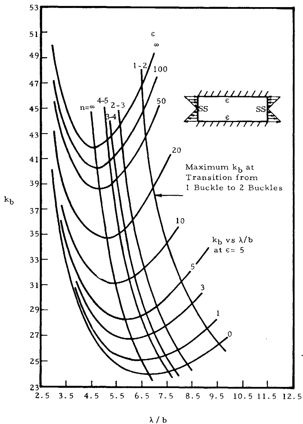
Figure 6-21. Bending-Buckling Coefficient of Plates as a Function of \lambda/b for Various Amounts of Edge Rotational Restraint
