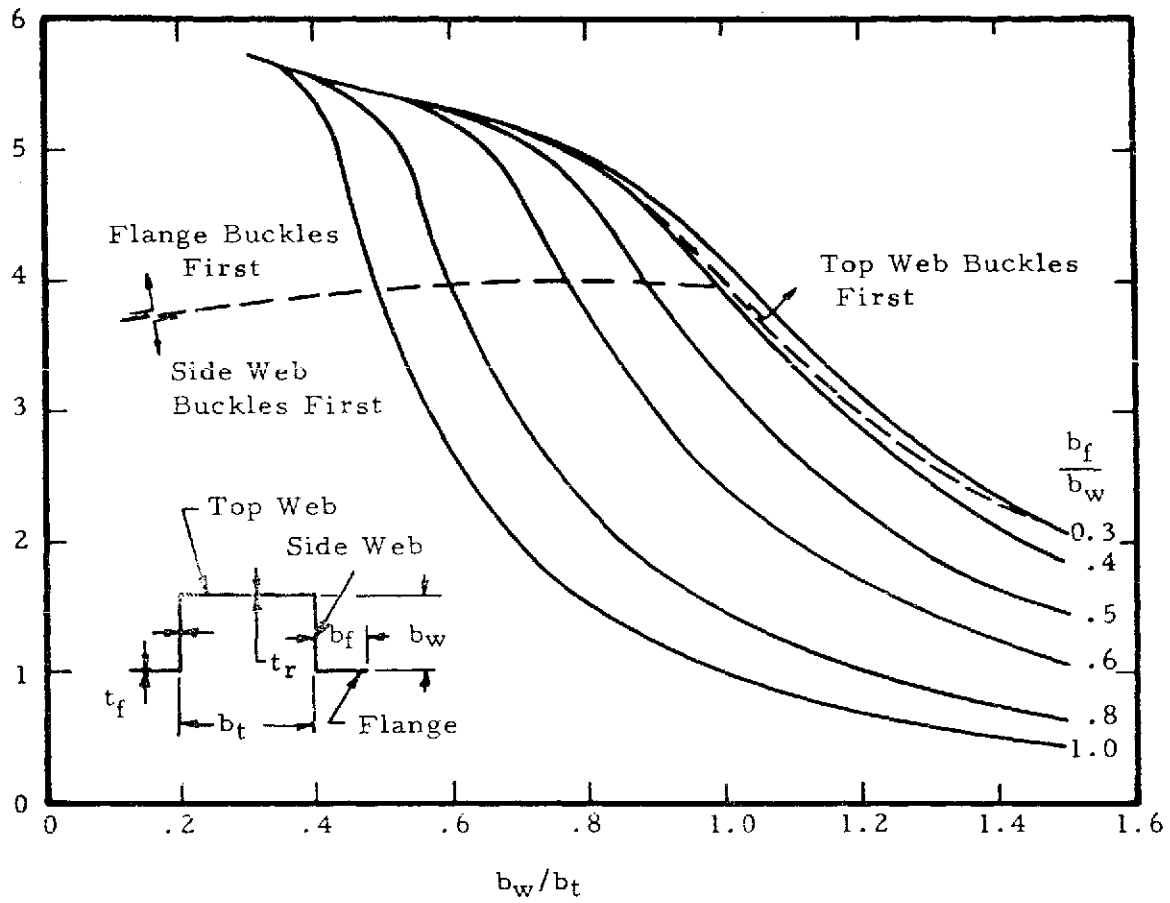
Figure 6-12. Buckling Stress for Hat-Section Stiffeners. t = t_f = t_w = t_r ;
