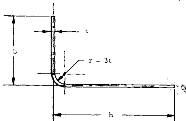
Figure 2-70. Angle Section
