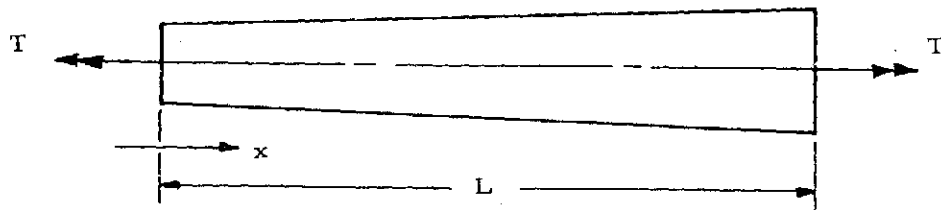
Figure 1-47. Nonuniform Circular Beam in Torsion
