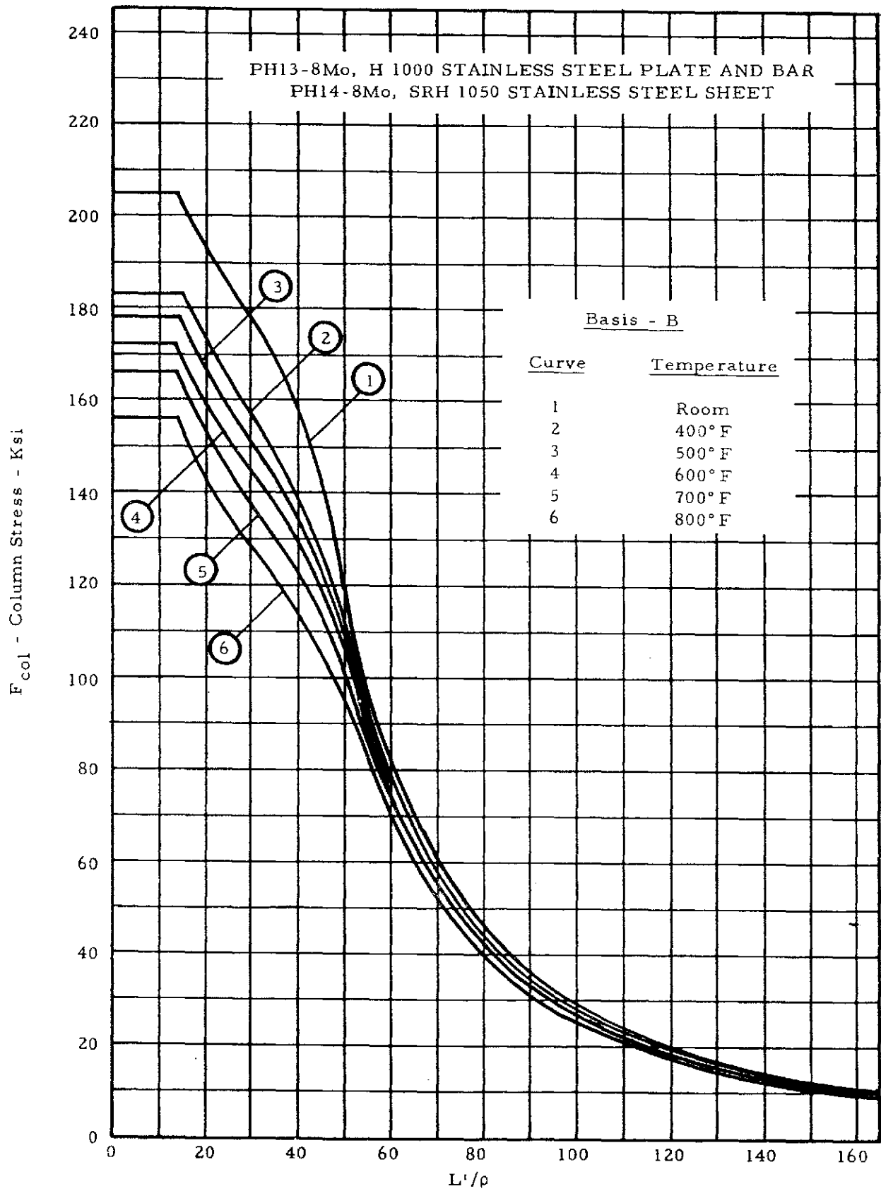
Figure 2-22. Column Allowable Curves
