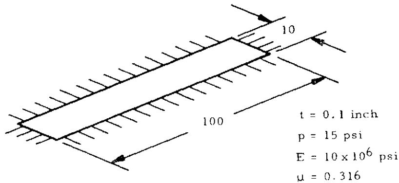
Figure 7-7. Long Rectangular Membrane
