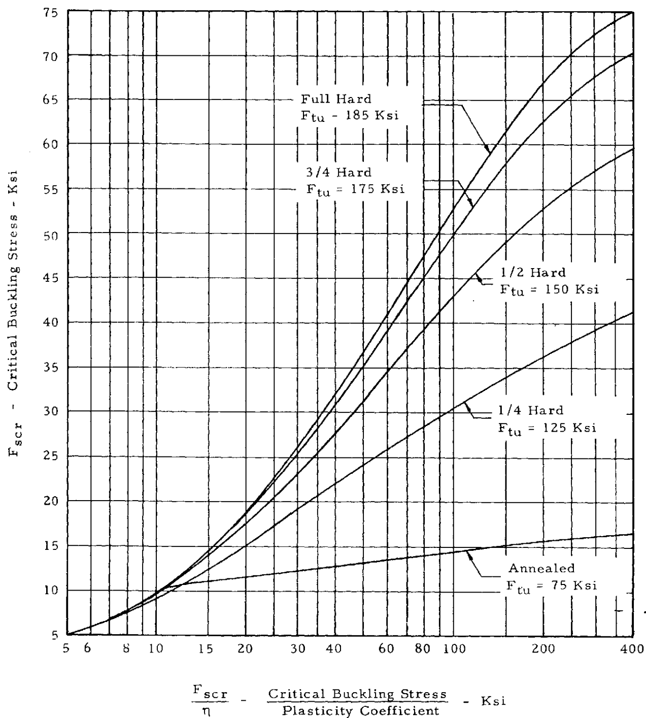
Figure 1-13. F_{scr} versus F_{scr}/\eta for Stainless Steel
