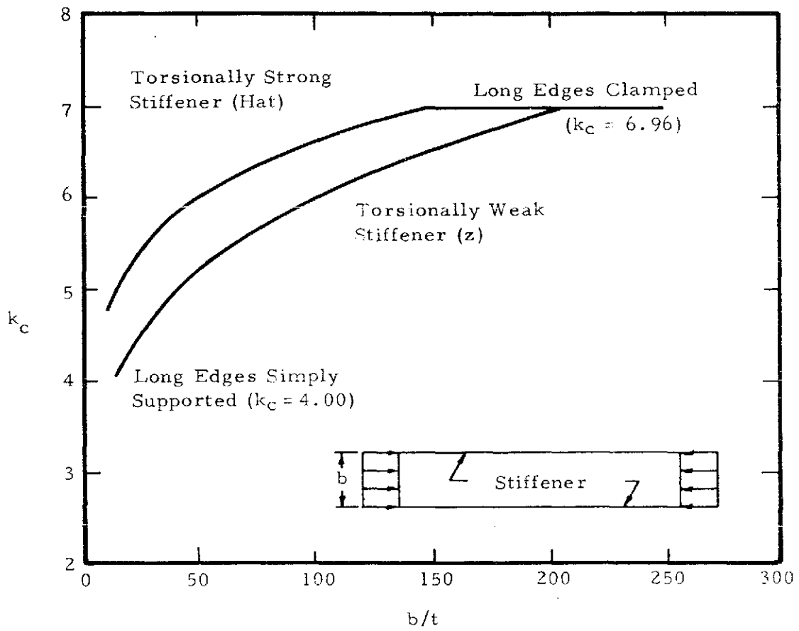
Figure 6-10. Compressive-Buckling Coefficient for Long Rectangular Stiffened Panels as a Function of b/t and Stiffener Torsional Rigidity
