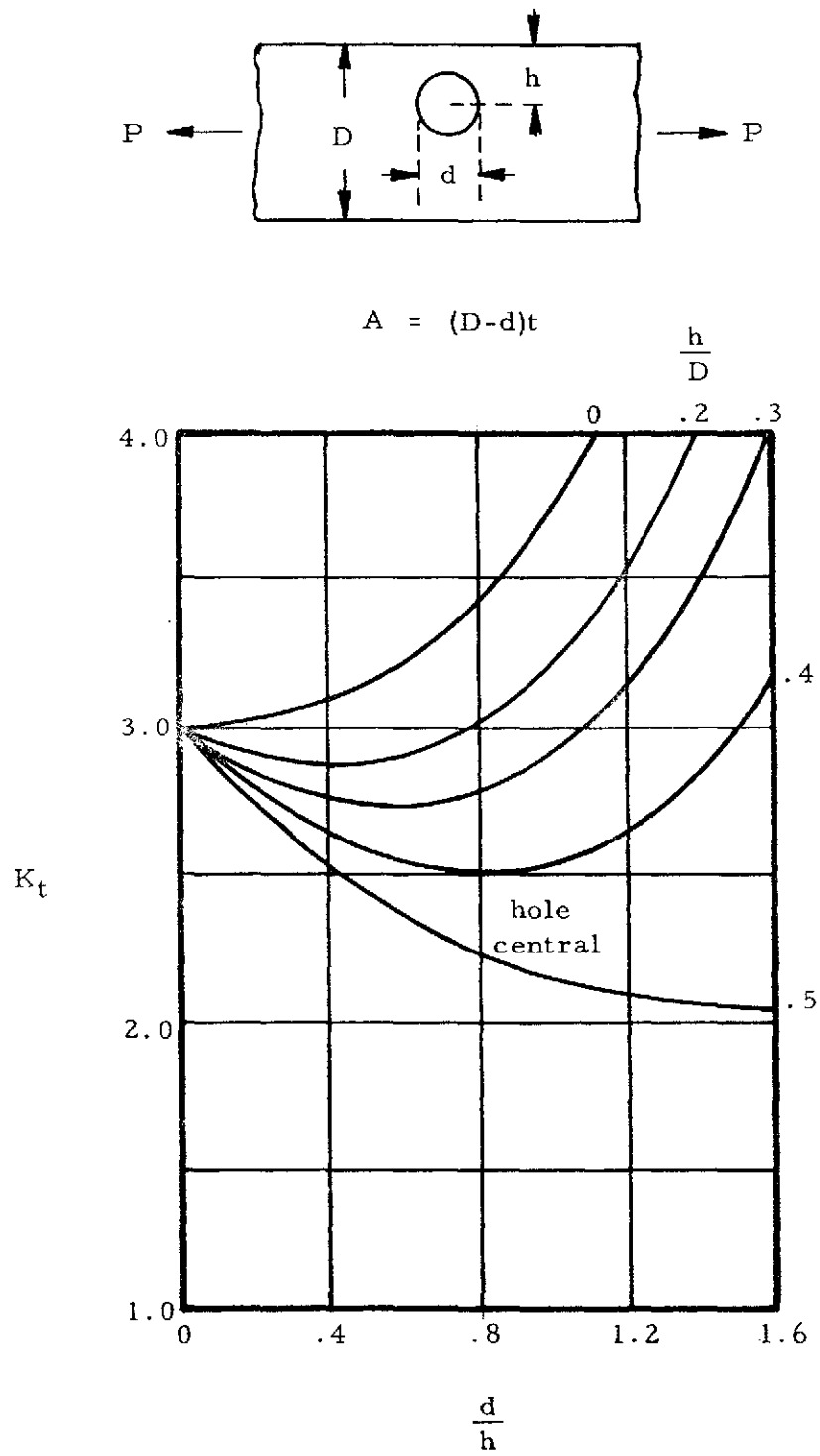
Figure 3.4 Rectangular Bar with Offset Through Hole
