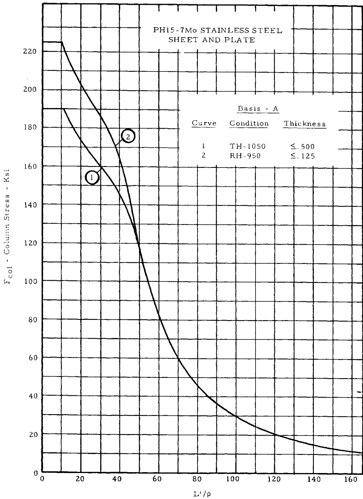
Figure 2-23. Column Allowable Curves
