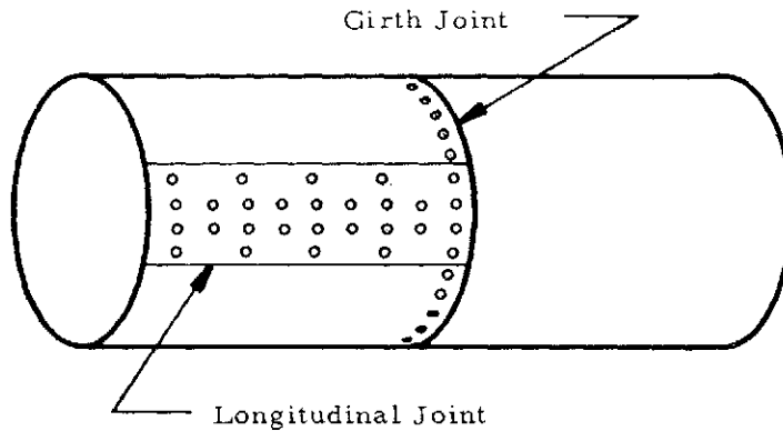
Figure 8-3. Joints on a Cylindrical Pressure Vessel
