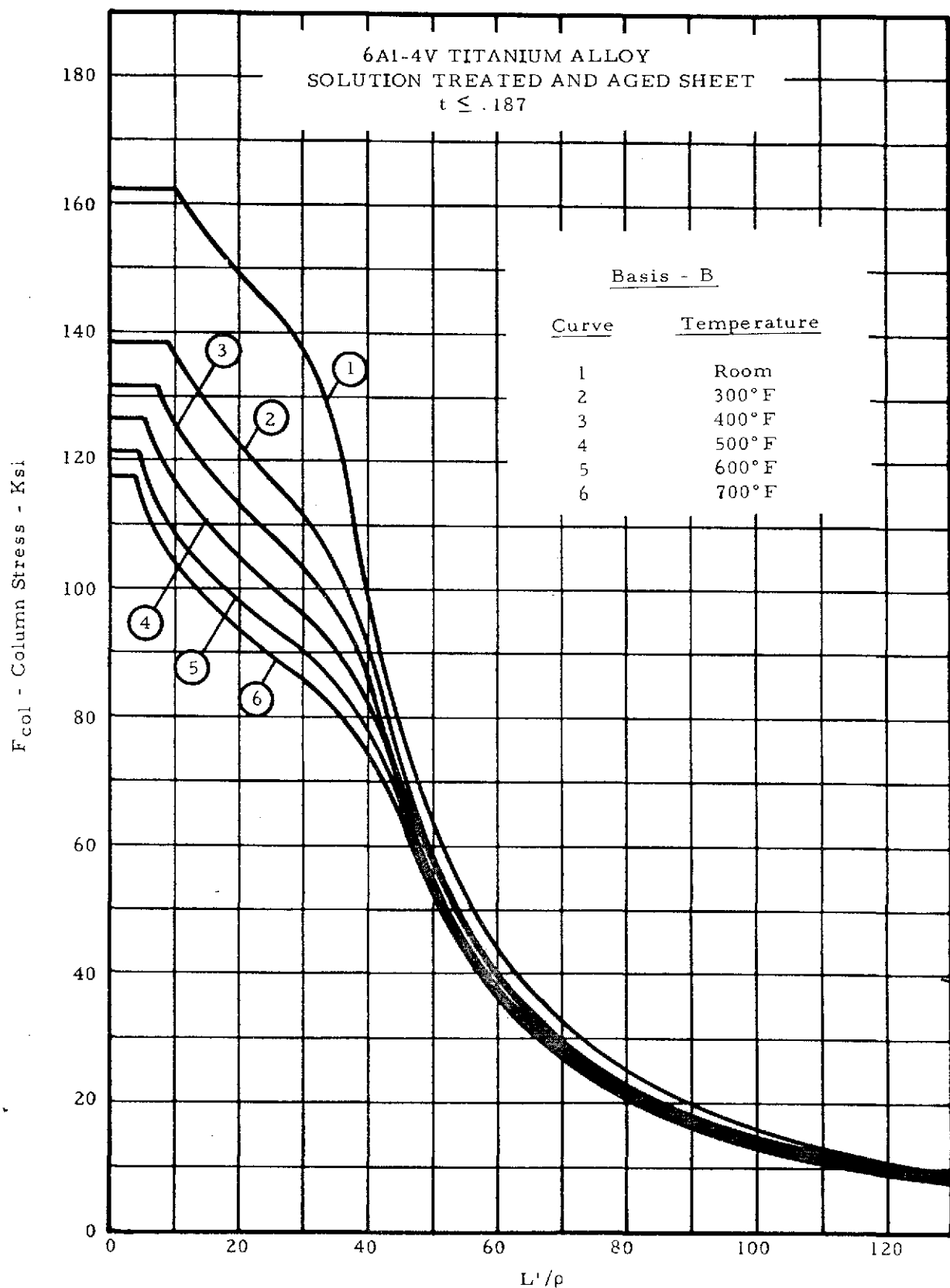
Figure 2-30. Column Allowable Curves
