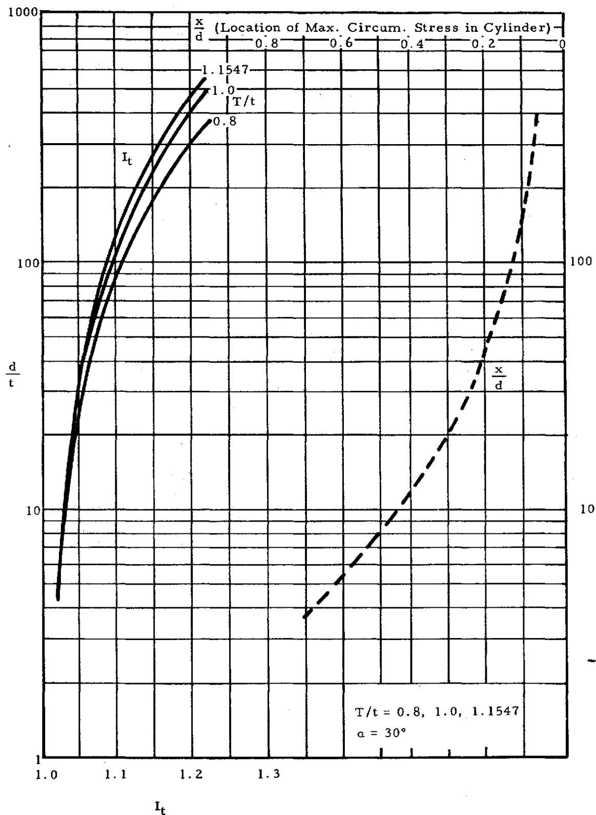
Figure 8-20. Stress Ratios for Pressure Vessels with Conical Head Closures *
