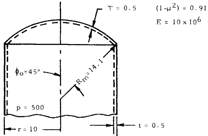
Figure 8-9. Cylindrical Pressure Vessel with Dished Head
