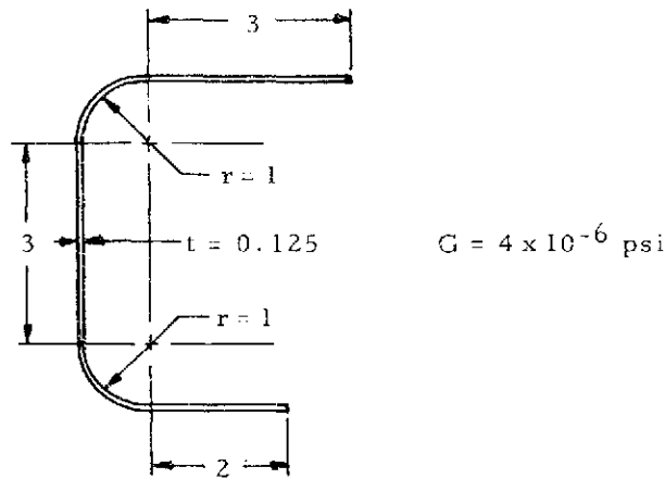
Figure 1-53. Thin Open Section
