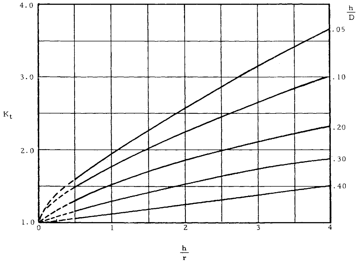
Figure 3-5. Stepped Rectangular Bar with Radial Fillet
