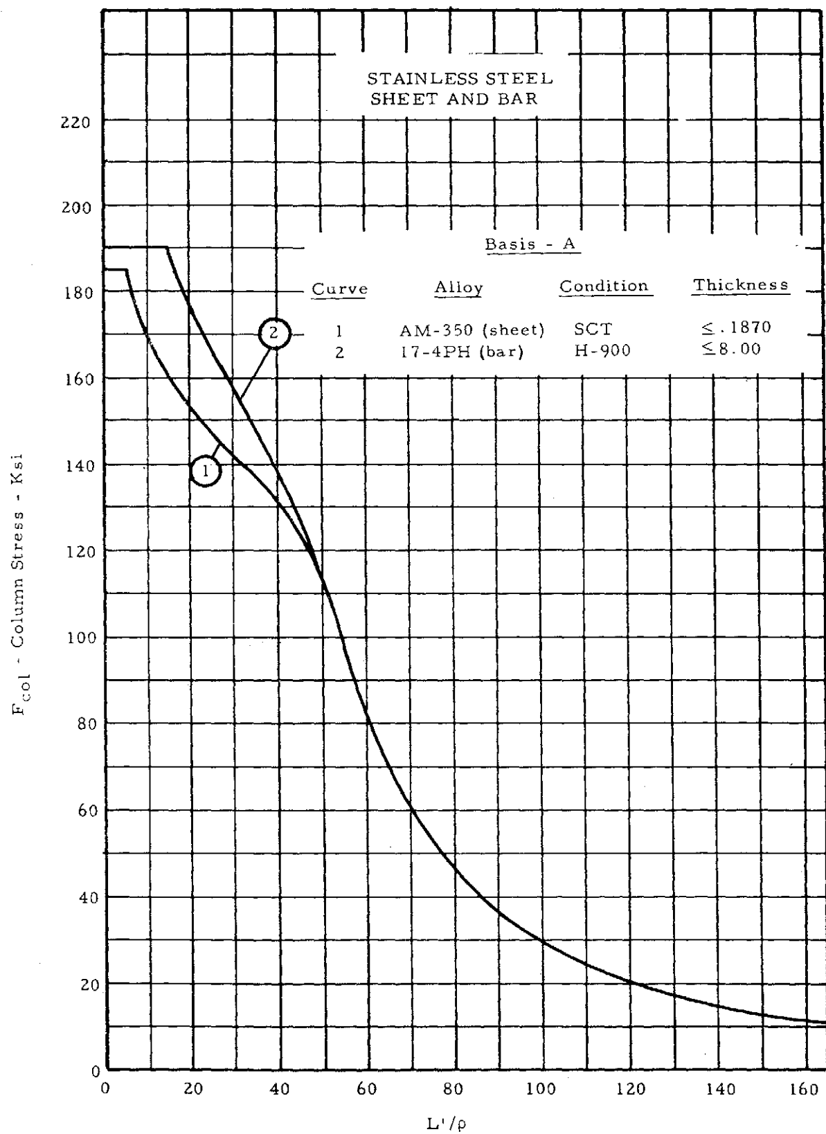
Figure 2-21. Column Allowable Curves
