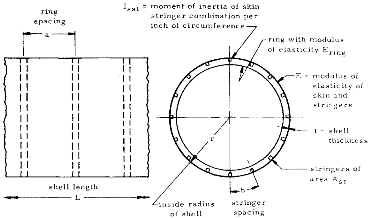
Figure 8-39. Shell with Rings and Stringers
