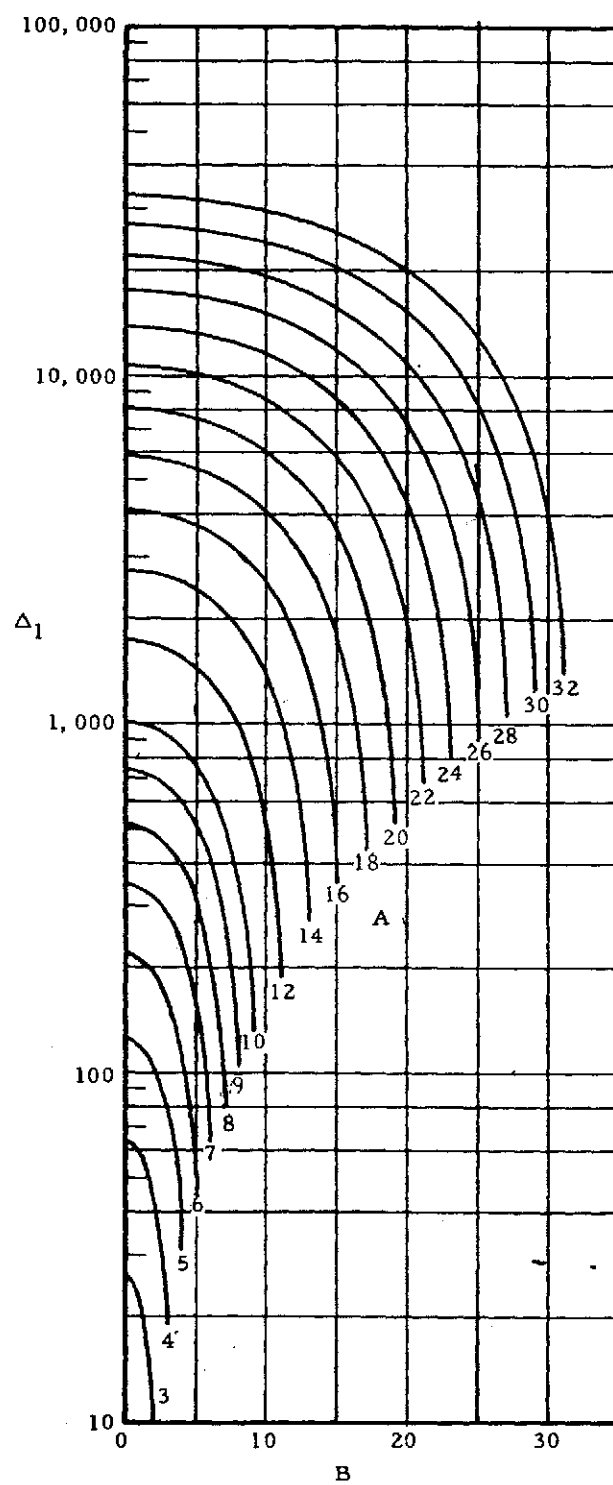
Figure 8-45. \Delta_1 as a Function of A and B
