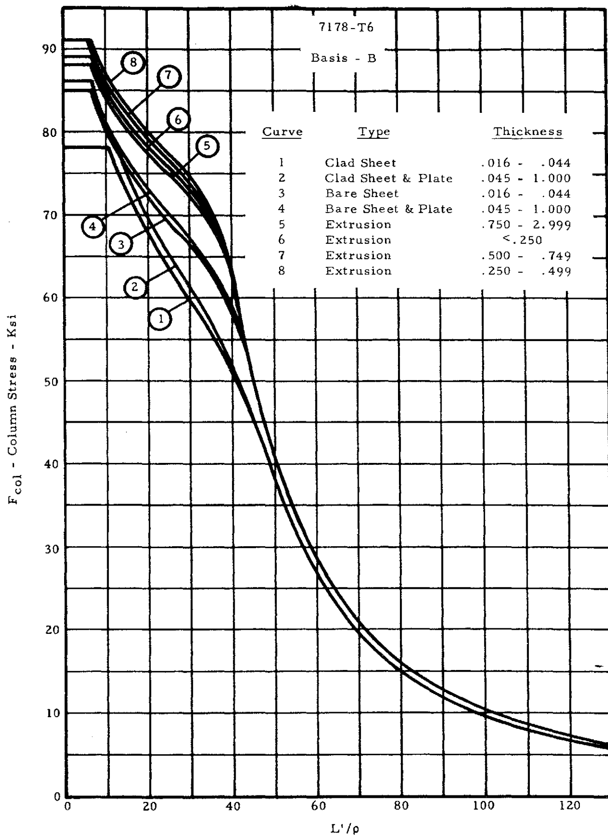
Figure 2-10. Column Allowable Curves
