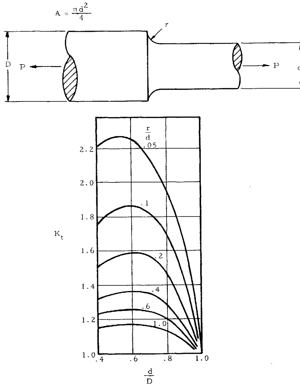
Figure 3-1. Stepped Round Bar with Radial Fillet
