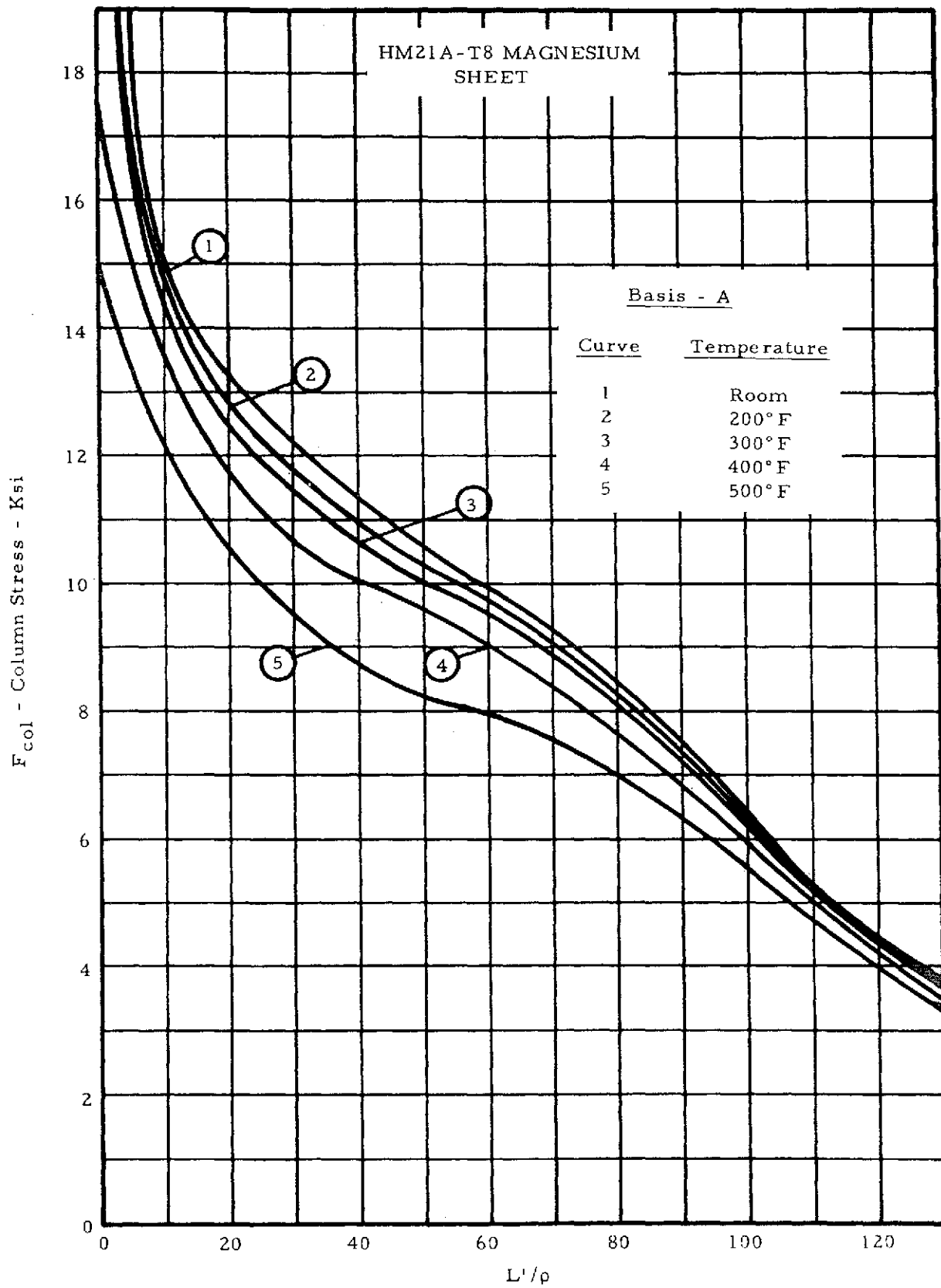
Figure 2-14. Column Allowable Curves
