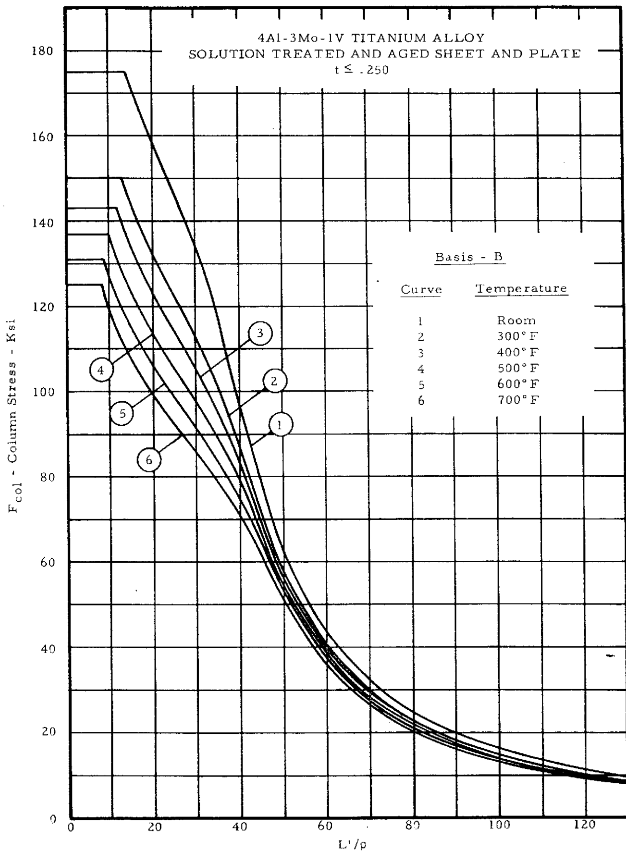
Figure 2-26. Column Allowable Curves
