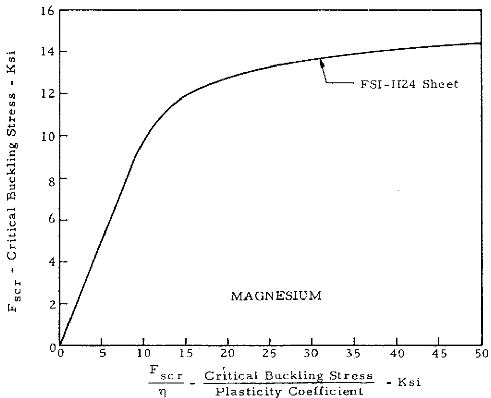
Figure 1-14. F_{scr} versus F_{scr}/\eta for Aluminum and Magnesium
