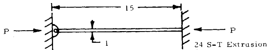
Figure 2-49. Column Loading Used for Illustration of Tangent-Modulus Equation
