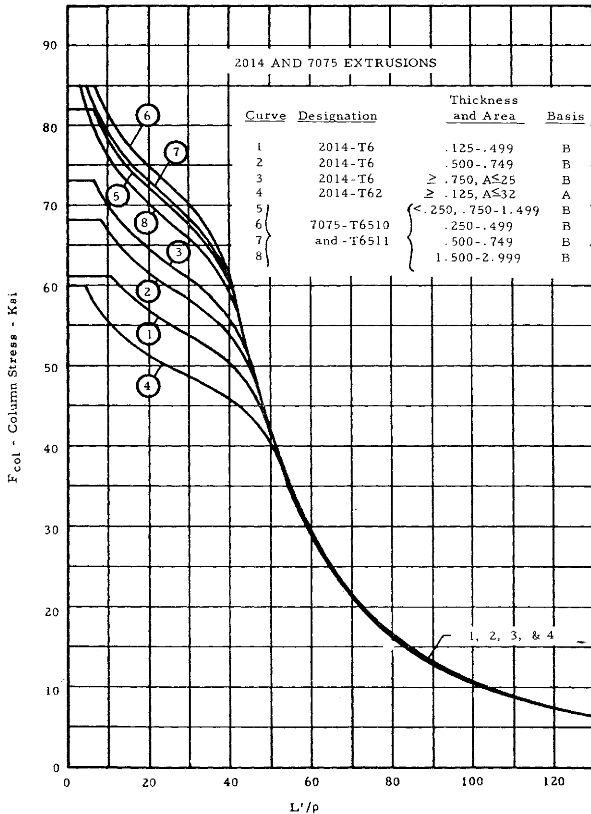
Figure 2-3. Column Allowable Curves
