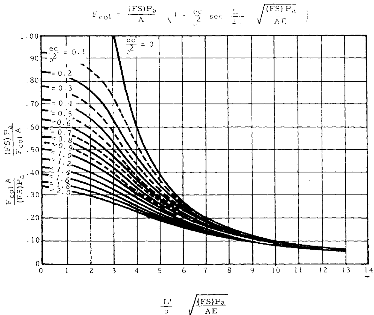
Figure 2-53. Graphical Presentation of the Secant Column Formula
