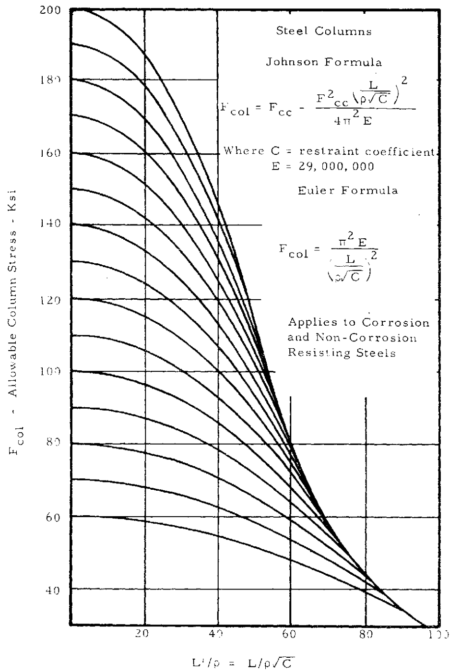
Figure 2-65a. Johnson-Euler Column Curve
