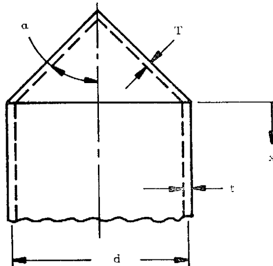
Figure 8-14. Cylindrical Pressure Vessel with Conical Head
