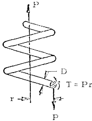
Figure 1-69. Helical Spring of Round Wire
