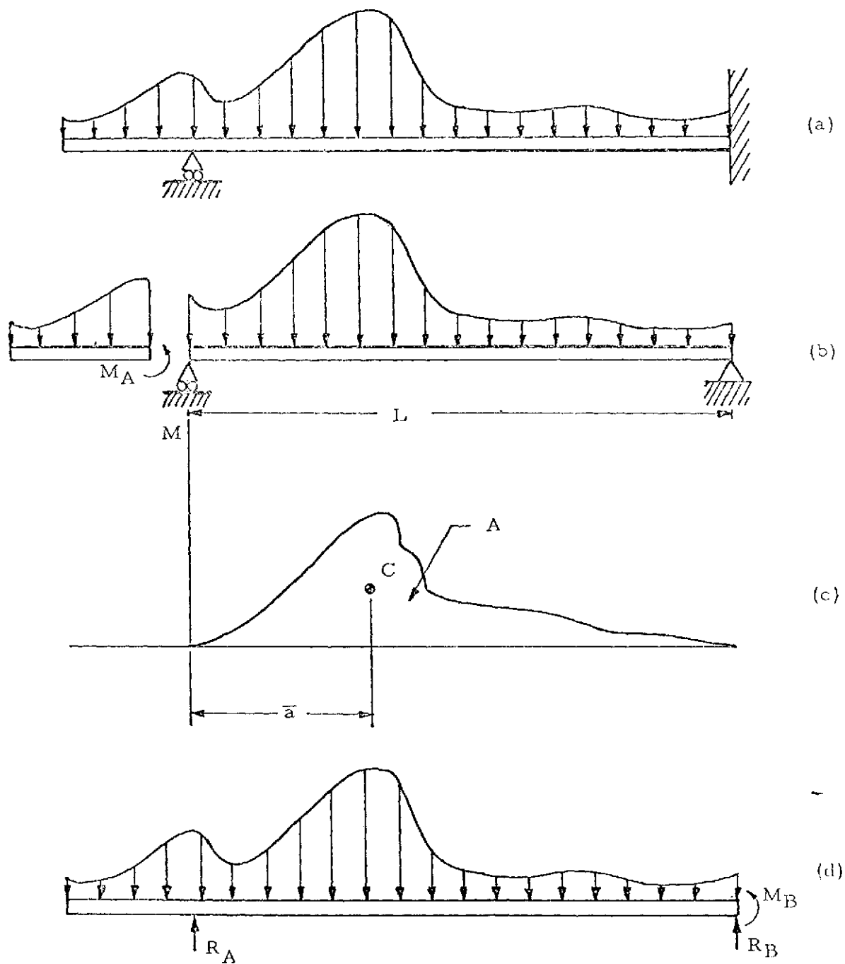
Figure 1-31. Method of Determining Reaction Forces and Moments on a Beam Fixed at One End and Pinned at One Point
