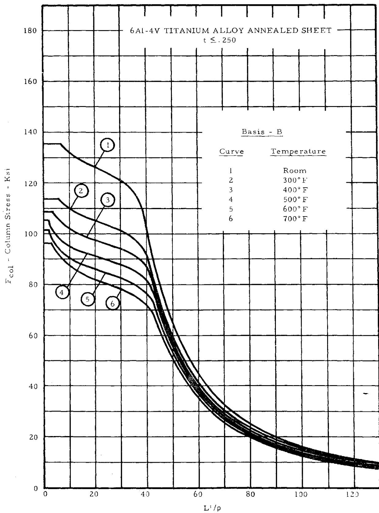
Figure 2-29. Column Allowable Curves
