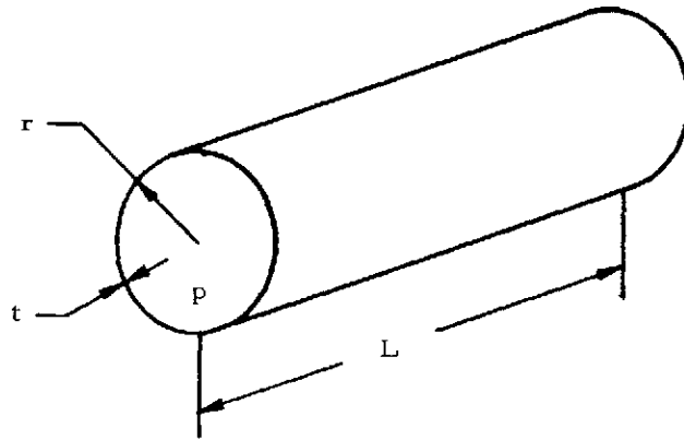
Figure 8-28. Pressurized Cylinder
