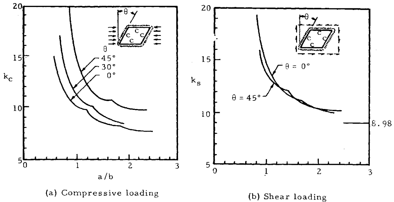
Figure 6-40. Buckling Coefficient of Clamped Oblique Flat Plates
