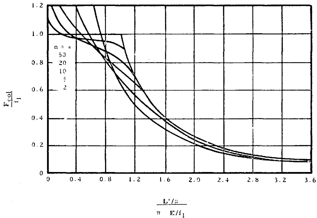
Figure 2-48. Nondimensional Plot of Tangent Modulus Equation with E_t Obtained from the Ramberg-Osgood Equation
