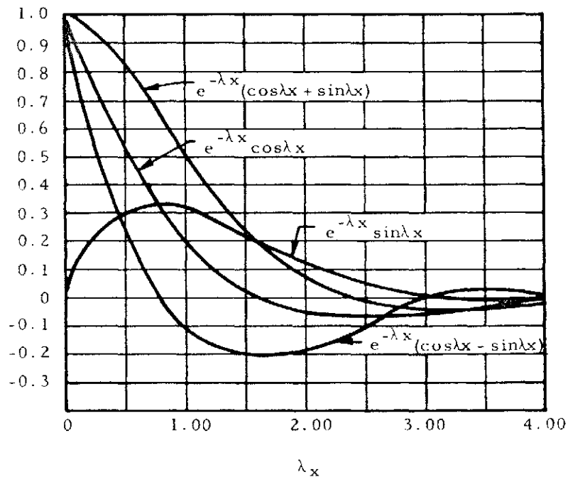
Figure 8-8. Curves for the Evaluation of the Equations in Table 8-4 *
