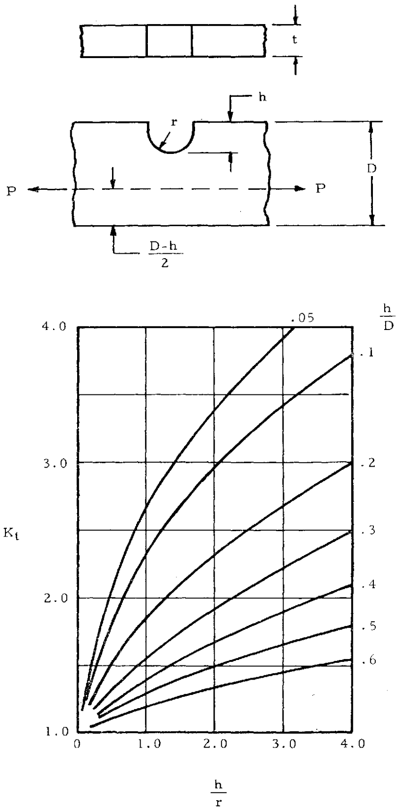
Figure 3-6. Rectangular Bar with U Notch (One Side)
