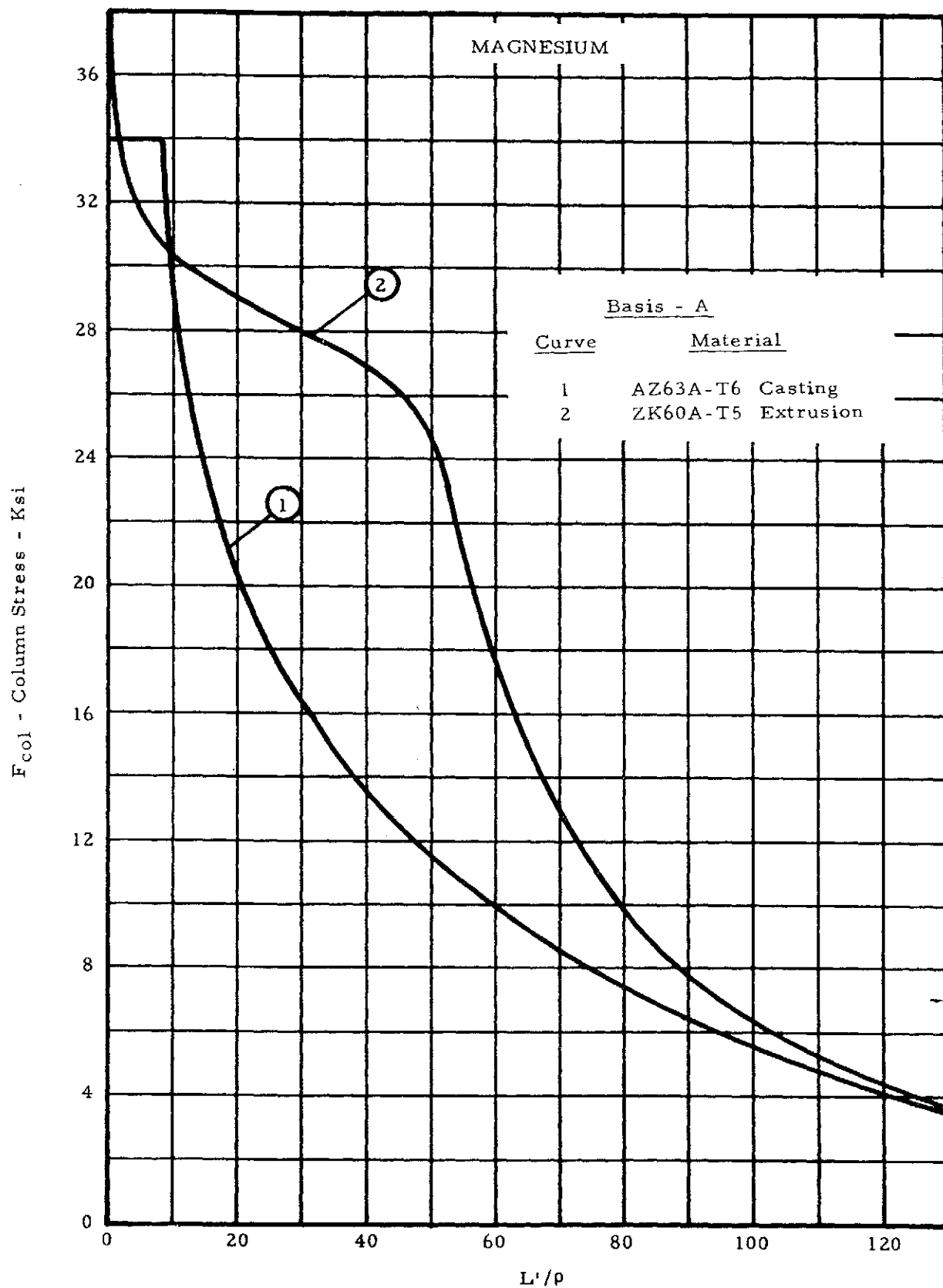
Figure 2-12. Column Allowable Curves
