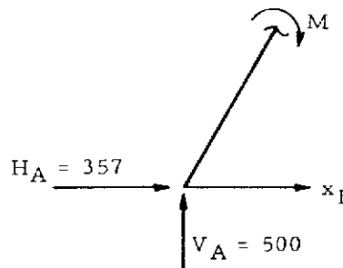
Figure 5-15. Section of Frame Leg
