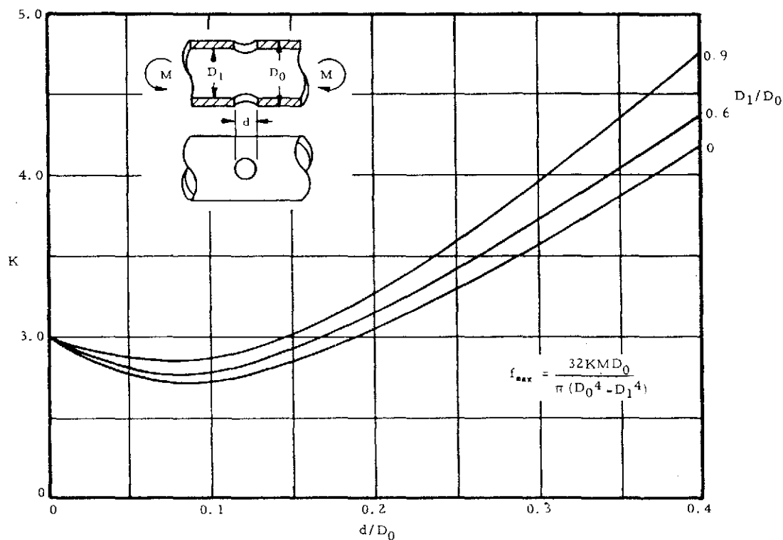
Figure 10-5. Stress Concentration Factor for Hollow Shaft with Radial Hole (concluded)
