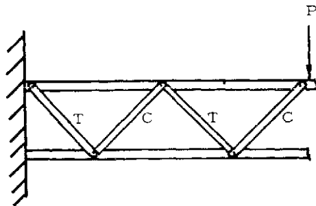
Figure 3-17. Example of Lacing Bars
