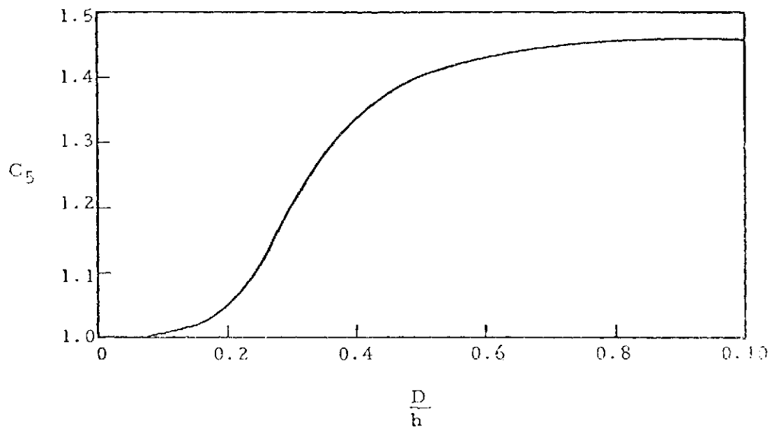
Figure 1-29. Design Reduction Factors Due to Access Hole
