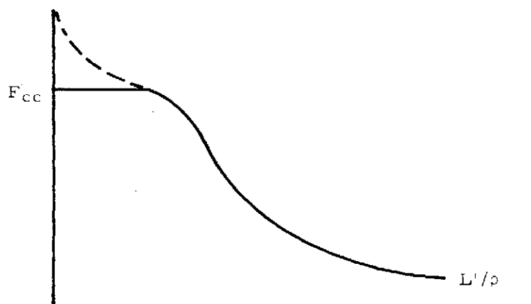
Figure 2-63. Failure Curve Based on the Assumption of No Interaction Between Primary Failure and Crippling .
