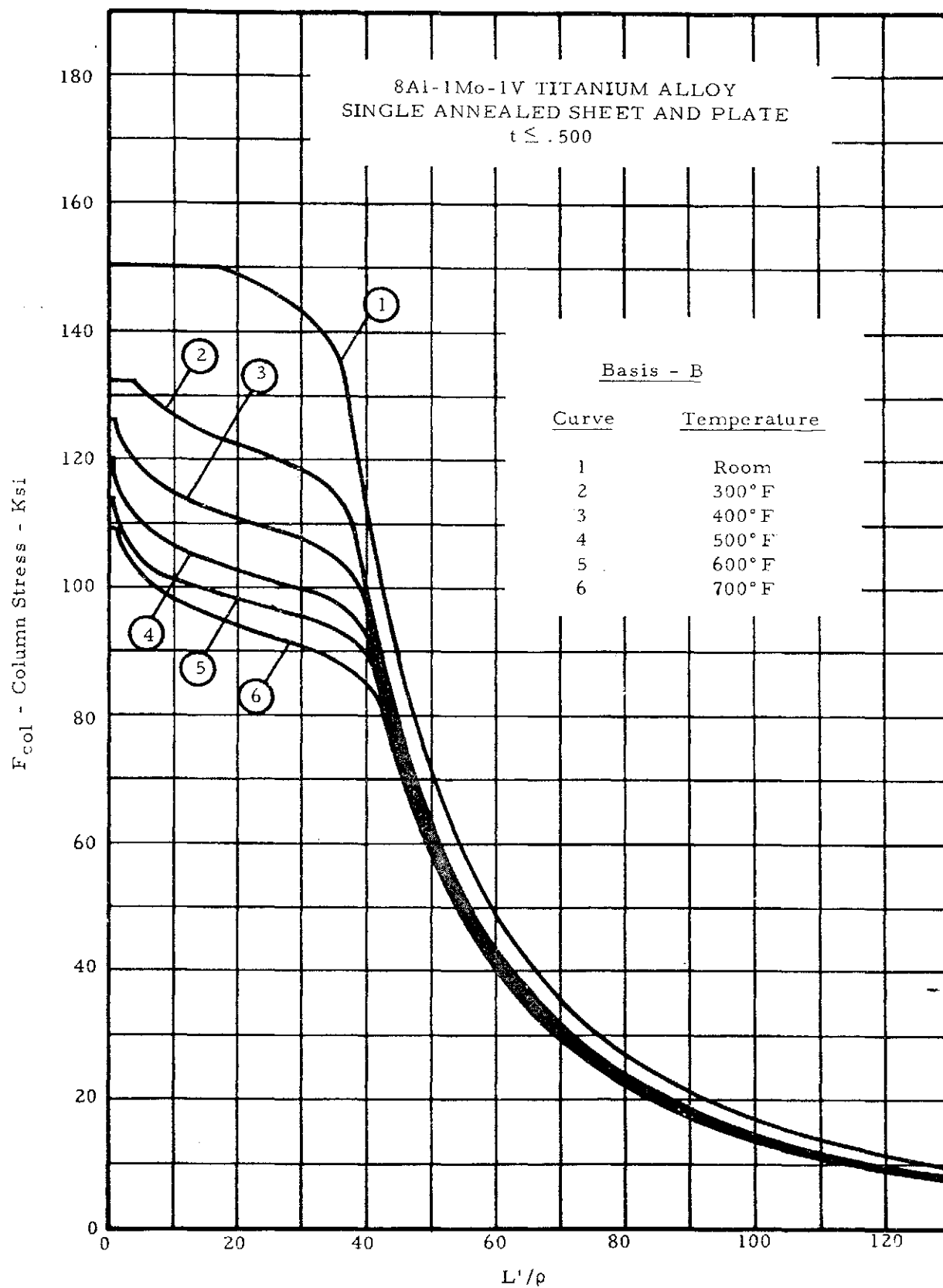
Figure 2-32. Column Allowable Curves
