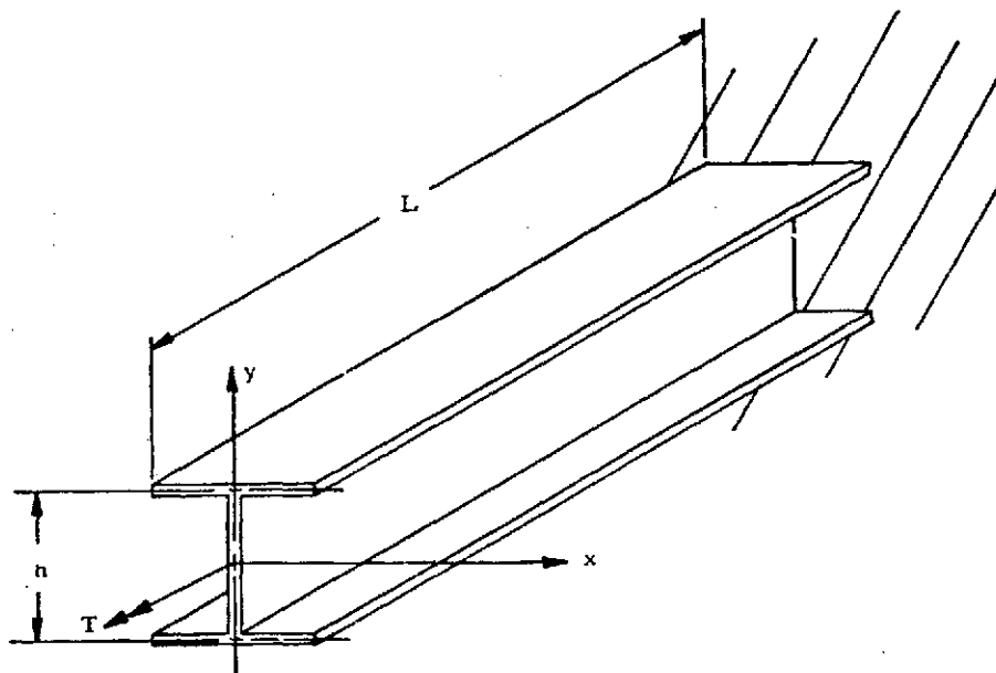
Figure 1-65. I-Beam Restrained at One End
