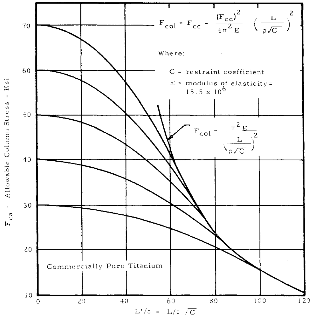
Figure 2-65b. Johnson-Euler Column Curve
