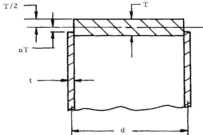
Figure 8-10. Junction of Cylinder and Flat Head
