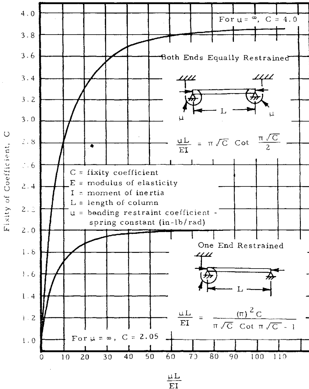
Figure 2-38. Fixity Coefficient for a Column with End Supports Having a Known Bending Restraint
