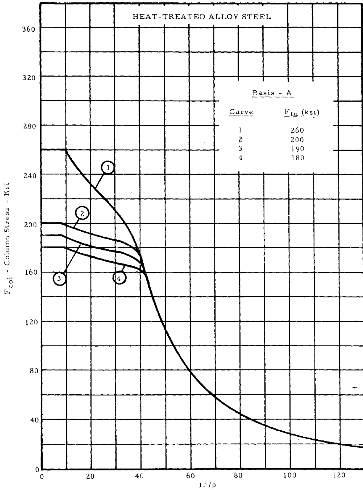
Figure 2-17. Column Allowable Curves
