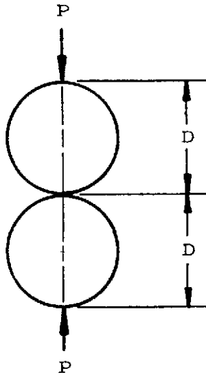
Figure 11-5. Similar Spheres in Contact
