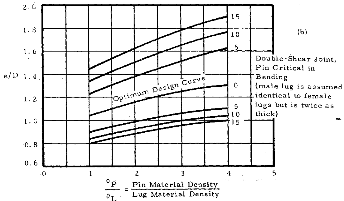
Figure 9-15. Edge Distance Ratio
