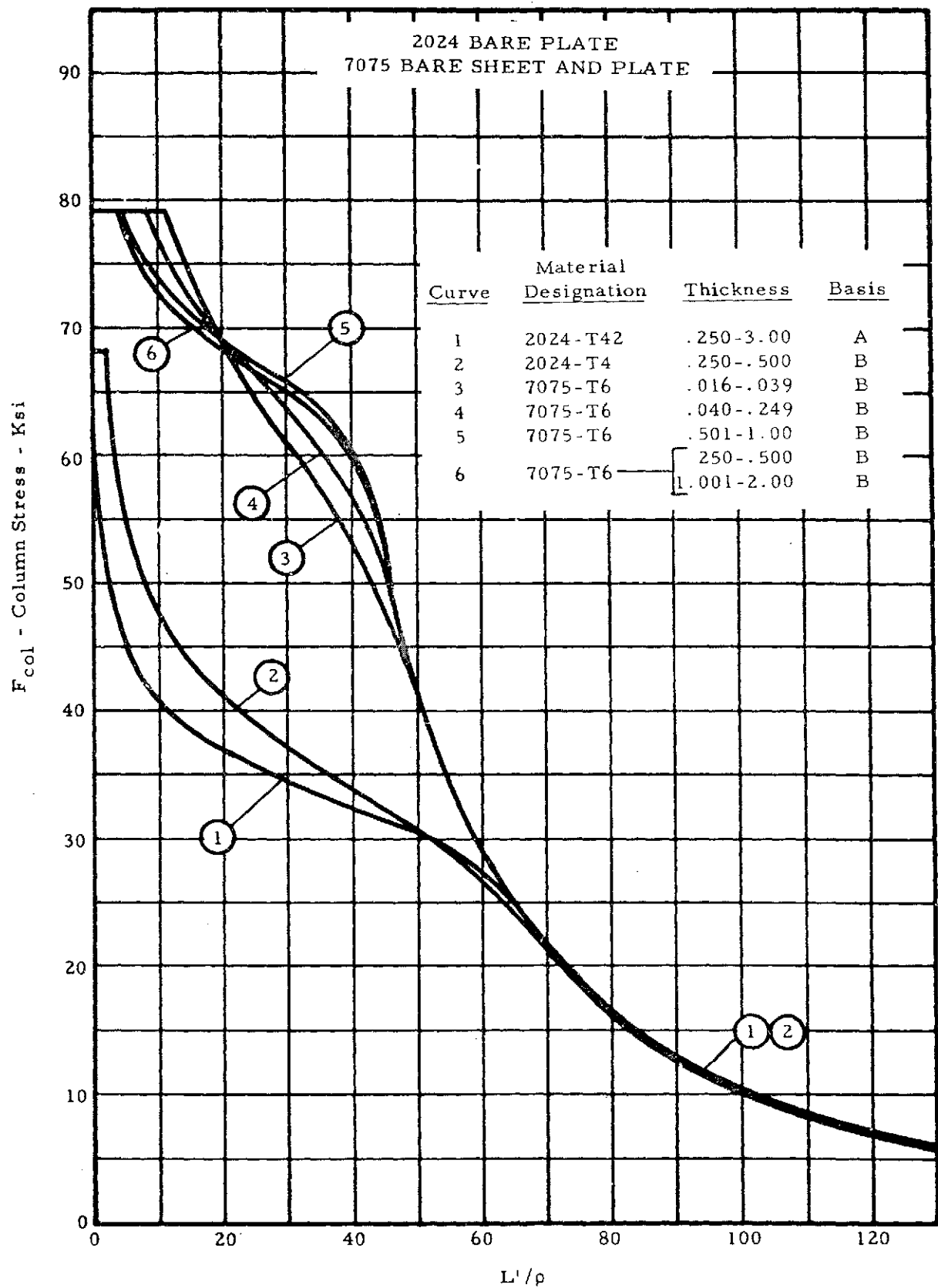
Figure 2-5. Column Allowable Curves
