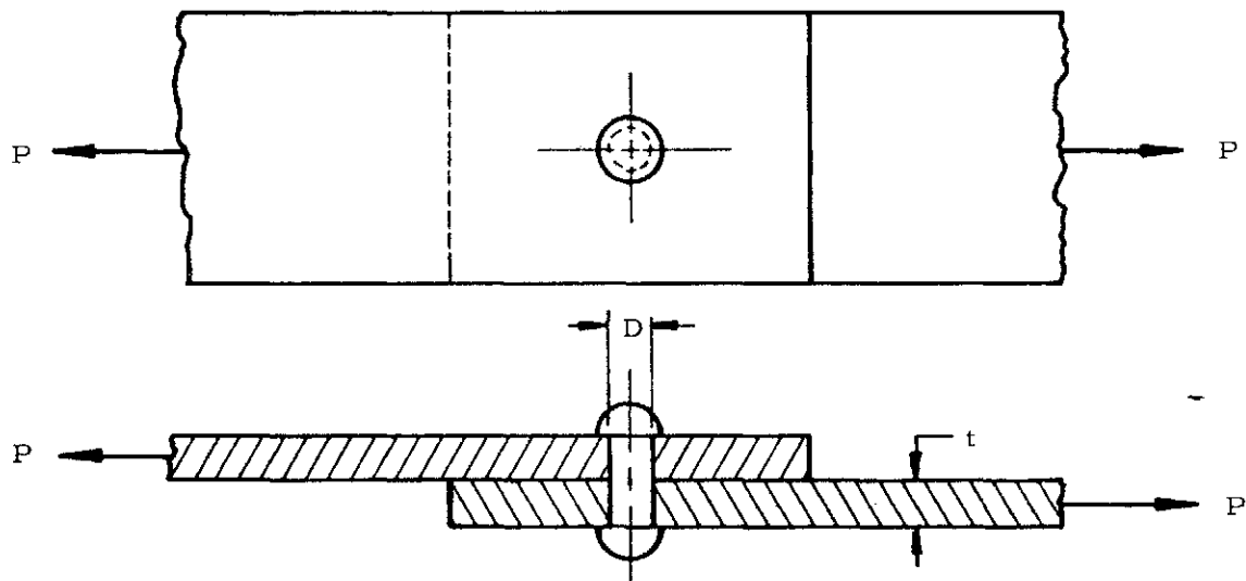
Figure 11-1. Riveted Connection
