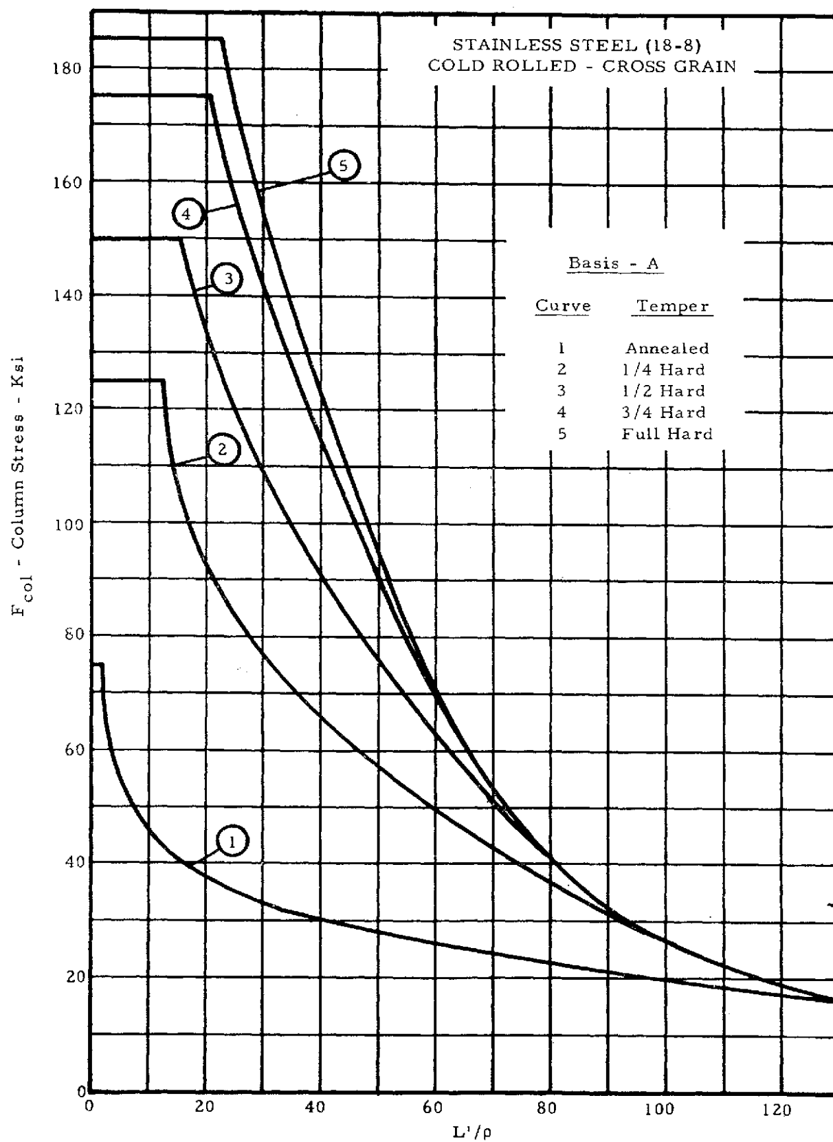
Figure 2-20. Column Allowable Curves
