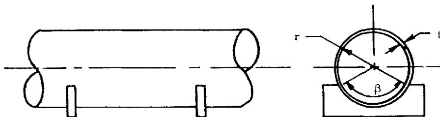
Figure 8-27. Cylindrical Pressure Vessel on Saddle Supports
