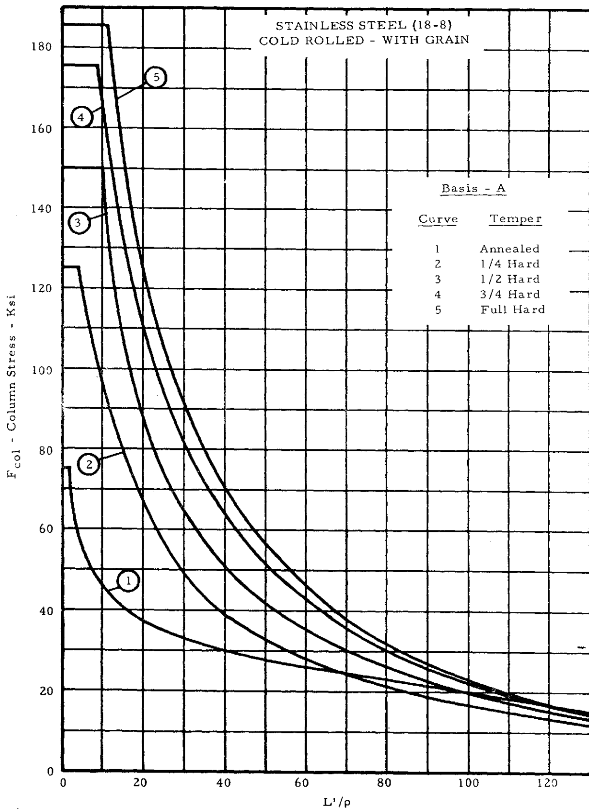
Figure 2-19. Column Allowable Curves
