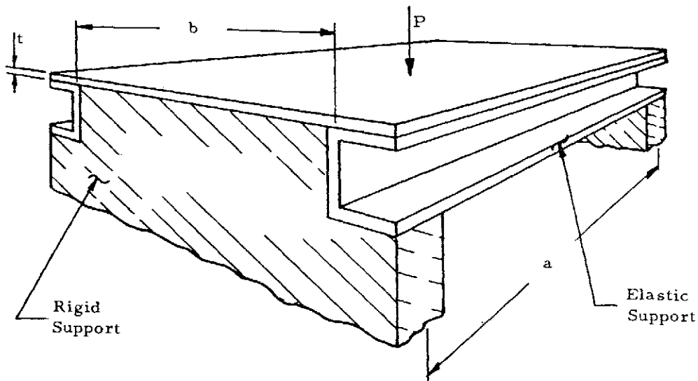
Figure 6-23. Beam-Supported Plate
