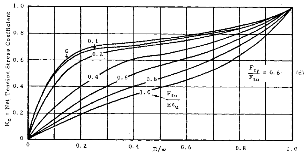
Figure 9-4. Net Tension Stress Coefficient (concluded)
