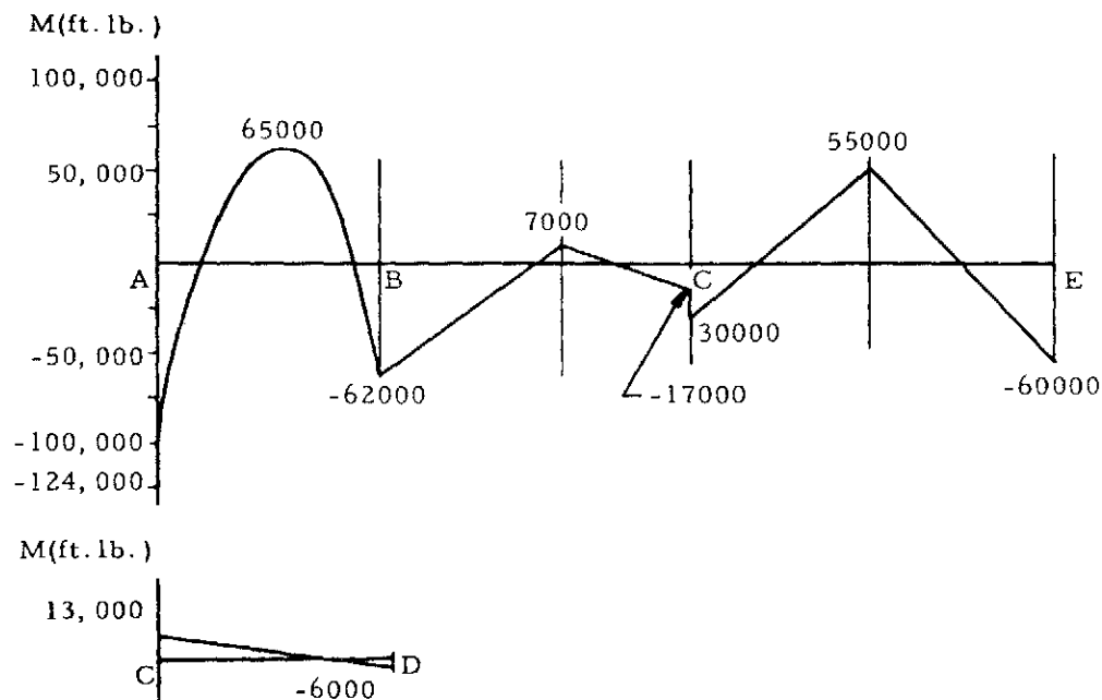
Figure 5-5. Moment Diagram for Frame Shown in Figure 5-4
