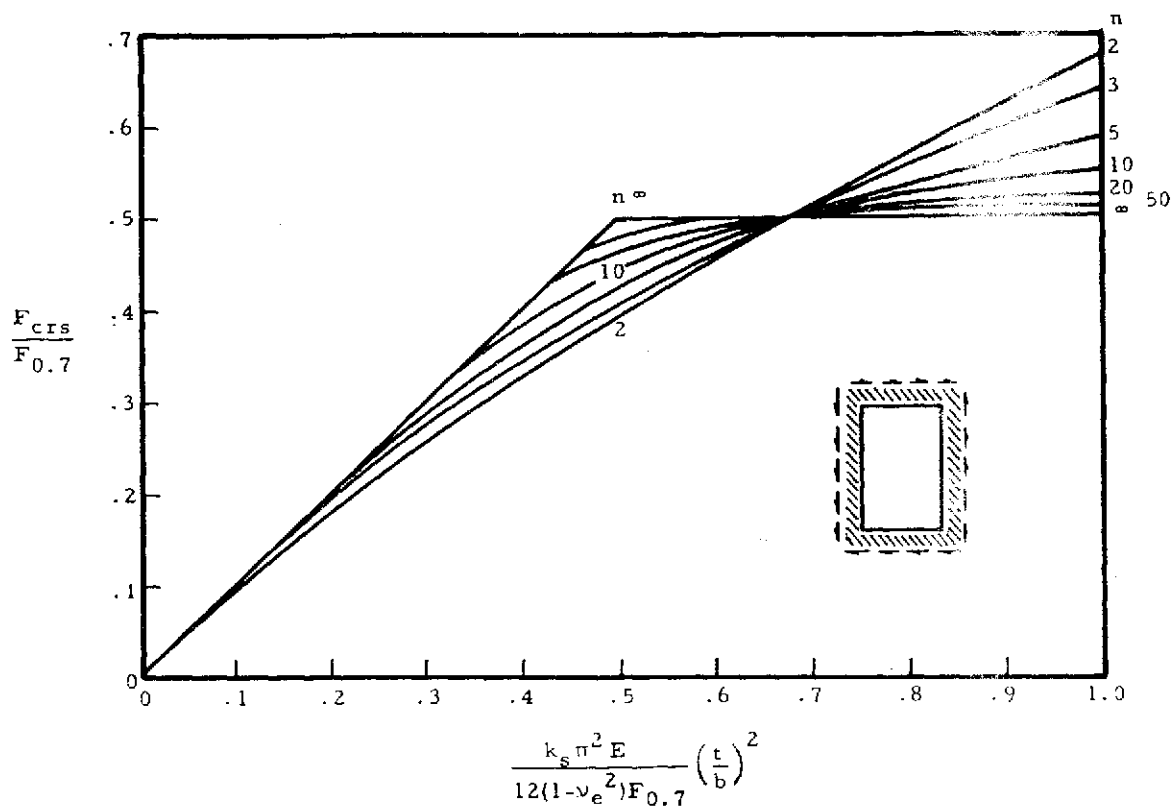
Figure 6-30. Chart of Nondimensional Shear Buckling Stress for Panels with Edge Rotational Restraint
