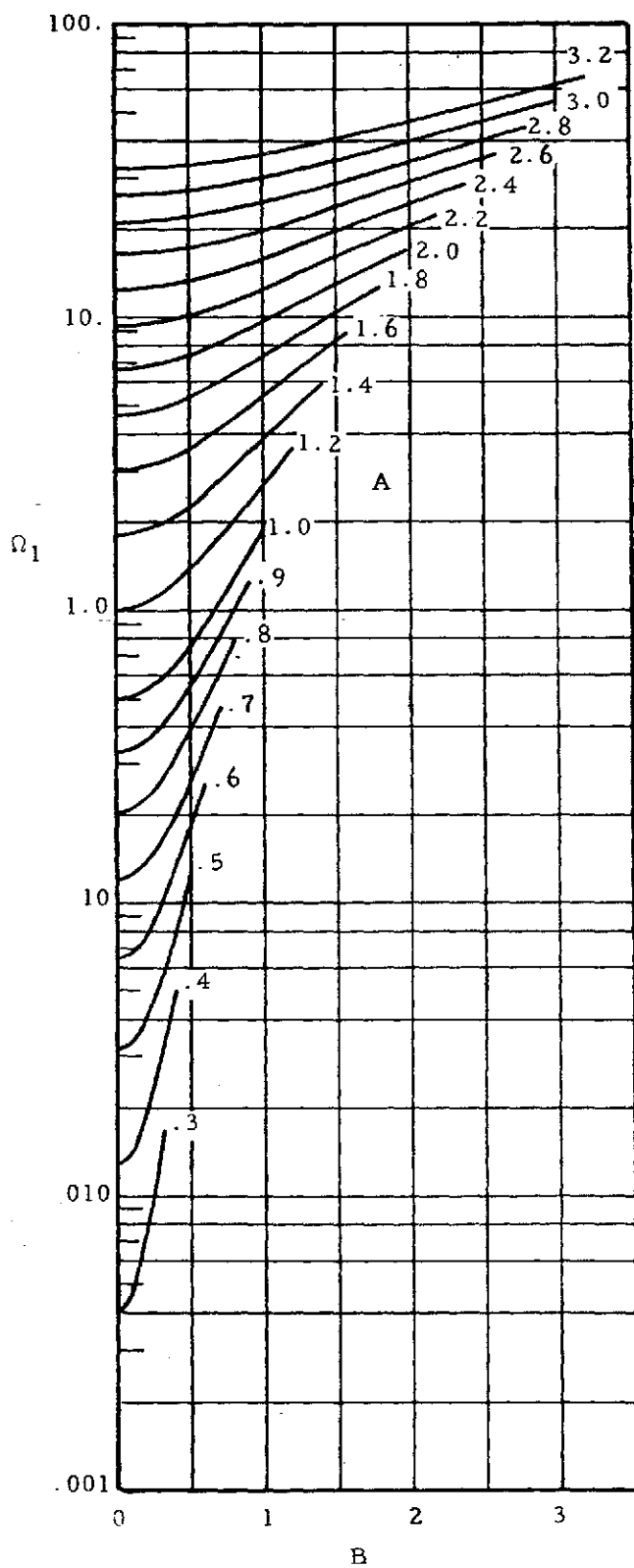
Figure 8-41. \Omega_1 as a Function of A and B
