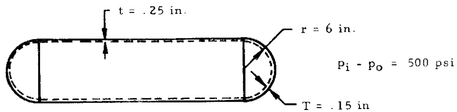
Figure 8-5. Thin Cylindrical Pressure Vessel with Hemispherical Heads
