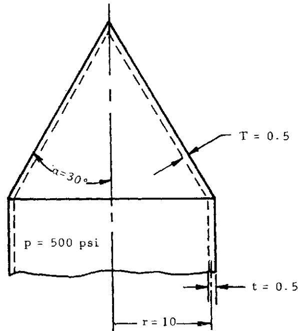
Figure 8-23. Thin Cylindrical Pressure Vessel with Conical Head
