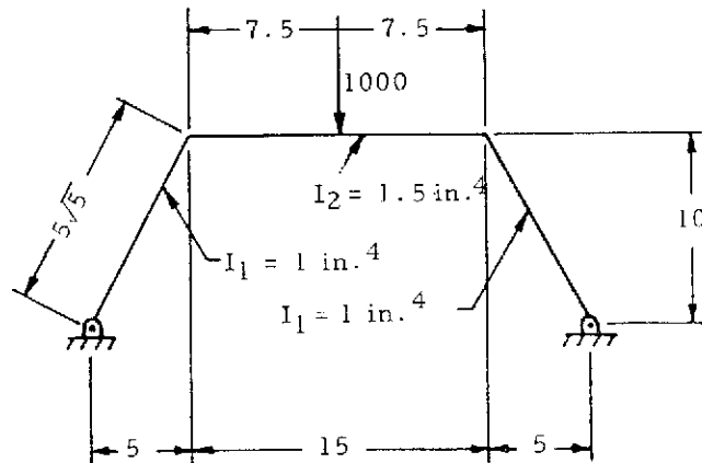
Figure 5-14. Trapezoidal Frame
