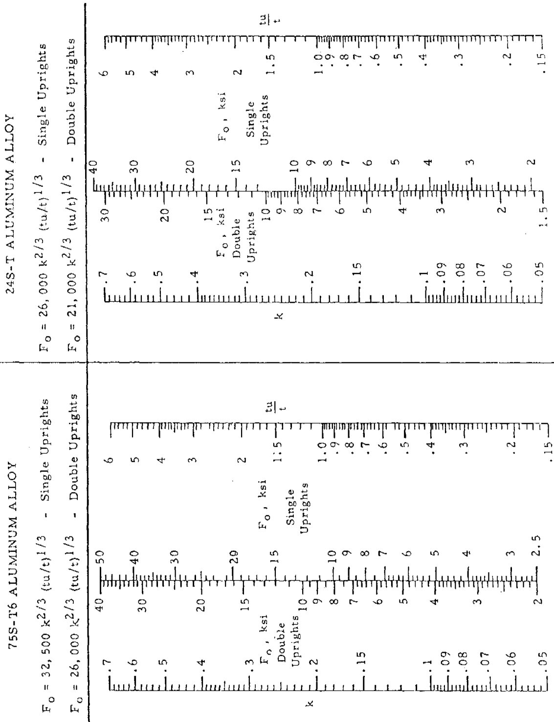
Figure 1-23. Nomograms for Upright Forced Crippling Allowable Stress
