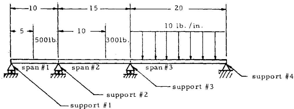
Figure 1-37. Continuous Beam on Four Supports
