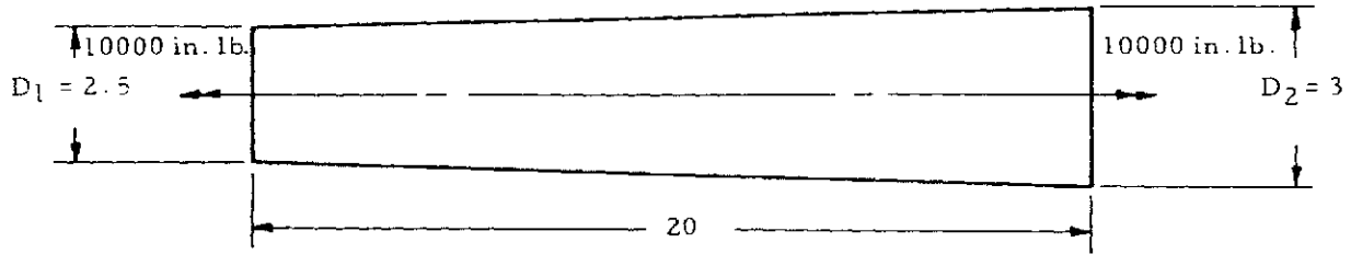
Figure 1-48. Tapered Circular Solid Beam in Torsion
