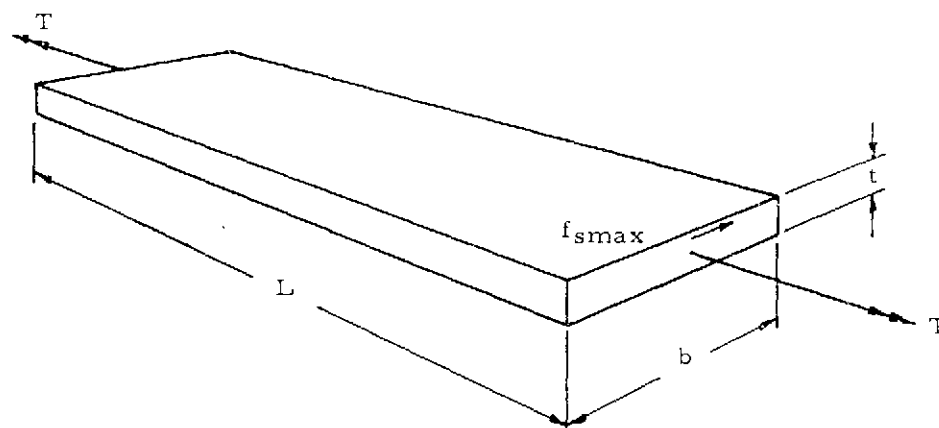
Figure 1-51. Rectangular Beam in Torsion
