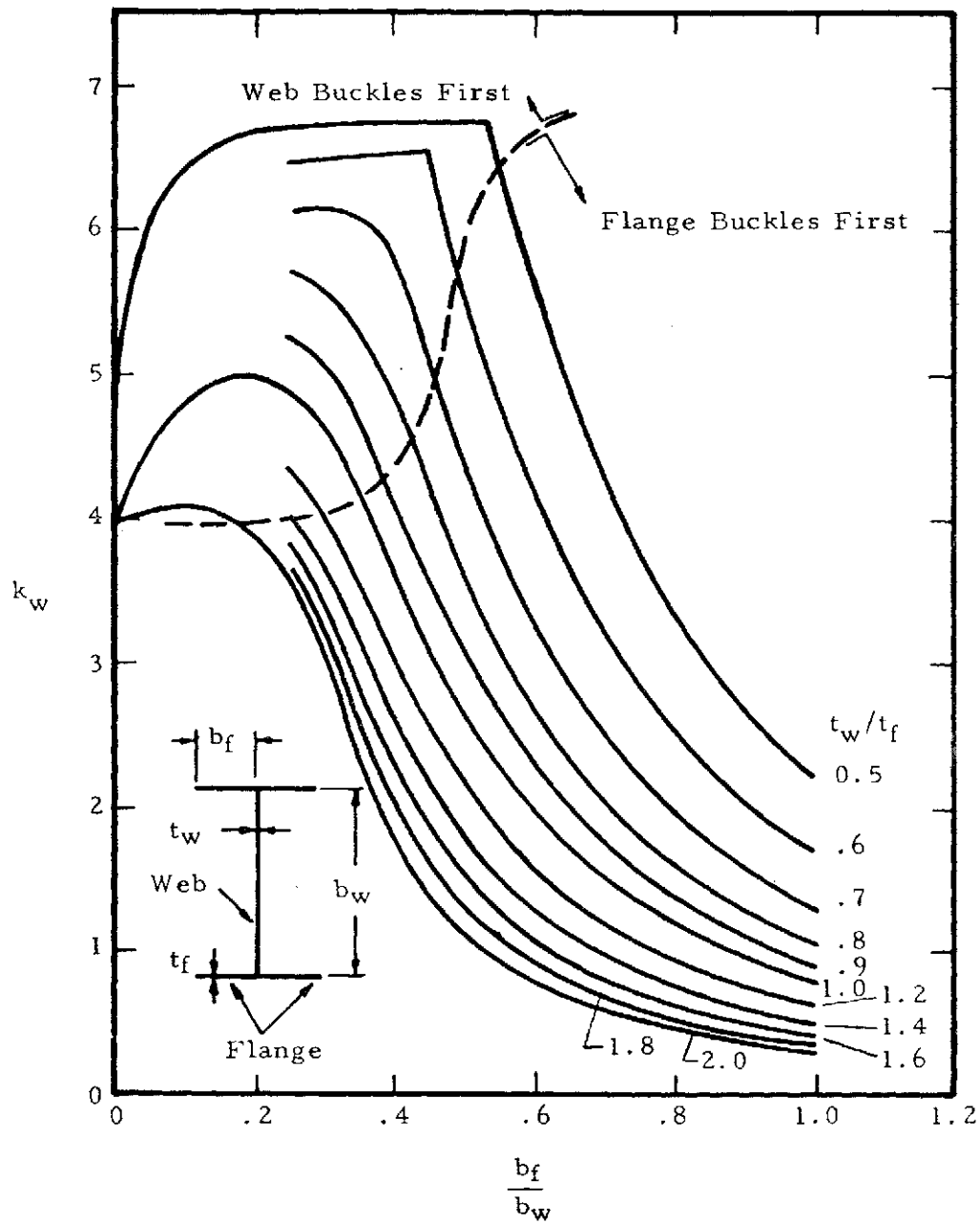
(b) H-section stiffeners
