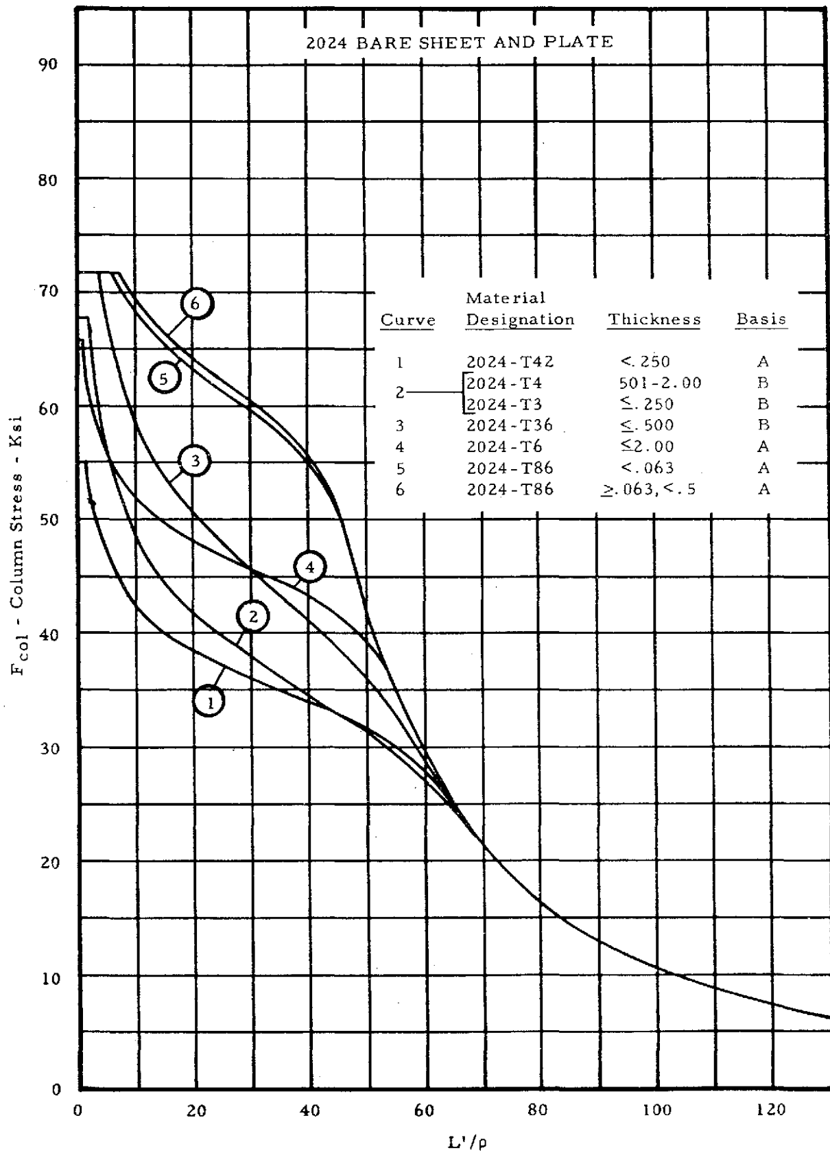
Figure 2-4. Column Allowable Curves
