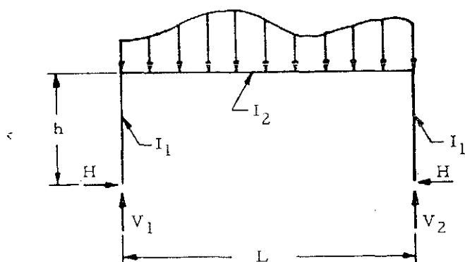
Figure 5-7. Free-Body Diagram of the Frame in Figure 5-6
