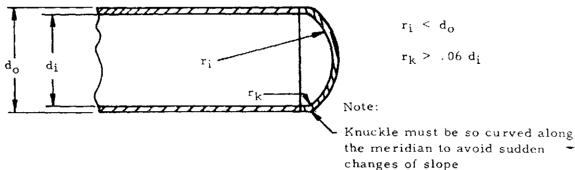
Figure 8-6. Proper Design of Dished Head
