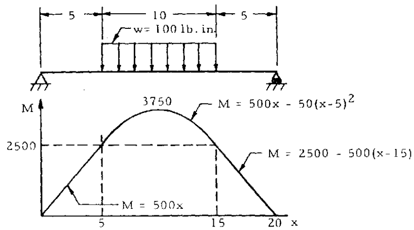
Figure 5-11. Determination of A_u
