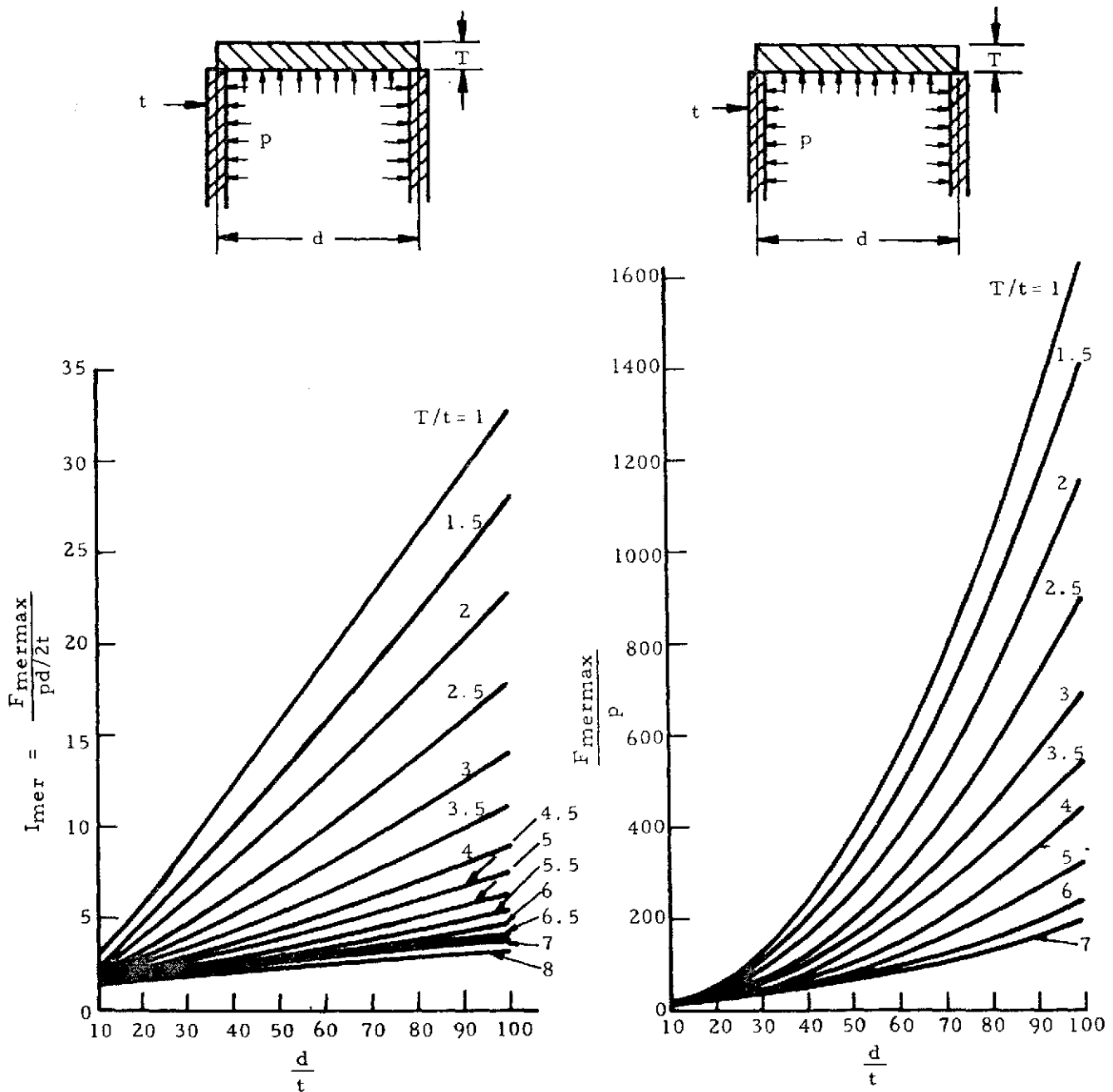
Figure 8-11. Graphical Presentation of Equation (8-11) for n = .5 *
