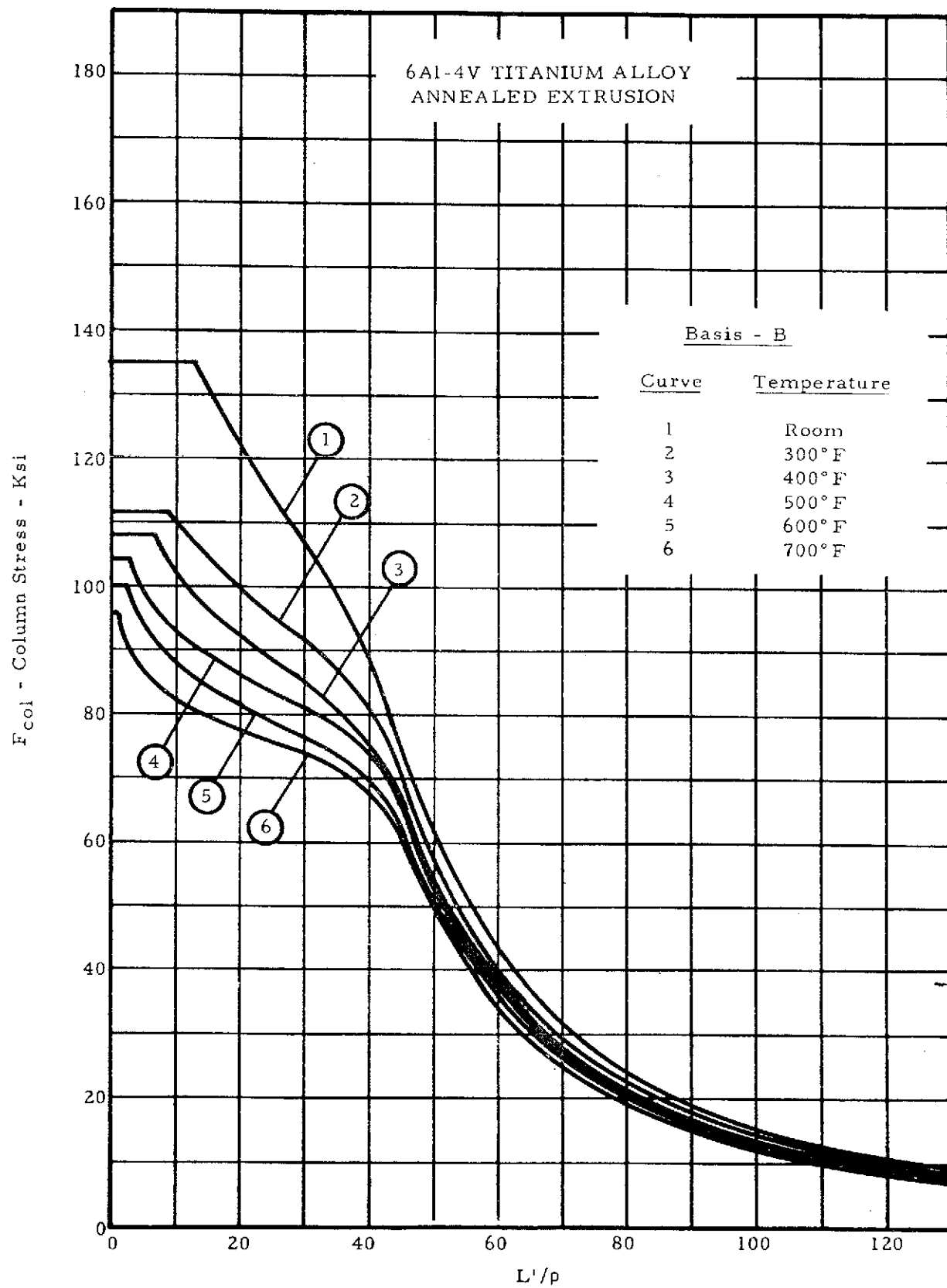
Figure 2-28. Column Allowable Curves
