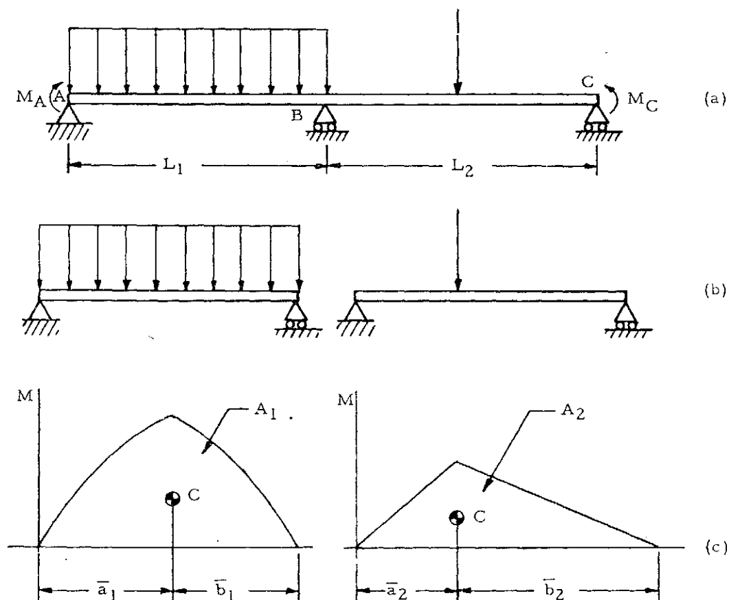
Figure 1-35. Beam Simply Supported at Three Points
