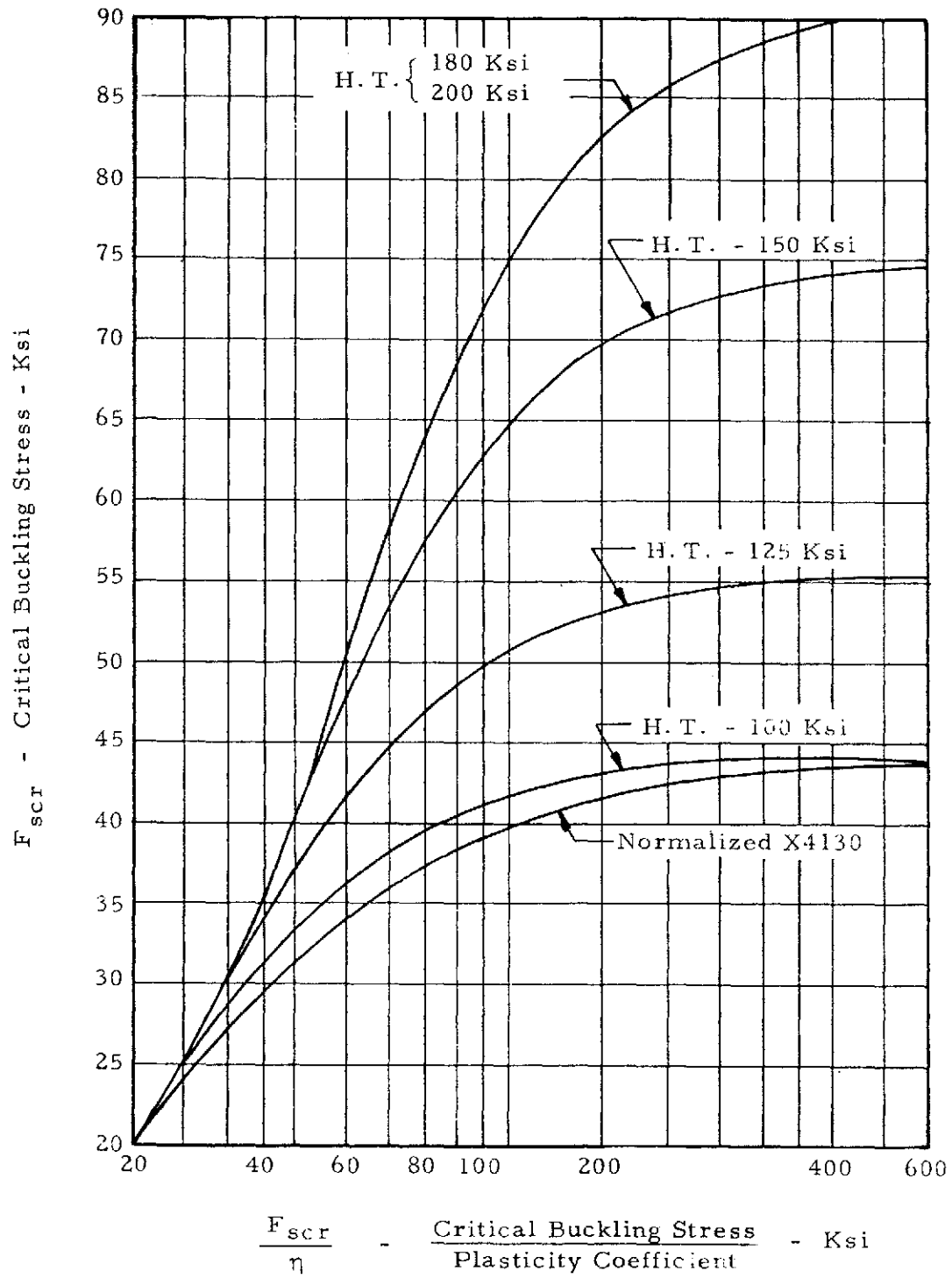
Figure 1-12. F_{scr} versus F_{scr}/\eta for Alloy Steel
