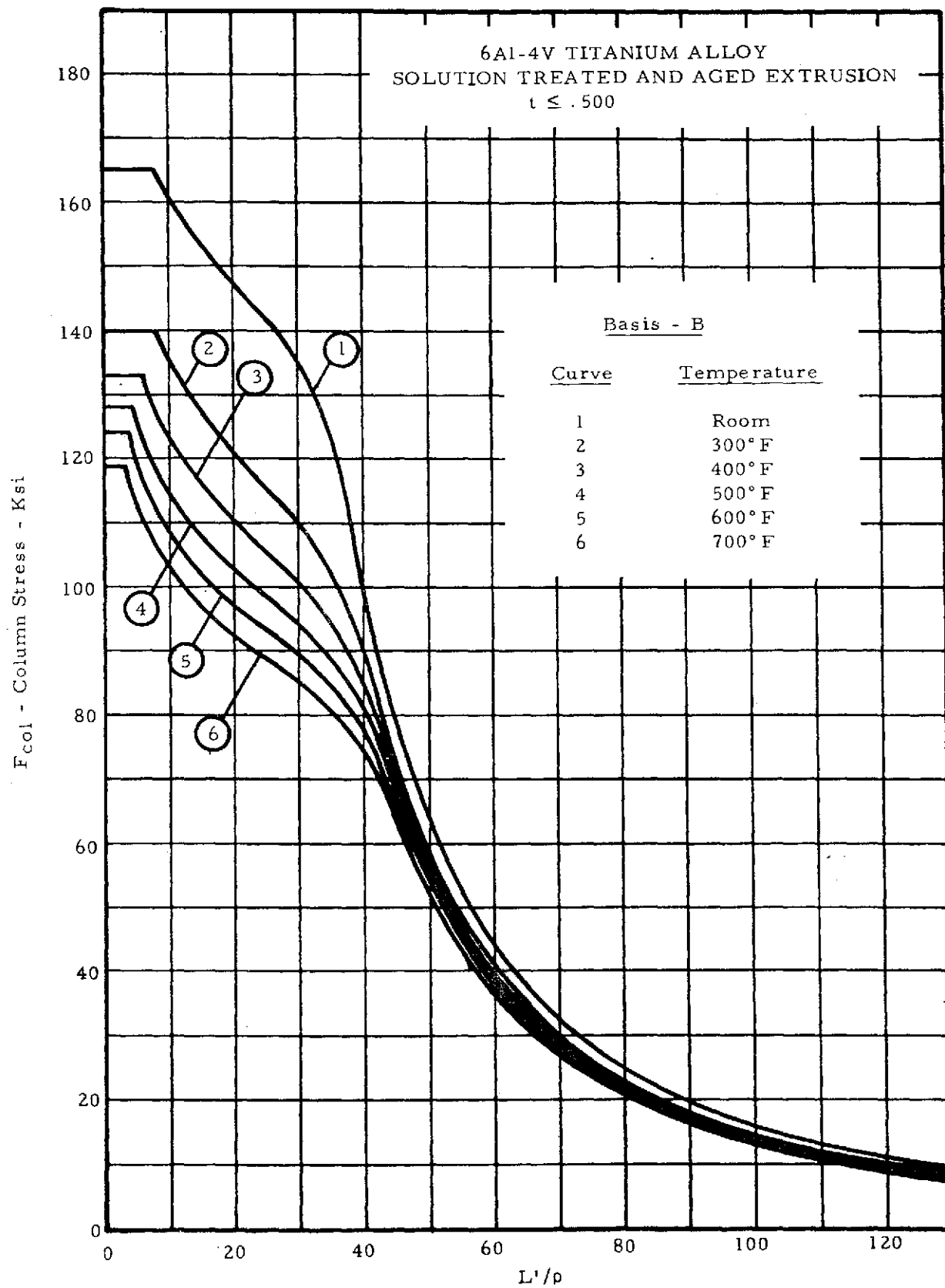
Figure 2-31. Column Allowable Curves
