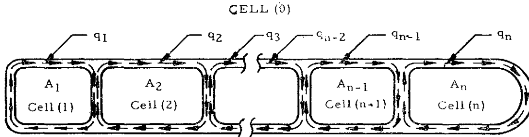
Figure 1-63. Multicell Tube in Torsion
