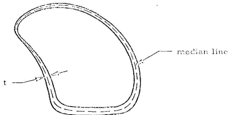
Figure 1-54. Cross Section of a Single Cell Closed Beam
