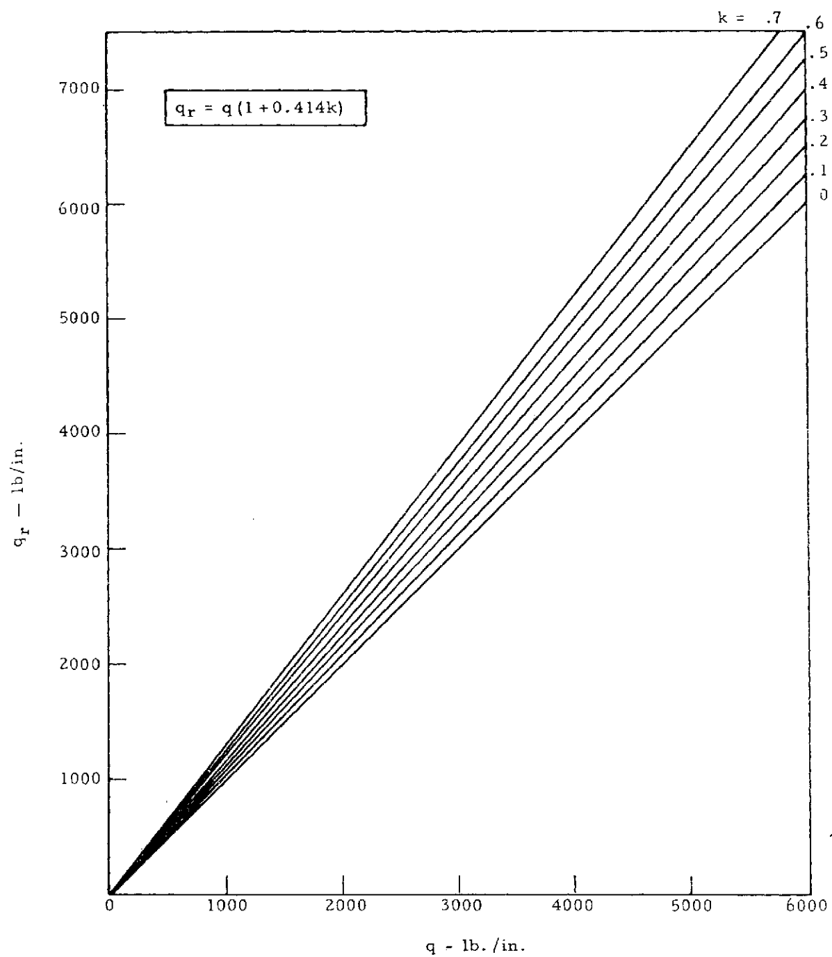
Figure 1-24. Rivet Loads—Web-to-Flange and Web Splices
