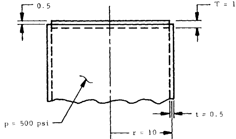
Figure 8-13. Thin Cylindrical Pressure Vessel with Flat Head
