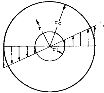
Figure 1-43. Stress Distribution of Circular Beam in Torsion
