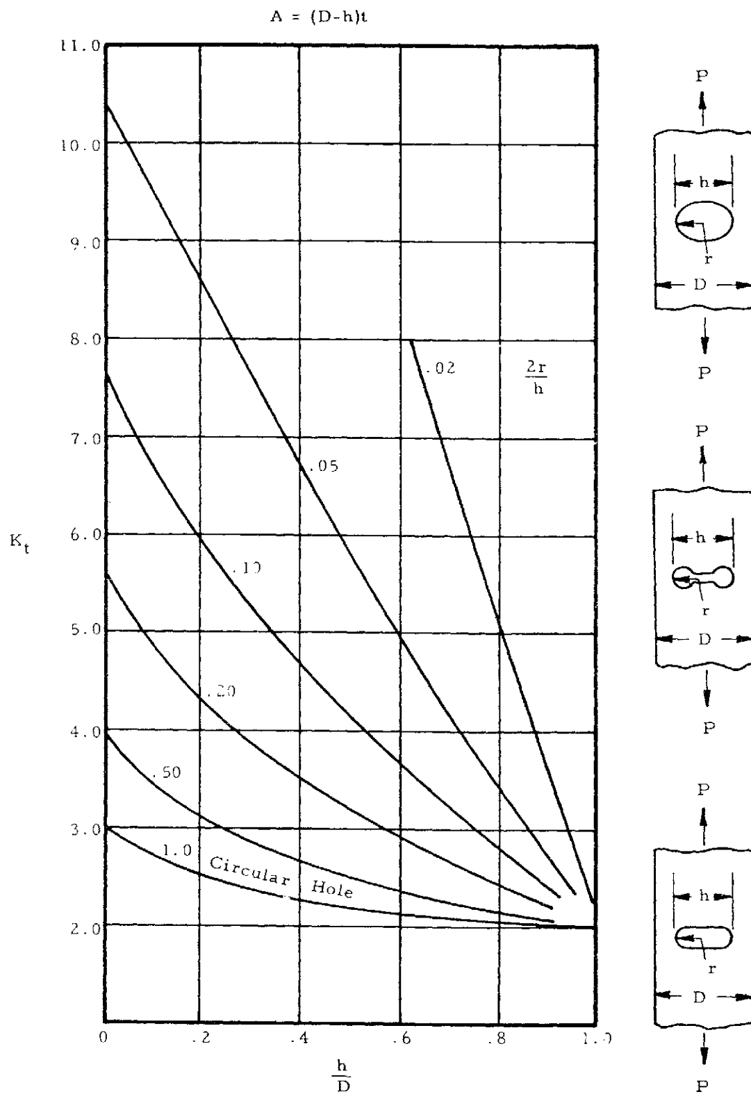
Figure 3-11. Rectangular Plate with Various Thru Sections
