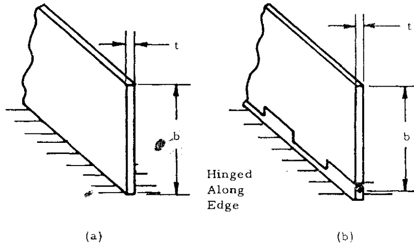
Figure 2-69. Idealized Edge Constraints of Long Flanges
