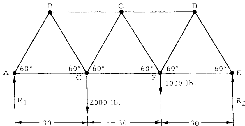
Figure 4-1. Planar Truss
