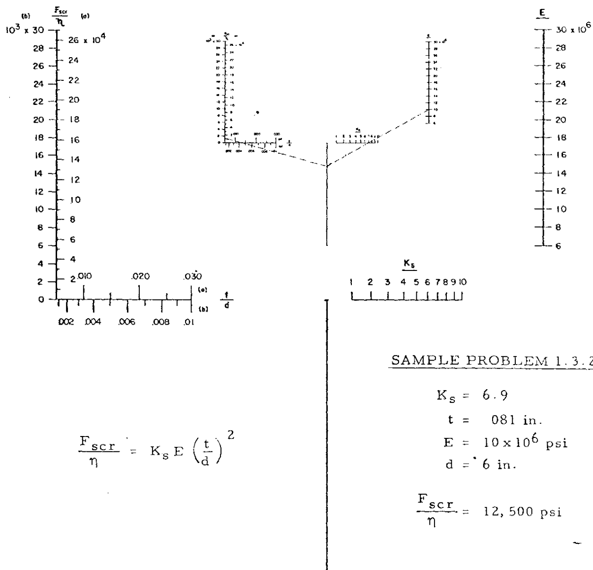
Figure 1-11. Nomograph for Critical Buckling Stress (Equation 1-19)
