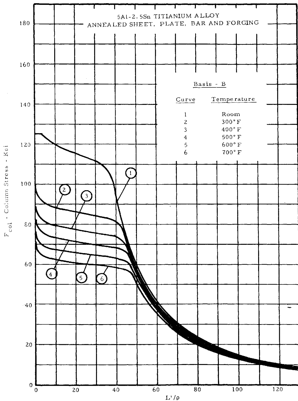
Figure 2-27. Column Allowable Curves
