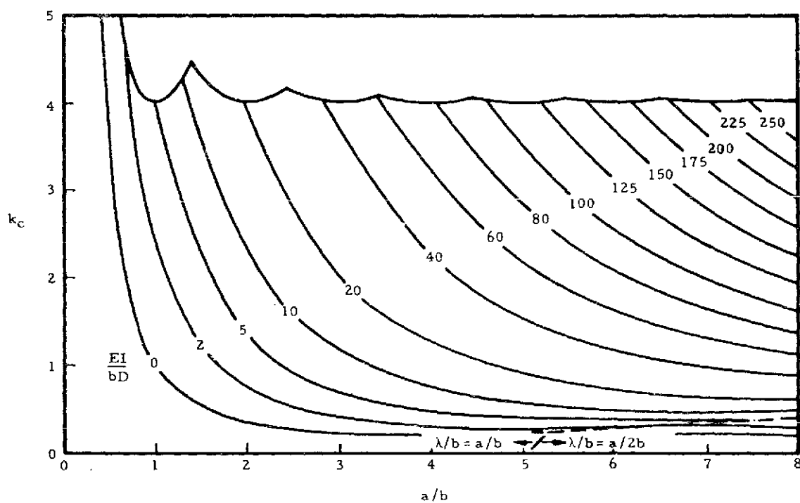
(h) Three stiffeners A/bt = 0.2
