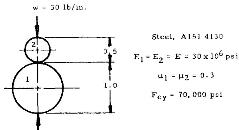
Figure 11-3. Cylinders in Contact
