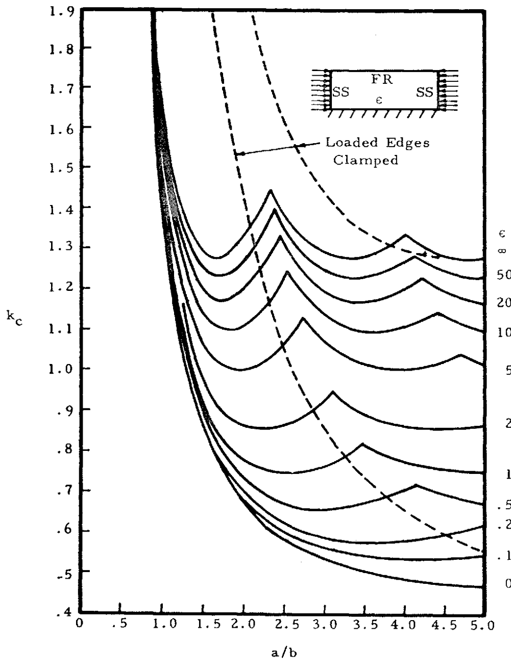
Figure 6-5. Compressive-Buckling-Stress Coefficient of Flanges as a Function of a/b for Various Amounts of Edge Rotational Restraint
