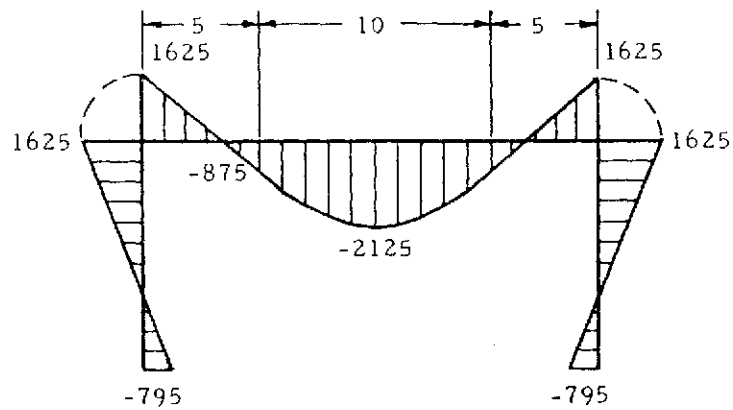
Figure 5-13. Moment Diagram for Frame in Figure 5-10
