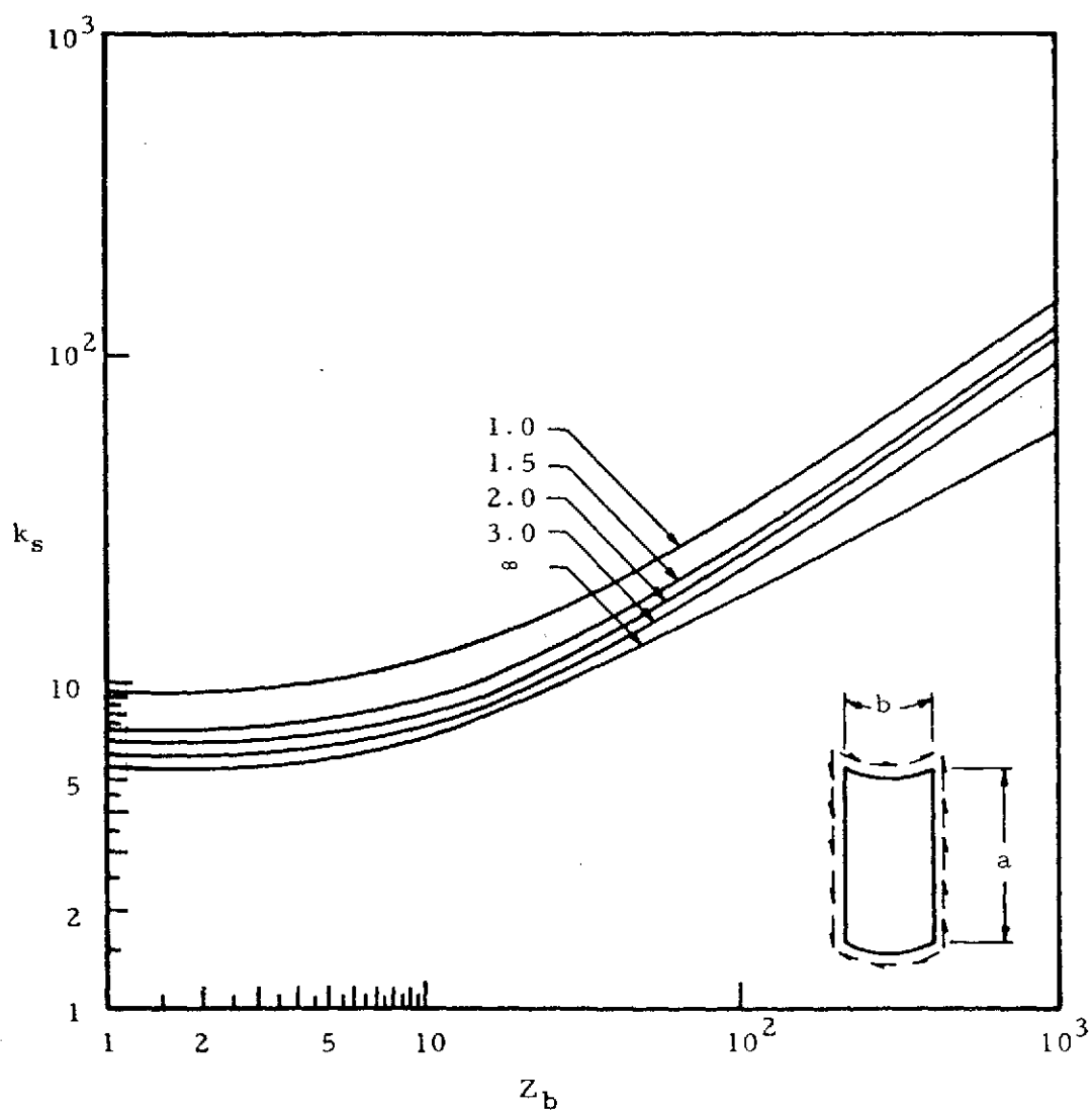
(a) Long simply supported plates
