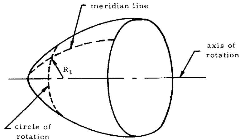
Figure 8-1. General Shell of Revolution
