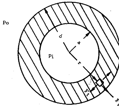
Figure 8-50. Thick Cylindrical Pressure Vessel
