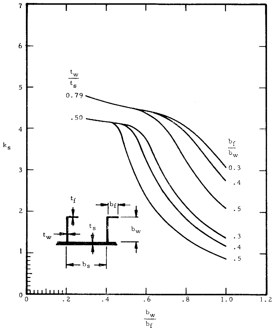
(b) Z-section stiffeners t_w/t_s = 0.50 and 0.79
