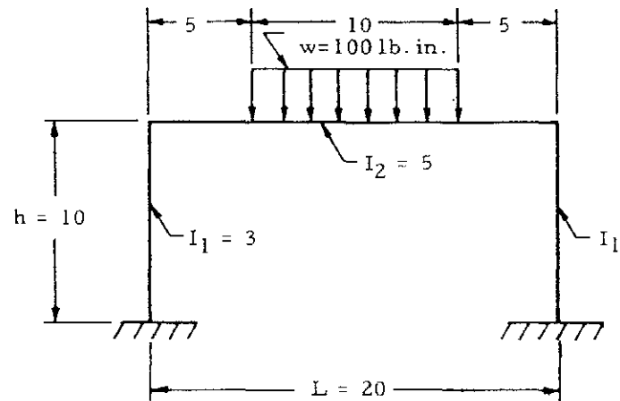
Figure 5-10. Rectangular Frame
