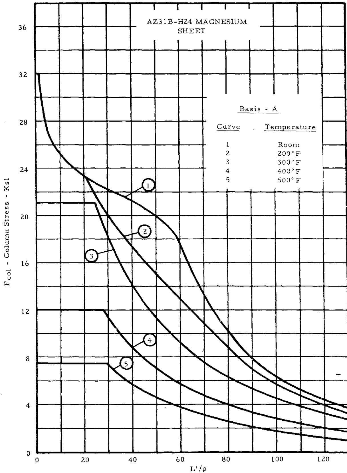
Figure 2-13. Column Allowable Curves
