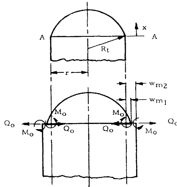
Figure 8-7. Illustration of the Necessity of Discontinuity Stresses *
