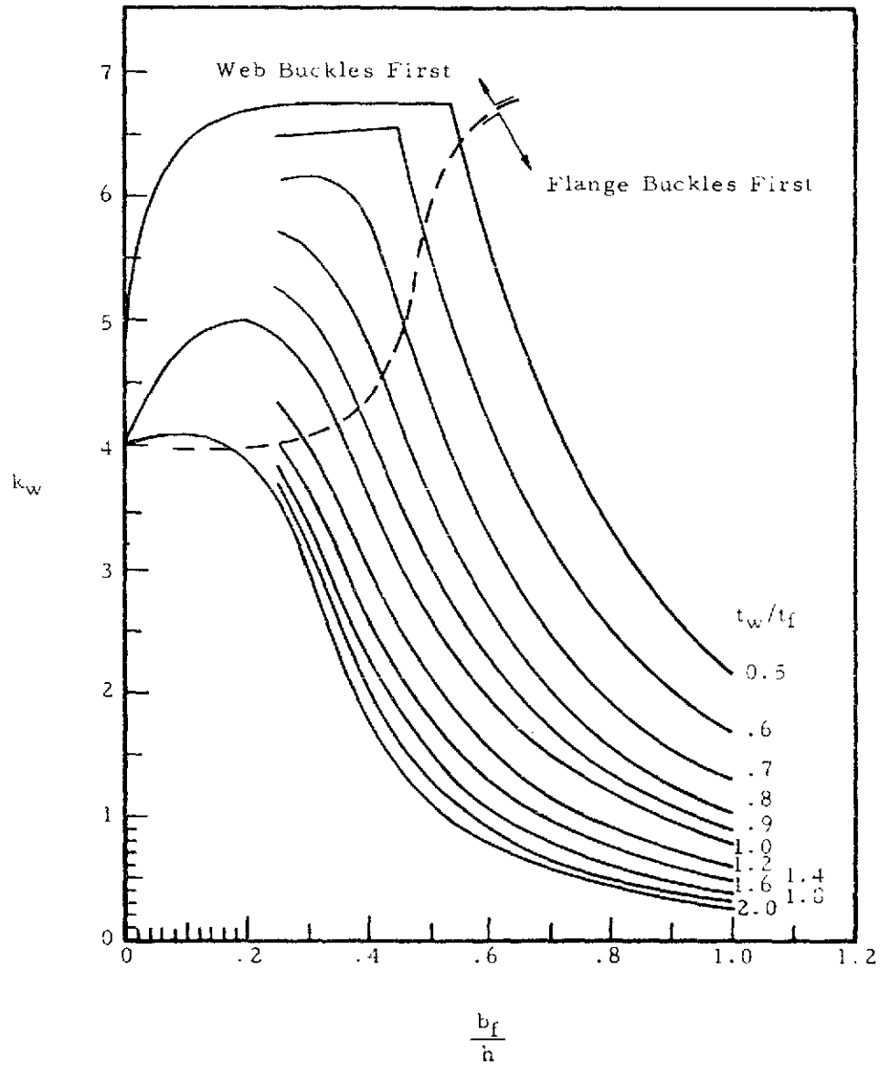
Figure 2-76. k_w for Equation (2-30)
