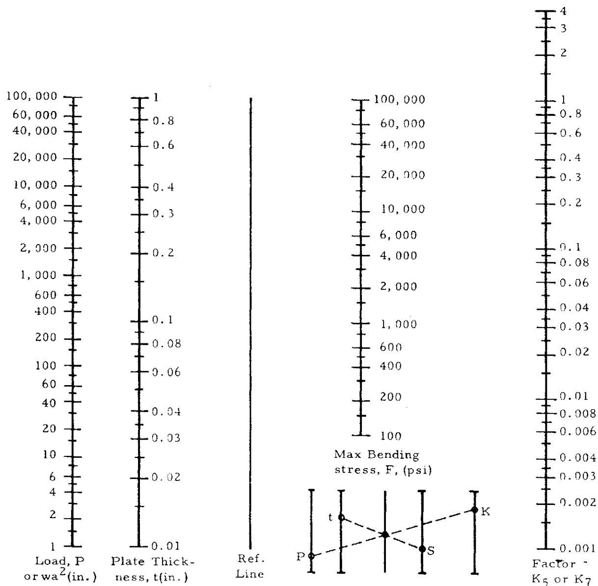
Figure 6-25. Nomogram for Determining Plate Stress F_b *
