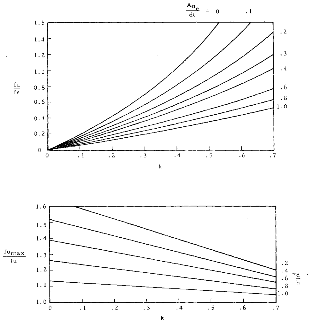
Figure 1-22. Upright Stress Ratios
