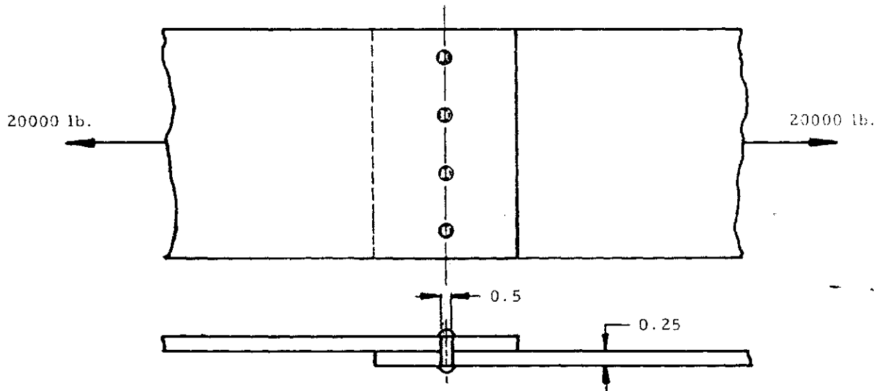
Figure 11-2. Riveted Plate
