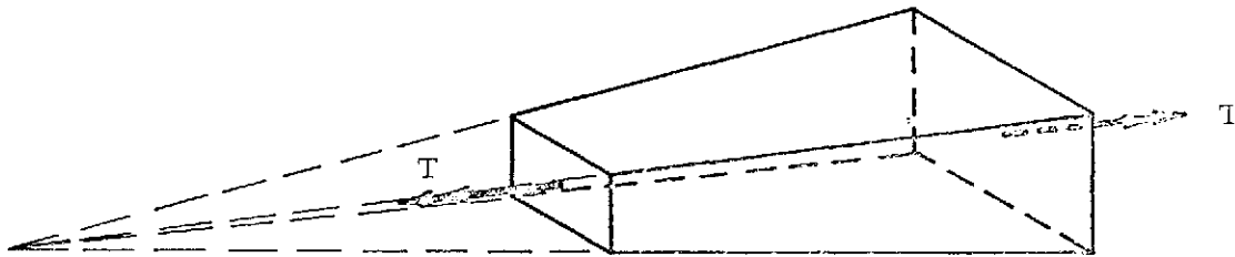
Figure 1-55. Tapered Box Beam in Torsion
