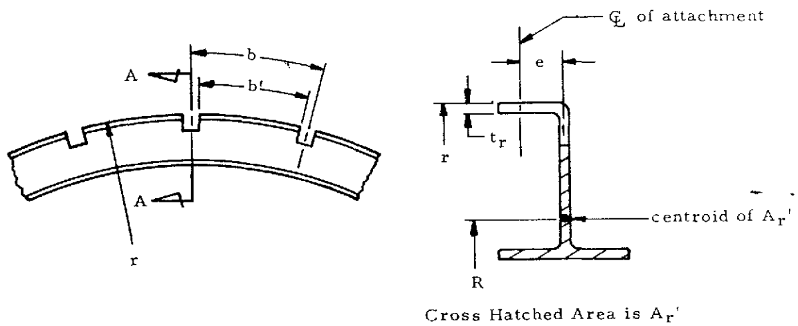
Figure 8-40. Section of Stiffening Ring
