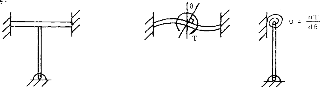
Figure 2-37. Example of Equivalent Torsional Spring
