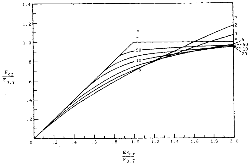
Figure 6-33. Nondimensional Buckling Chart for Axially Compressed Curved Plates
