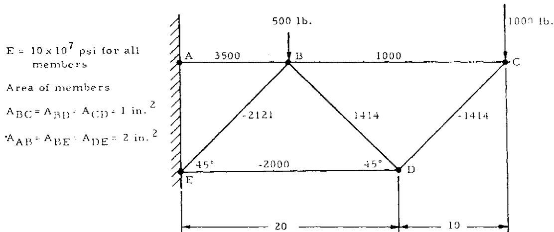
Figure 4-4. Cantilever Truss
