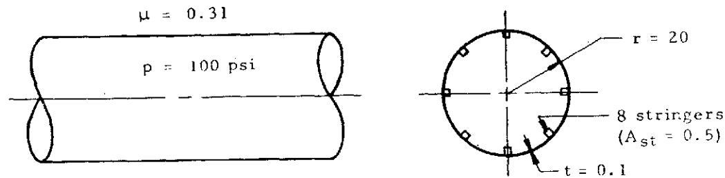
Figure 8-38. Thin Cylindrical Pressure Vessel with Stringers
