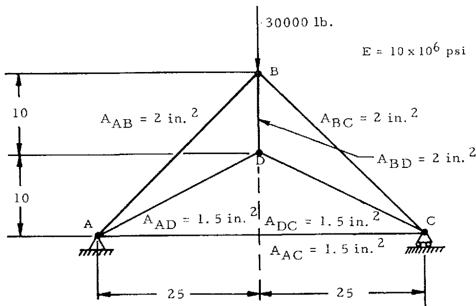
Figure 4-6. Statically Indeterminate Truss With a Single Redundancy
