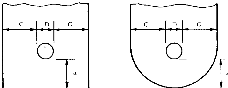
Figure 9-21. Lug Geometry for Fatigue Analysis
