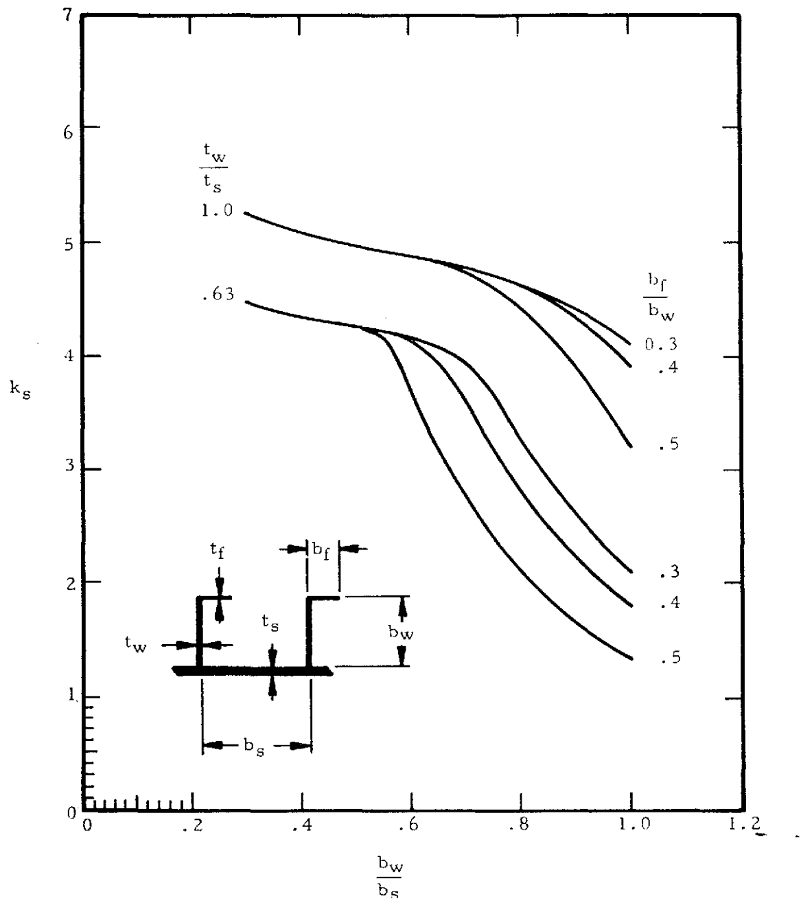
(c) Z-section stiffeners t_w/t_s = 0.63 and 1.0
