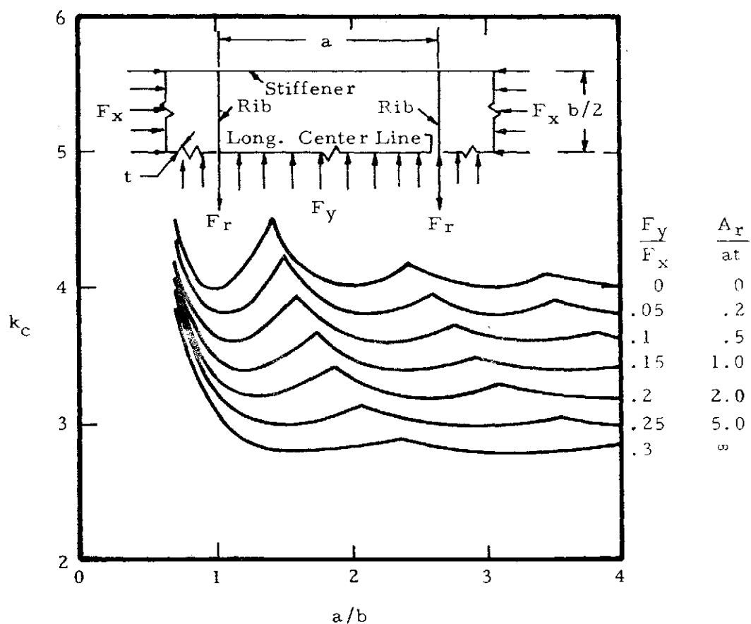
Figure 6-9. Compressive-Buckling Coefficient of Flat Plates Restrained Against Lateral Expansion. Poisson's Ratio Equals 0.3;
