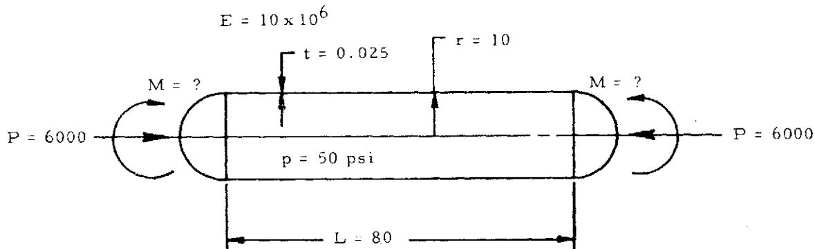
Figure 8-36. Pressurized Cylinder in Compression and Bending
