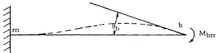
Figure 5-2. Illustration of Carry-Over Moment
