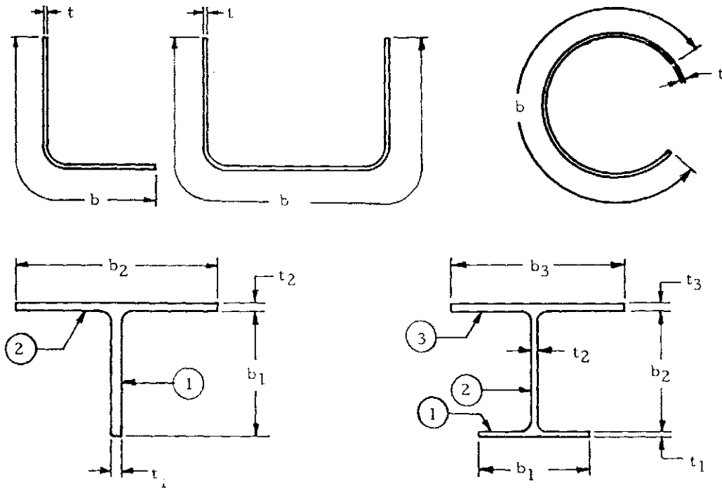
Figure 1-52. Beams Composed of Thin Rectangular Members
