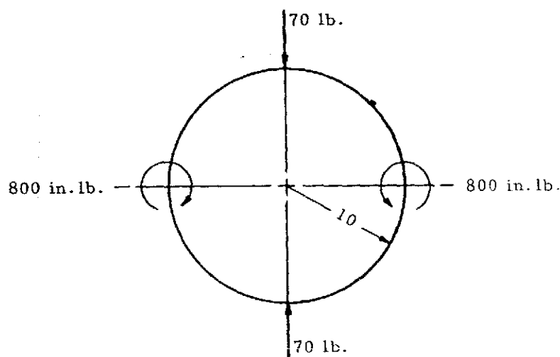
Figure 5-18. Circular Ring
