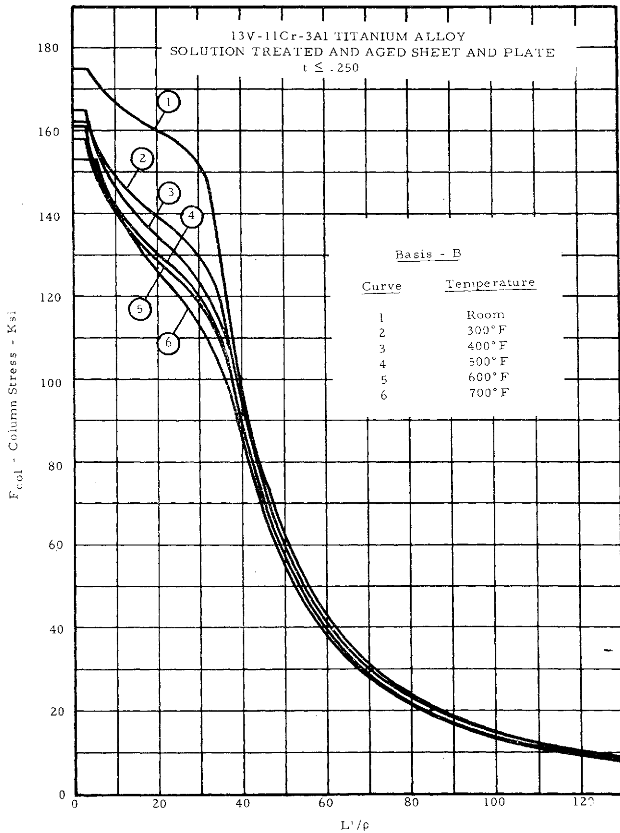
Figure 2-33. Column Allowable Curves
