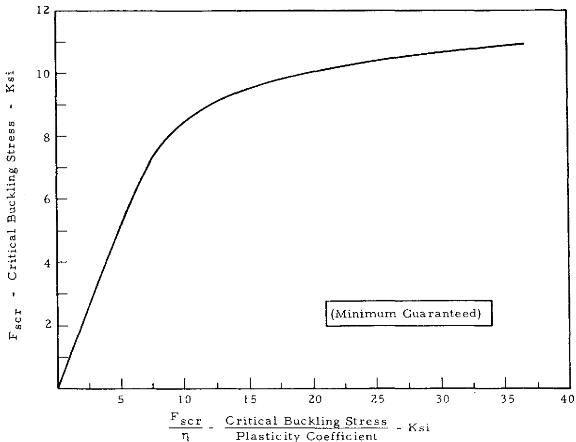
Figure 1-16. F_{scr} versus F_{scr}/\eta for 356-T6 Sand Casting
