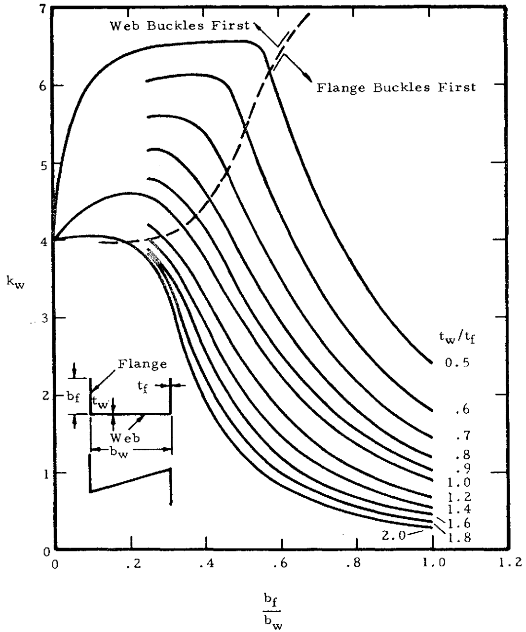
(a) Channel- and Z-section stiffeners
