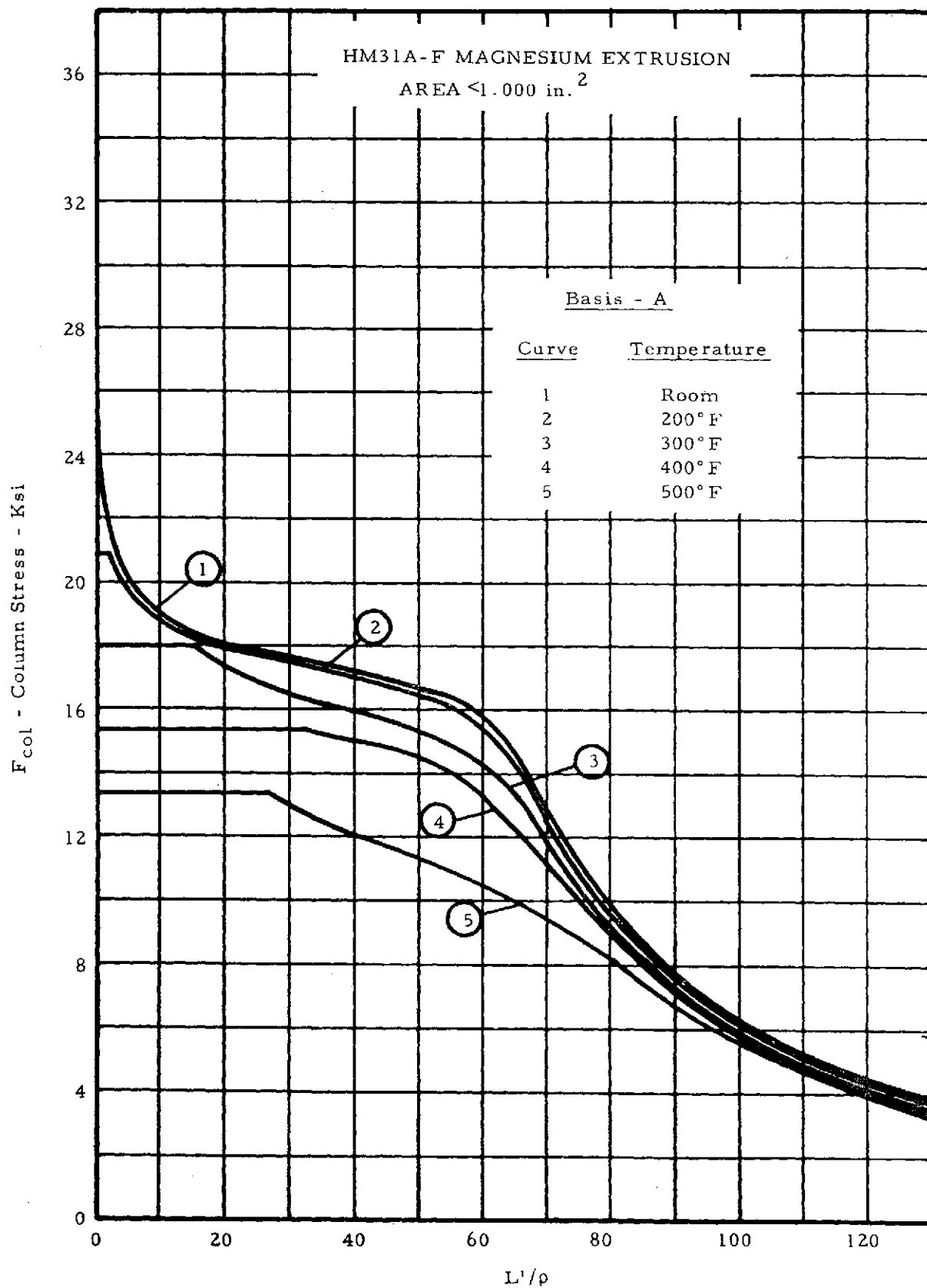
Figure 2-15. Column Allowable Curves
