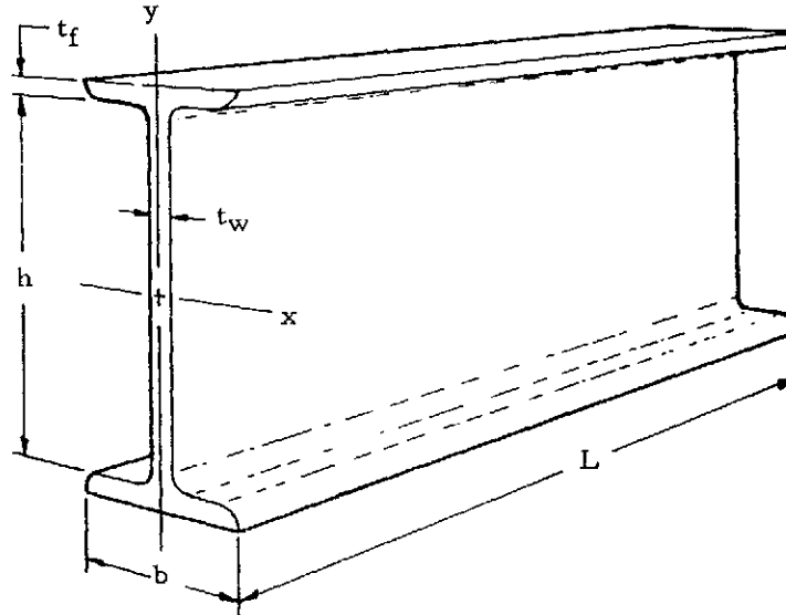
Figure 1-7. Deep I Beam
