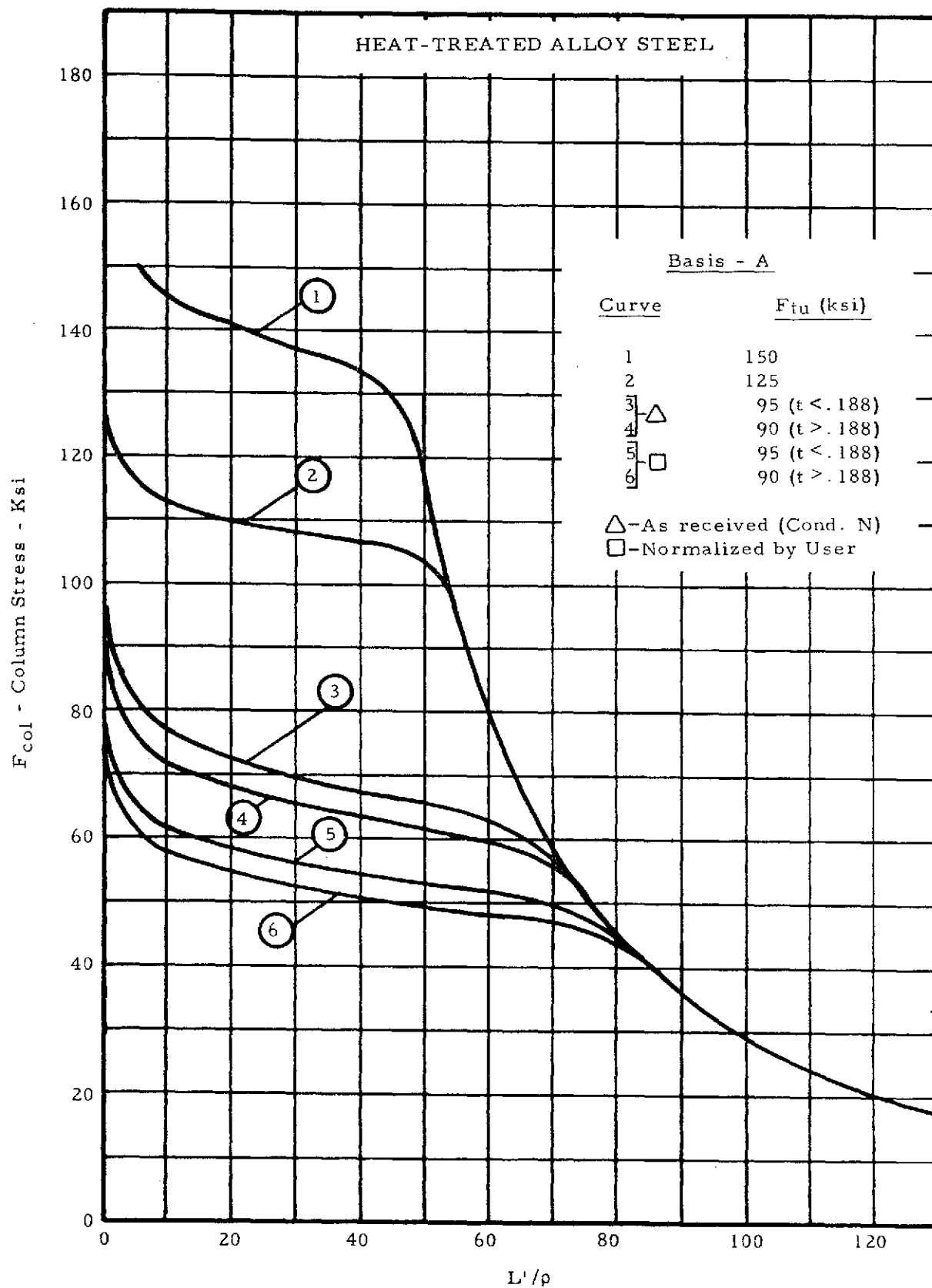
Figure 2-18. Column Allowable Curves
