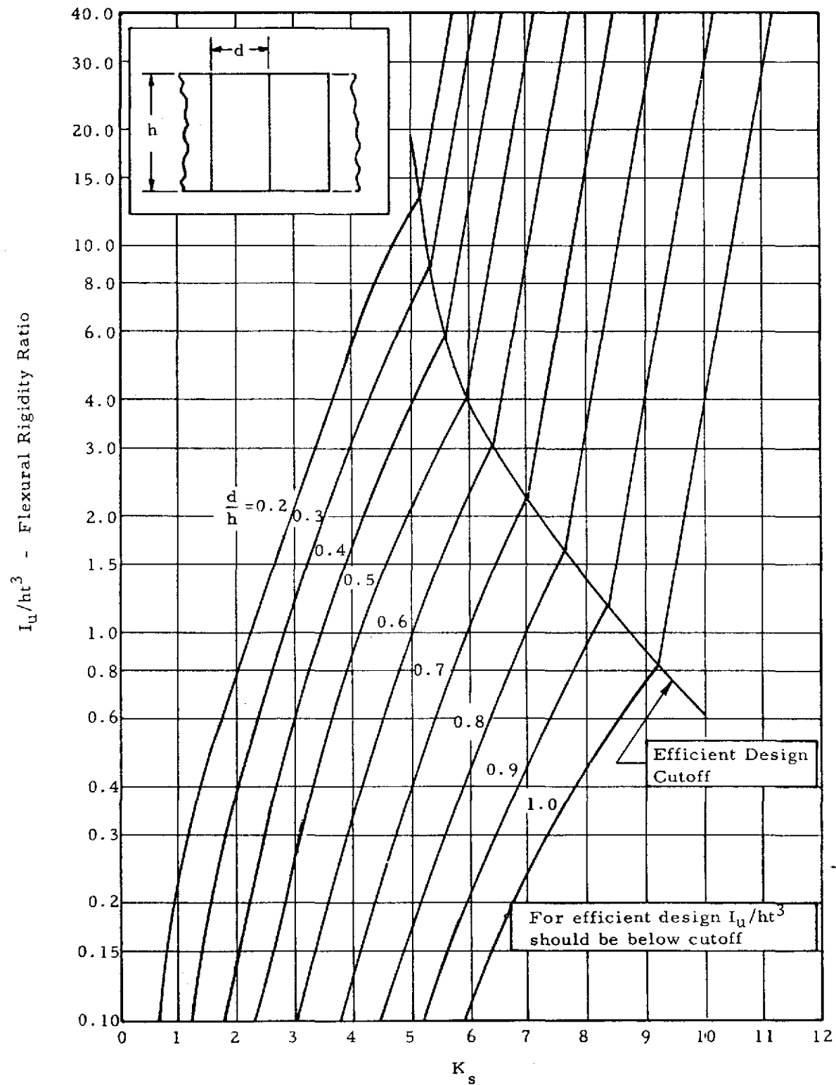
Figure 1-10. Critical Shear Stress Coefficient, K_s
