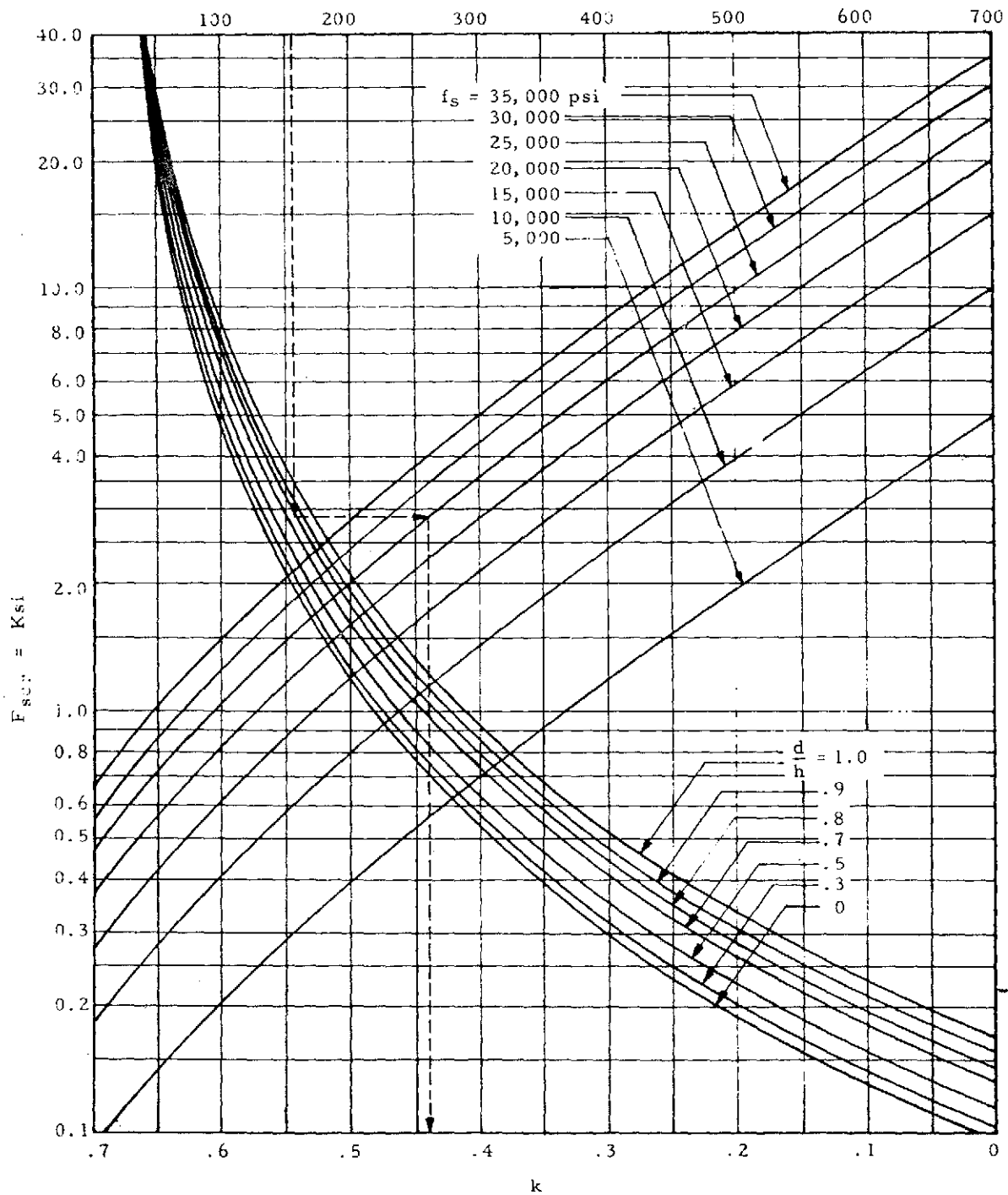
Figure 1-18. Diagonal Tension Factor, k , and Initial Buckling Stress, F_{scr} , for Shear Webs with Simply Supported Edges, E = 10 \times 10^6 psi
