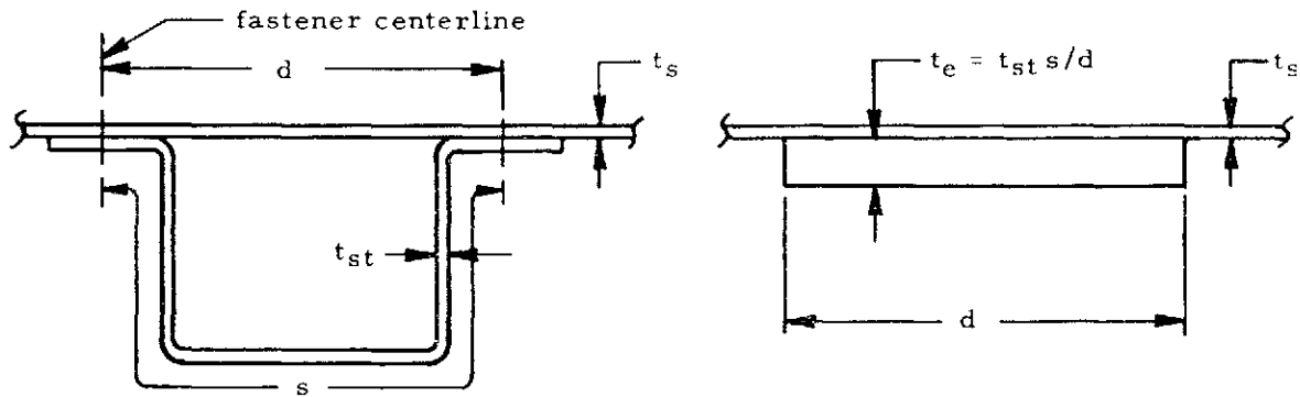
Figure 1-58. First Method of Transforming Closed Stiffeners
