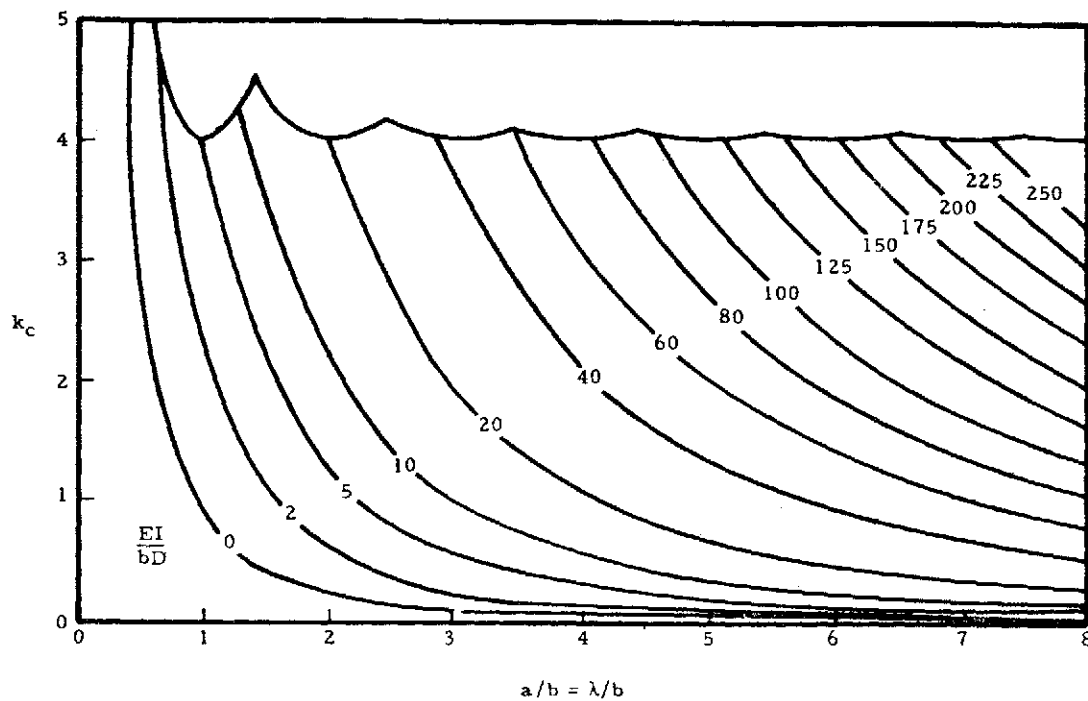
(k) Infinite number of stiffeners A/bt = 0.2
