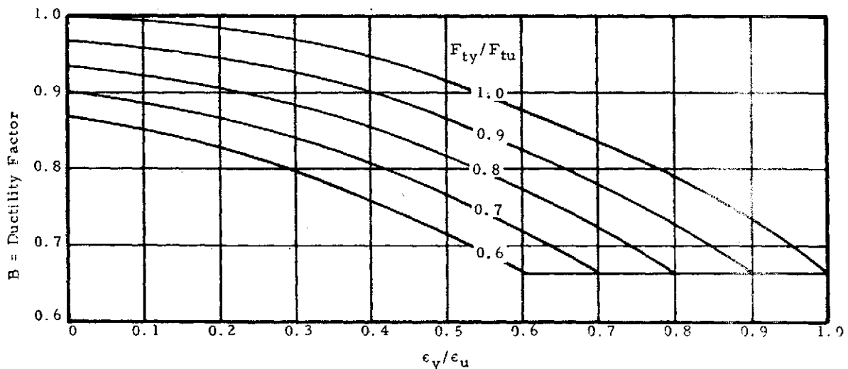
Figure 9-17. Ductility Factor
