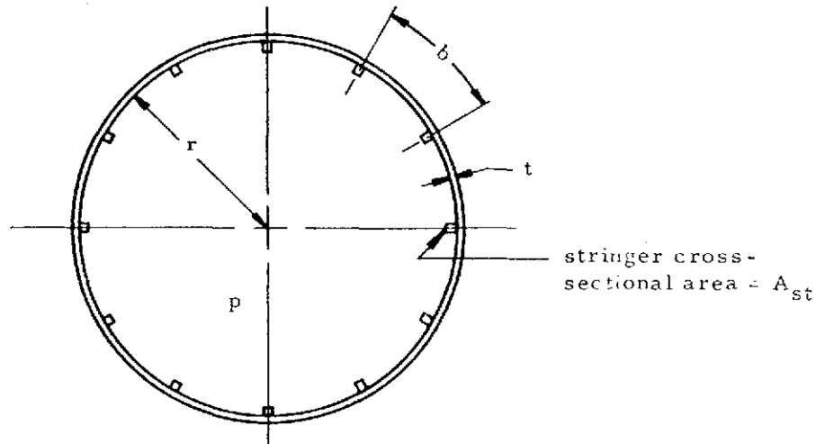
Figure 8-37. Cross Section of Shell with Stringers
