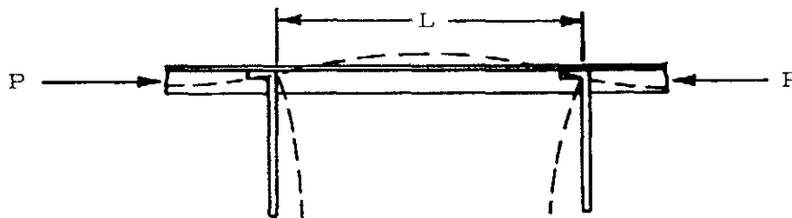
Figure 2-43. Semimonocoque Structure
