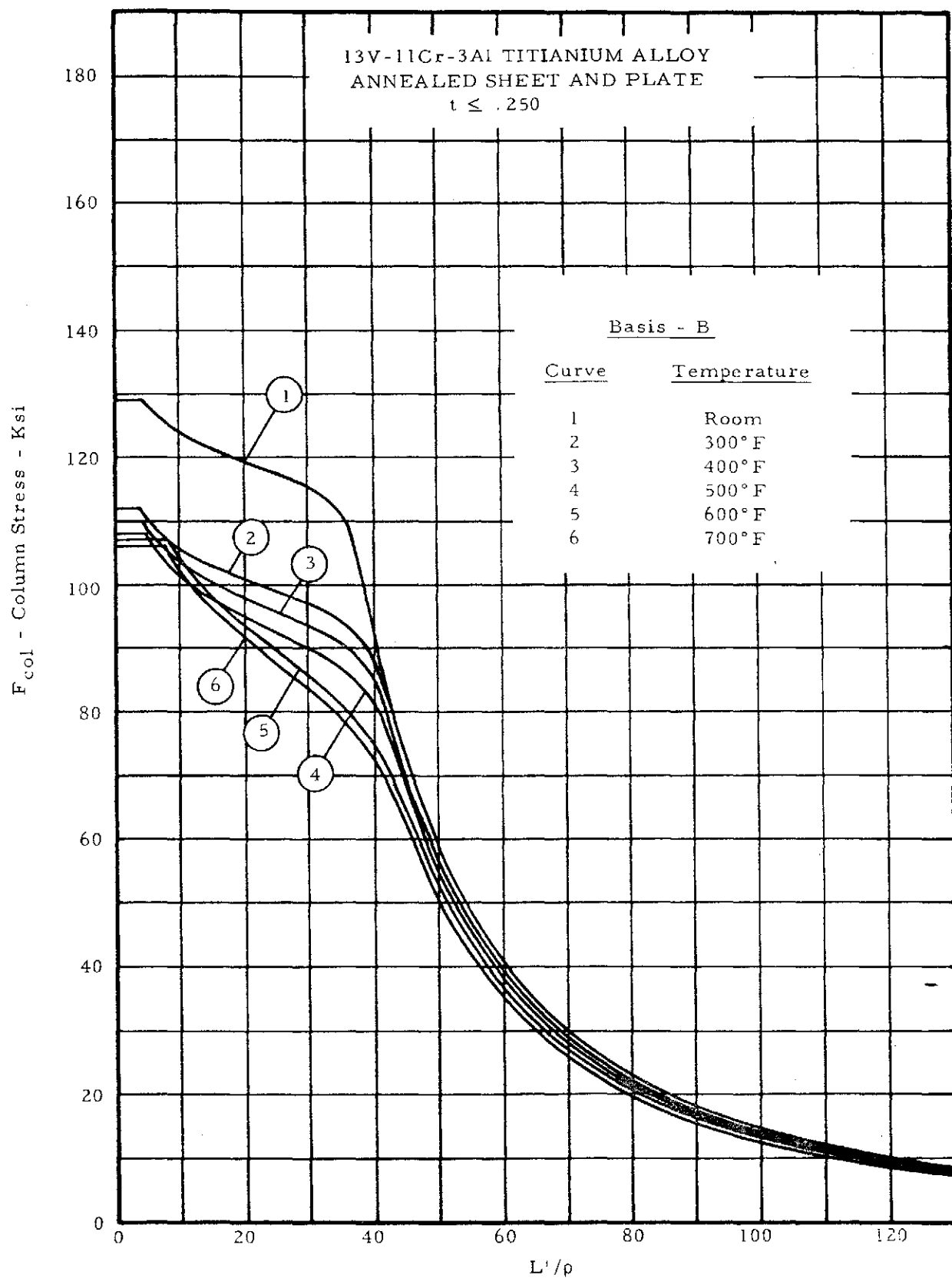
Figure 2-34. Column Allowable Curves
