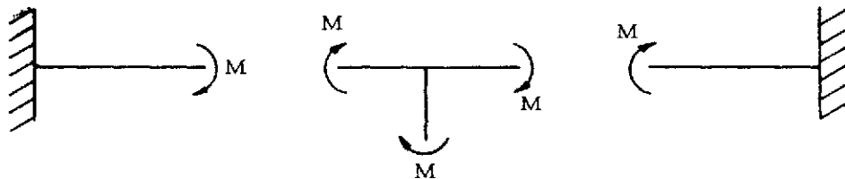
Figure 5-3. Positive Sense for Bending Moments
