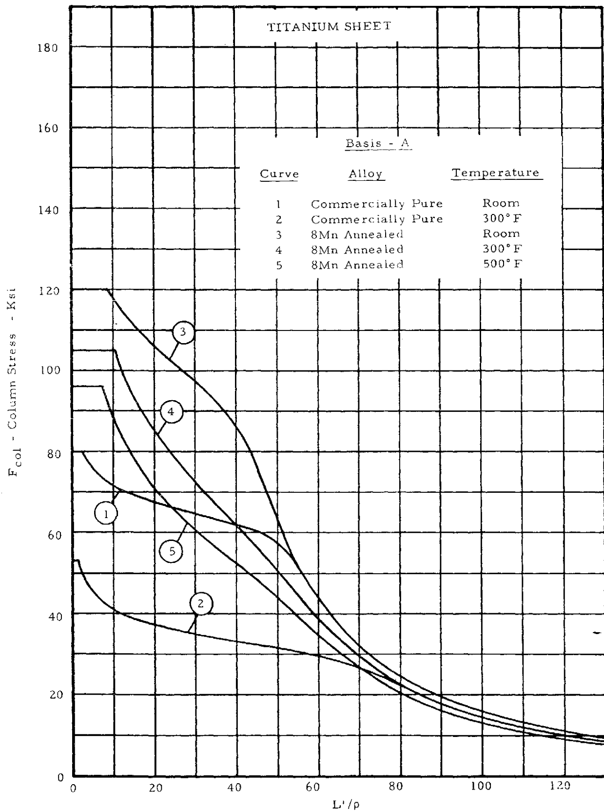
Figure 2-25. Column Allowable Curves
