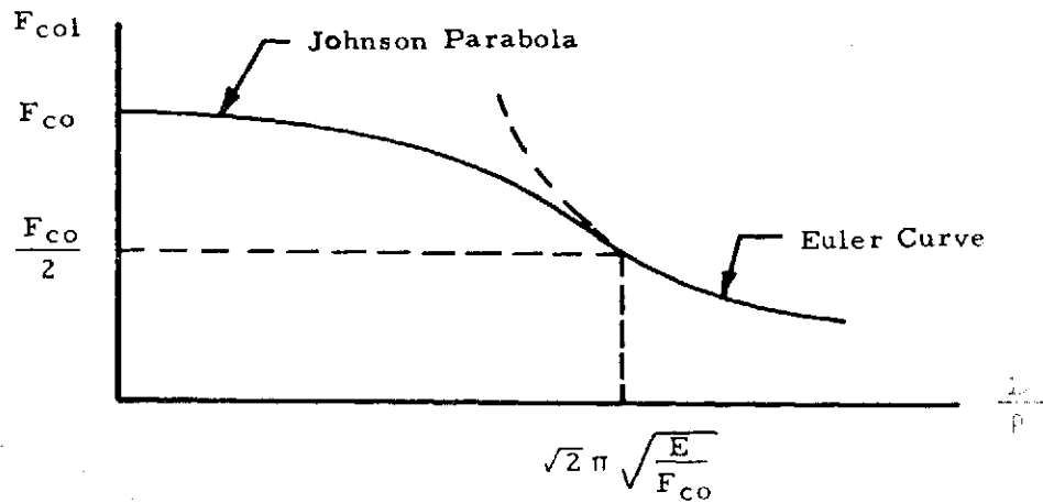
Figure 2-50. Typical Johnson-Euler Curve
