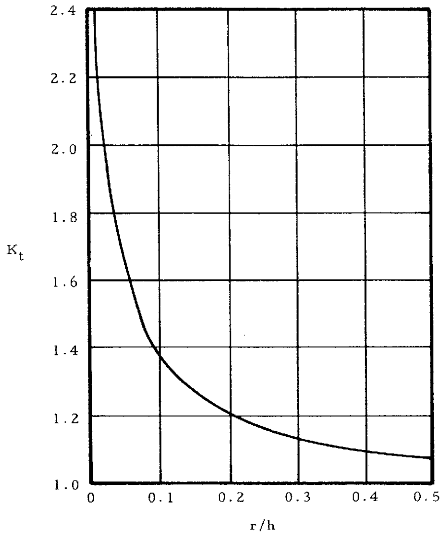
Figure 3-12. Rectangular Bar with Protrusion on One Side
