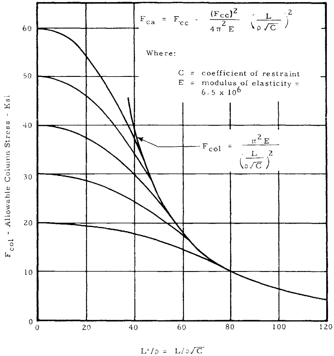
Figure 2-64b. Johnson-Euler Column Curve
