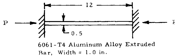
Figure 2-52. Concentrically Loaded Short Column
