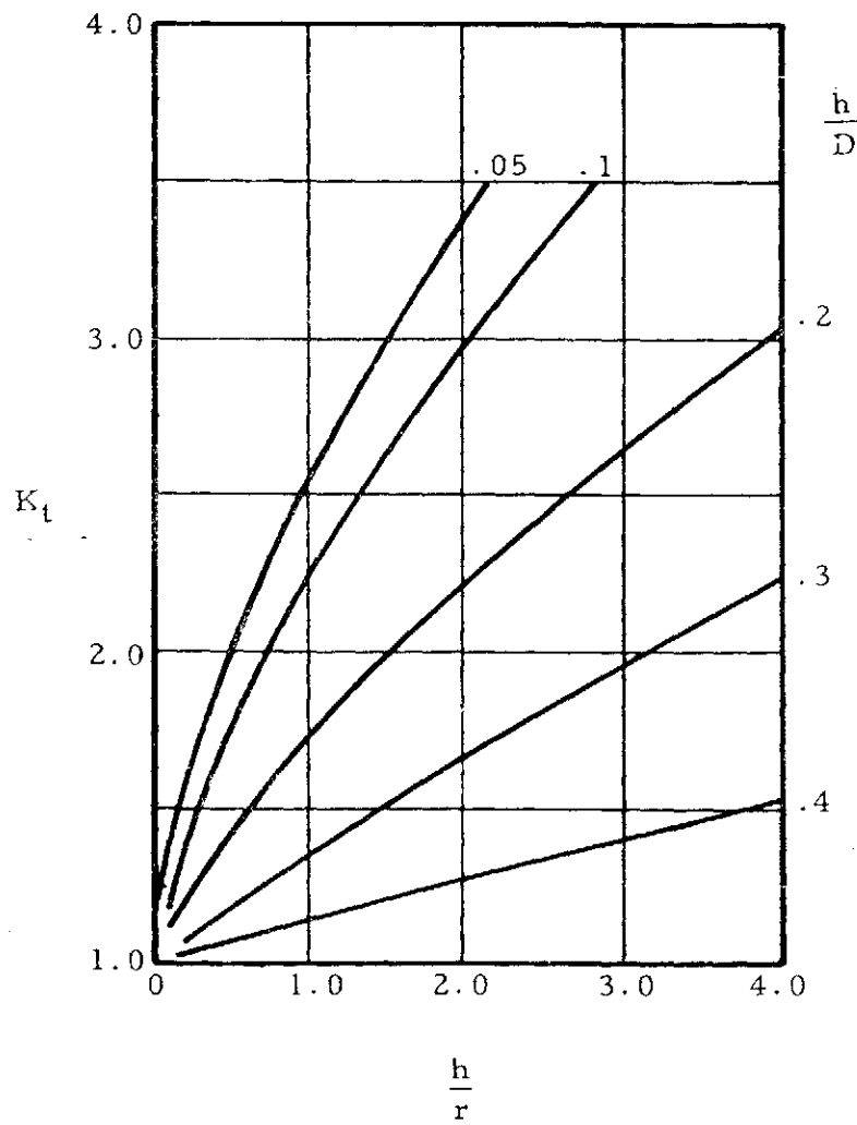
Figure 3-7. Rectangular Bar with U Notch (Both Sides)
