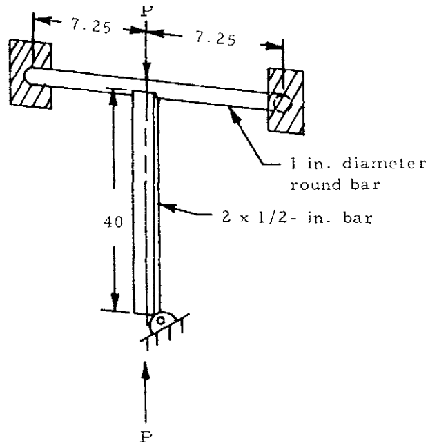
Figure 2-45. Example of Constrained Column
