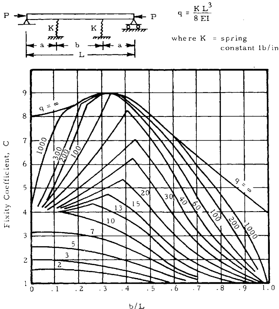
Figure 2-41. Fixity of a Column with Two Elastic, Symmetrically Placed Supports Having Spring Constants, K
