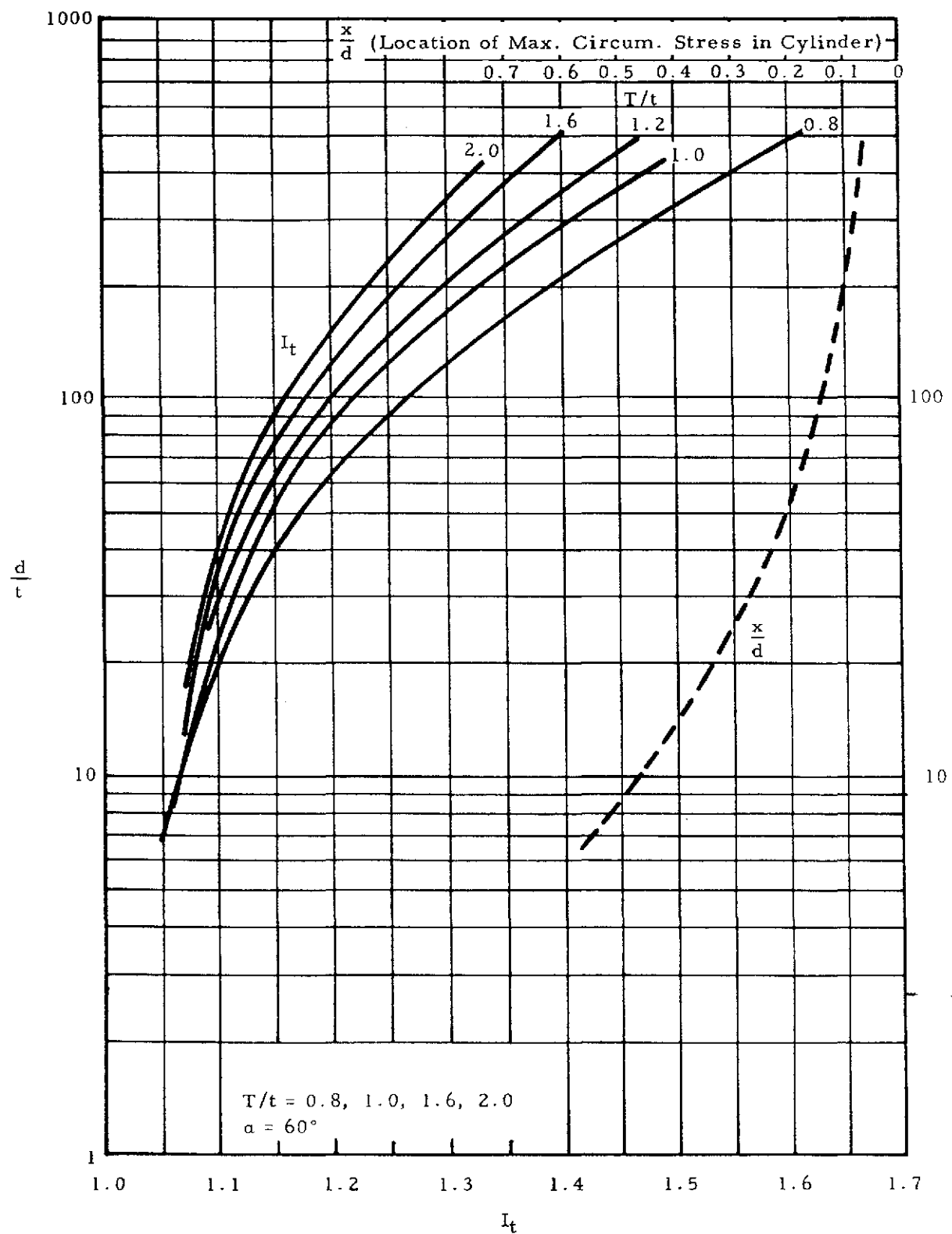
Figure 8-22. Stress Ratios for Pressure Vessels with Conical Head Closures *
