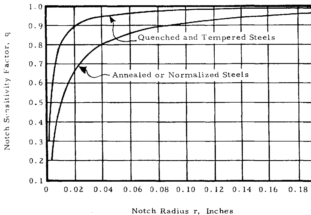
Figure 3-15. Average Notch Sensitivity Curves. Applicable Particularly to Normal Stresses; Used Also for Shear Stresses
