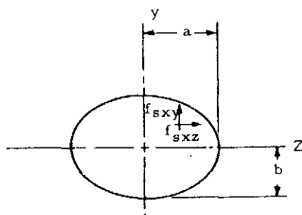
Figure 1-50. Cross Section of Elliptical Beam in Torsion
