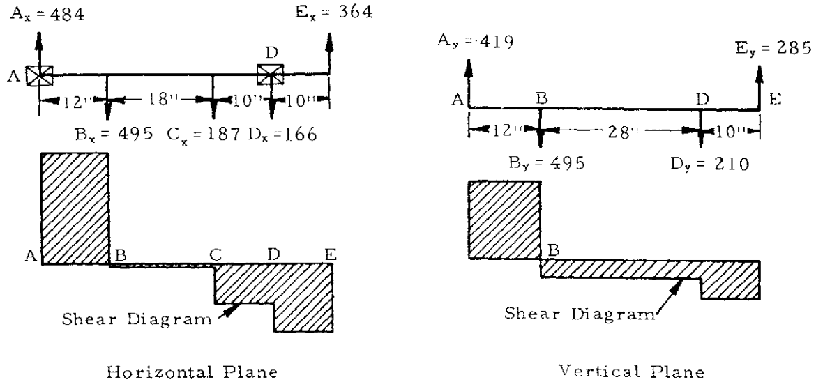
Figure 10-7. Drawing Illustrating Construction of Shear Diagrams
