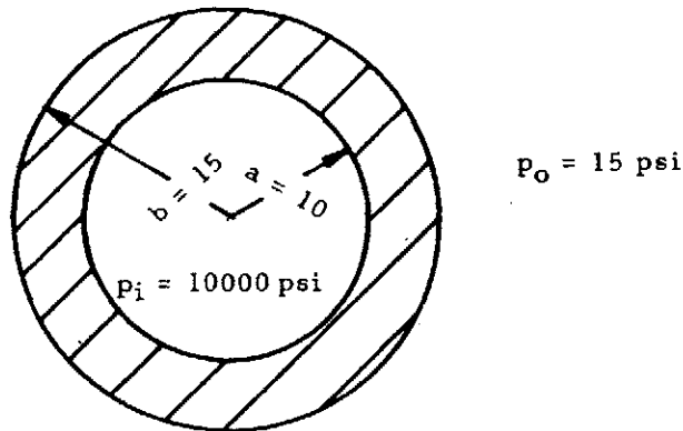
Figure 8-51. Thick Cylindrical Pressure Vessel
