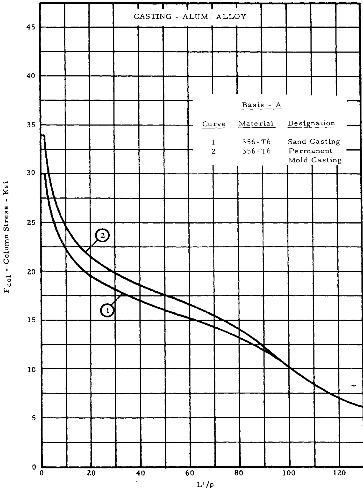
Figure 2-11. Column Allowable Curves
