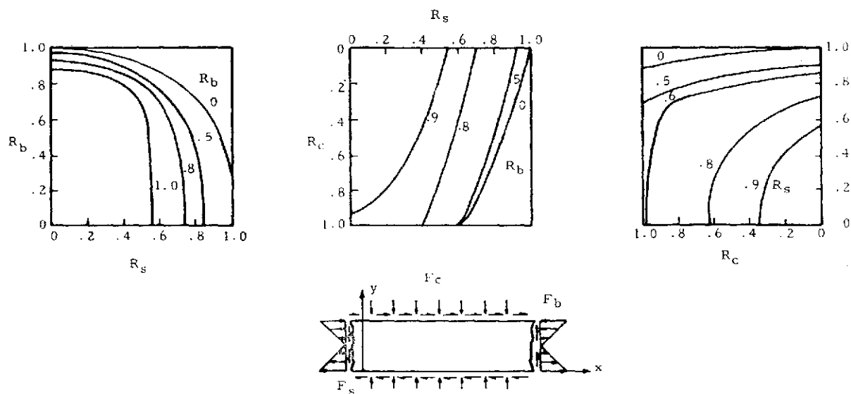
(a) Upper and lower edges simply supported
