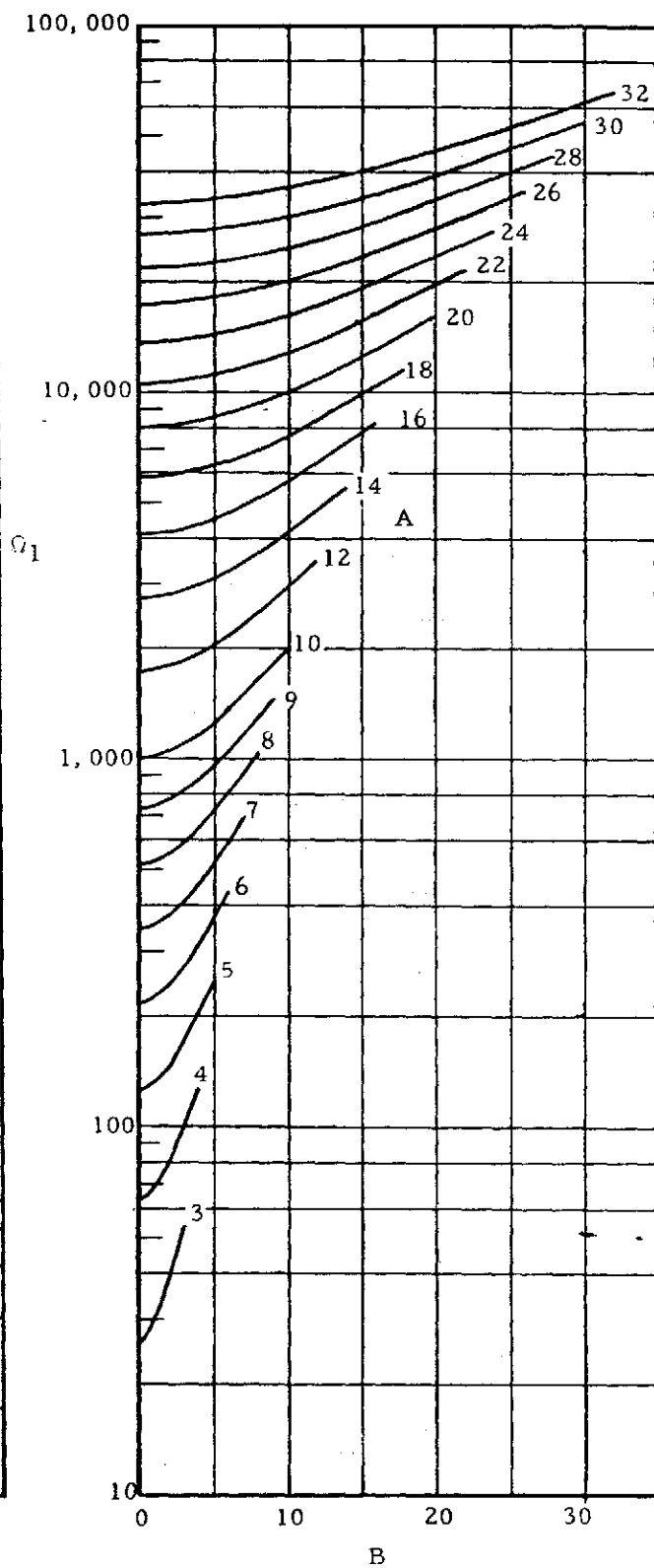
Figure 8-41. \Omega_1 as a Function of A and B
