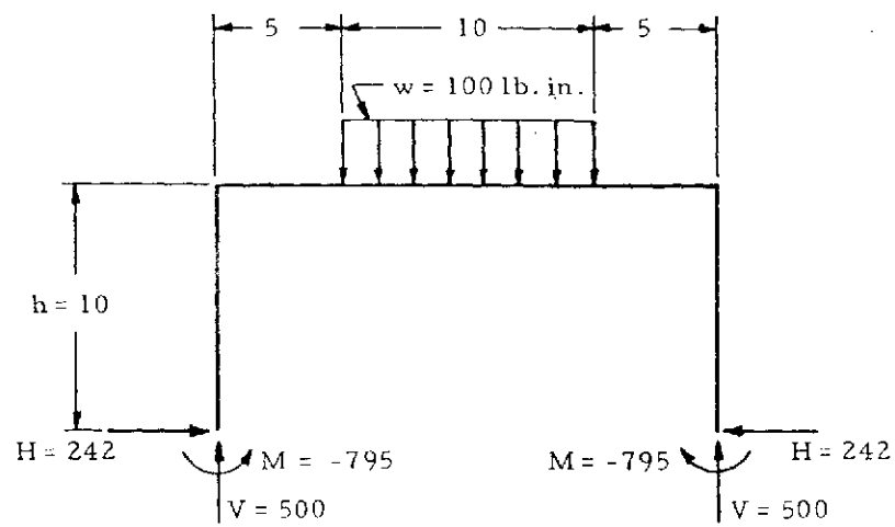
Figure 5-12. Free-Body Diagram of Frame in Figure 5-10
