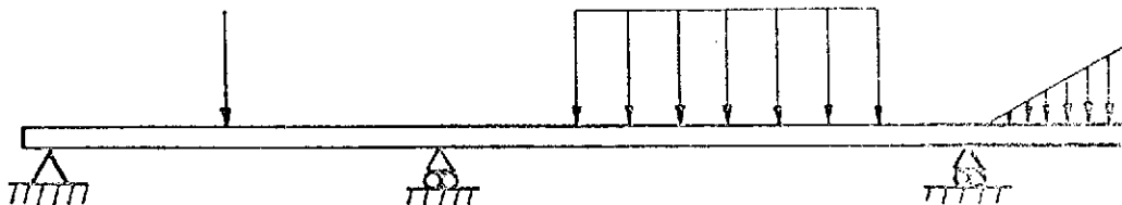
Figure 1-30. Beam Under Transverse Loading
