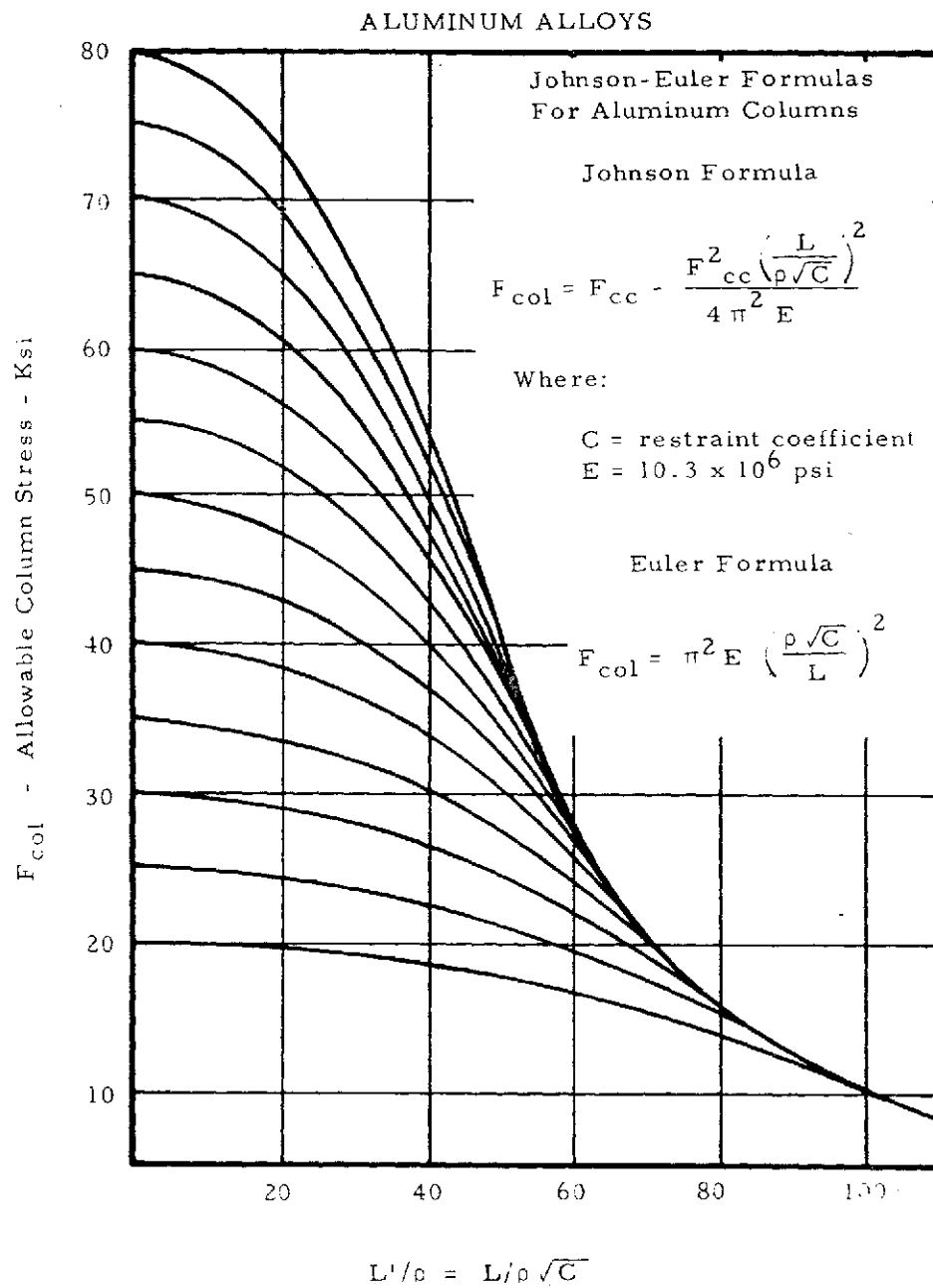
Figure 2-64a. Johnson-Euler Column Curve
