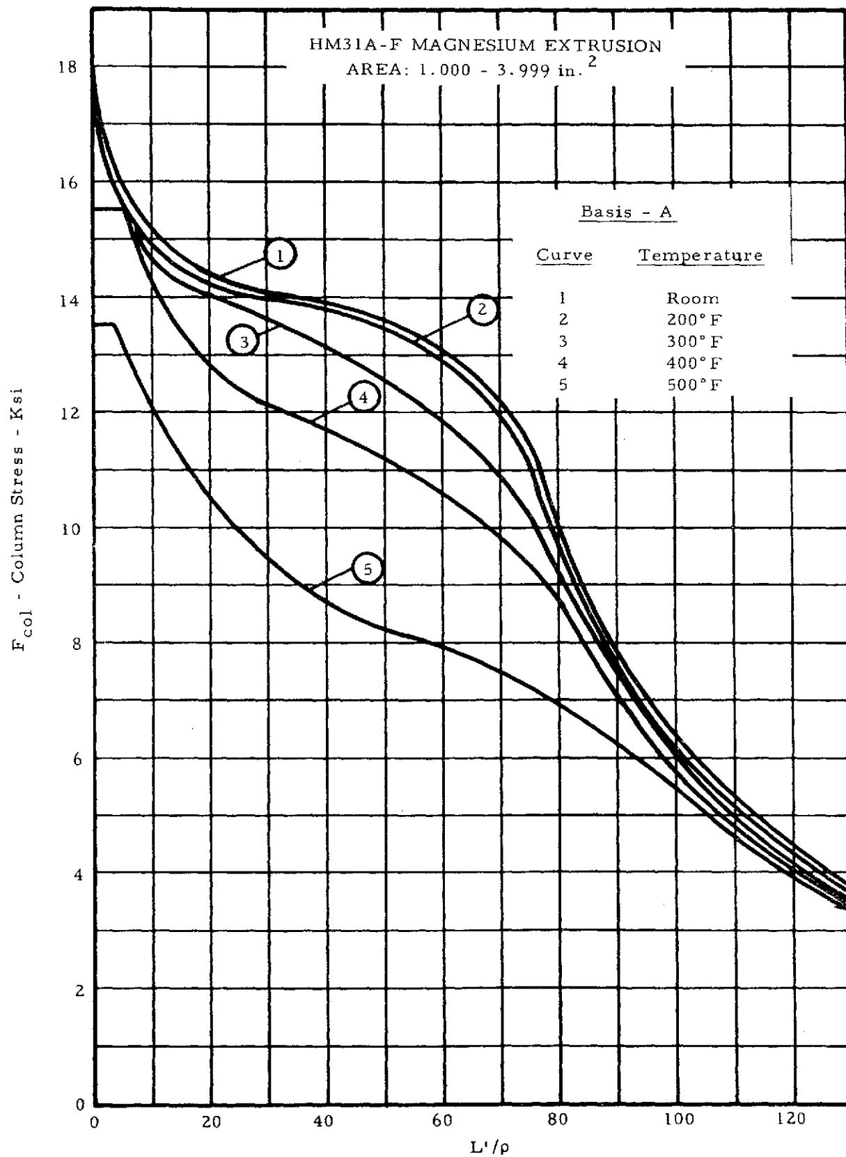
Figure 2-16. Column Allowable Curves
