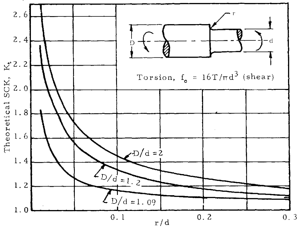
Figure 10-1. Stress Concentration Factor for Solid Shaft with Fillet (concluded)
