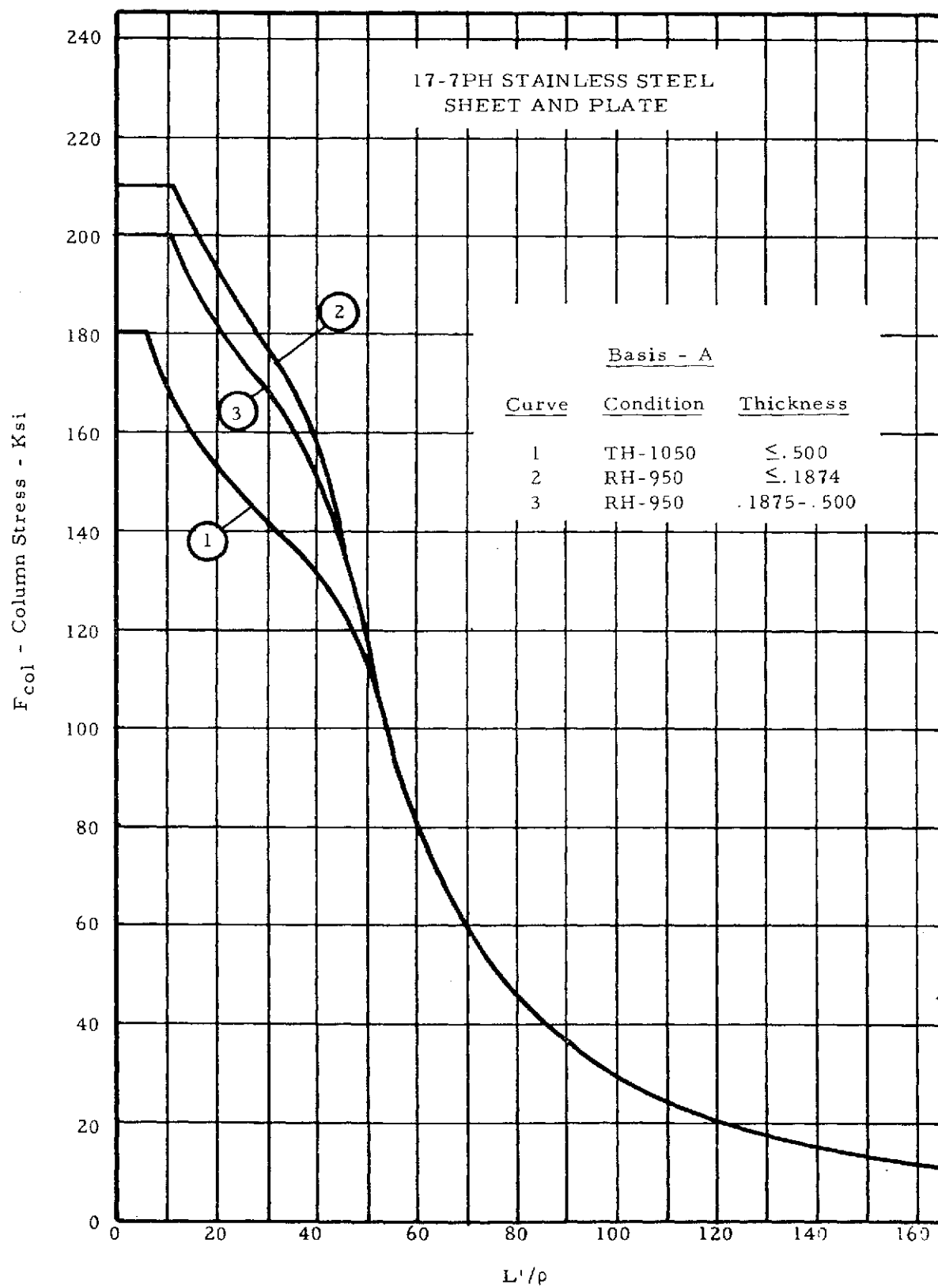
Figure 2-24. Column Allowable Curves
