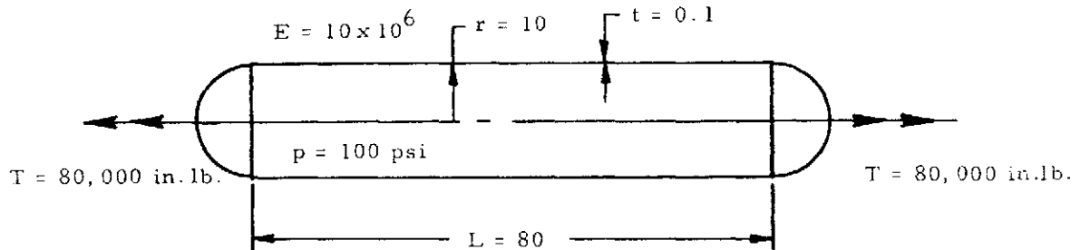
Figure 8-35. Pressurized Cylinder in Torsion
