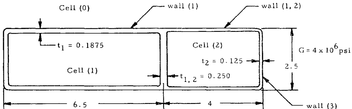
Figure 1-64. Two Cell Closed Beams
