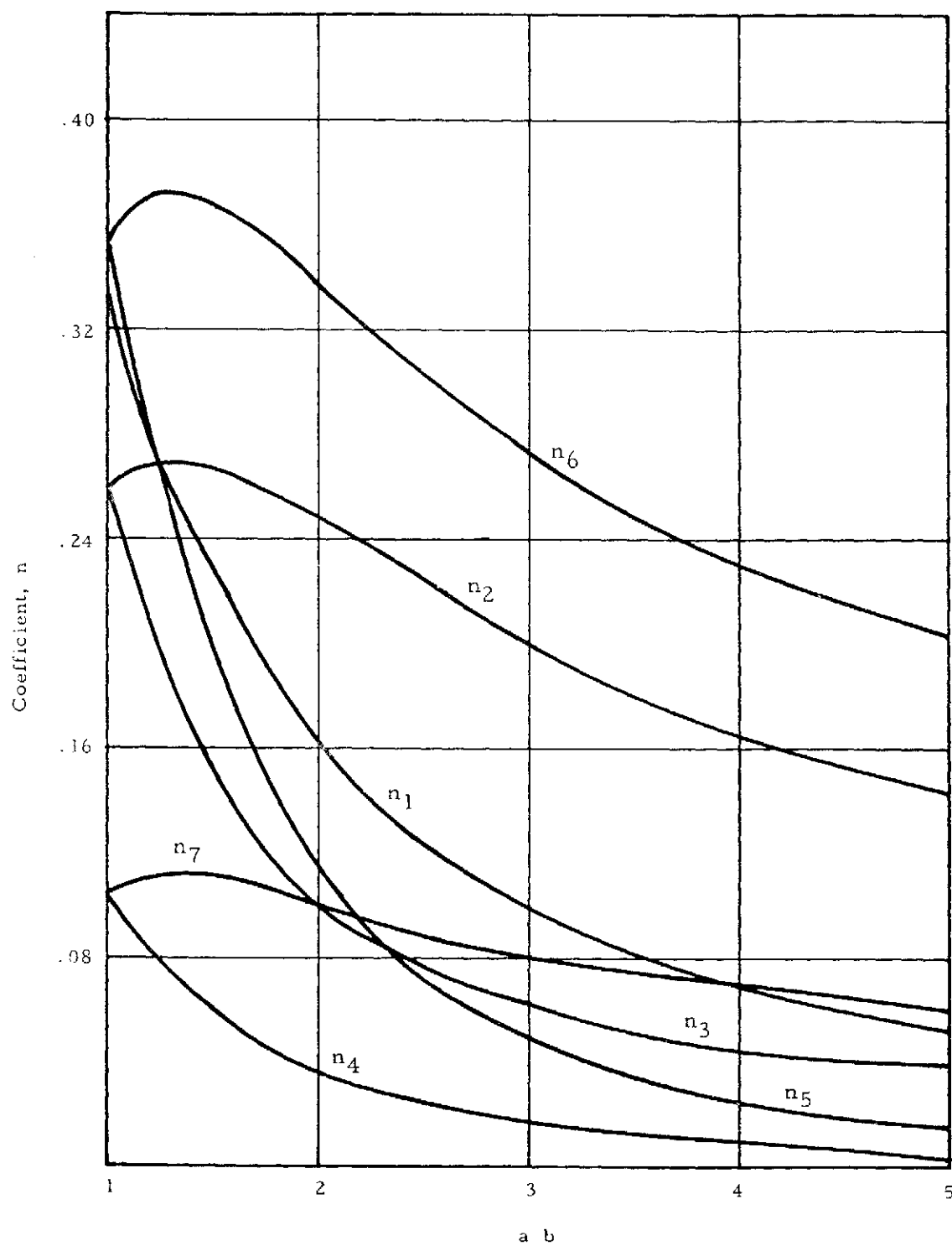
Figure 7-9. Coefficients for Equations (7-7) Through (7-13)
