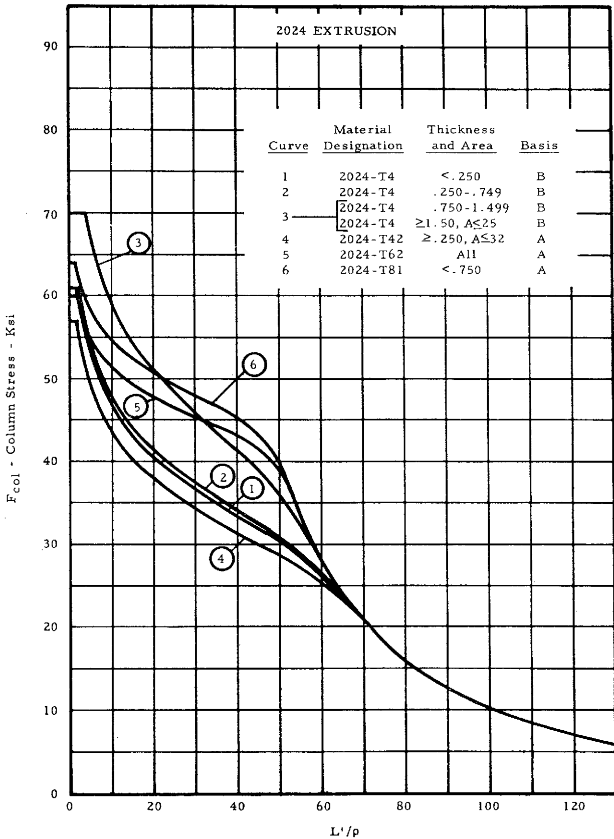
Figure 2-6. Column Allowable Curves
