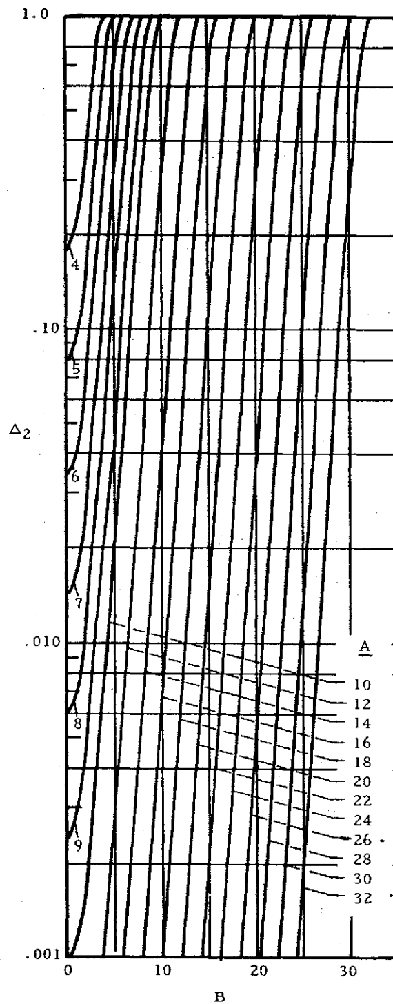
Figure 8-46. \Delta_2 as a Function of A and B
