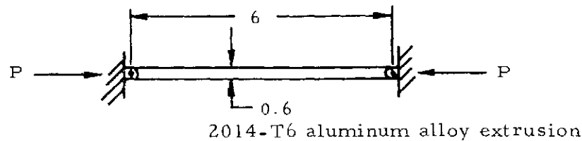
Figure 2-35. Pinned End Column in Axial Load
