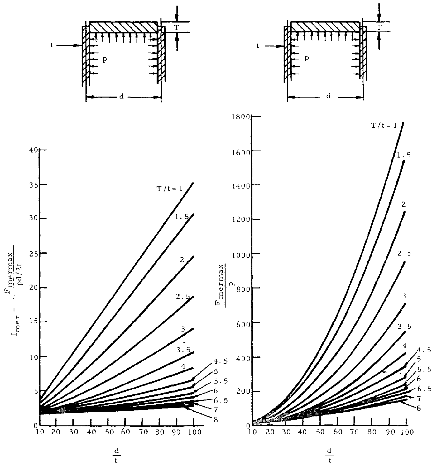
Figure 8-12. Graphical Presentation of Equation (8-11) for n = 0 *
