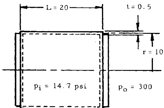
Figure 8-25. Cylinder Under External Pressure
