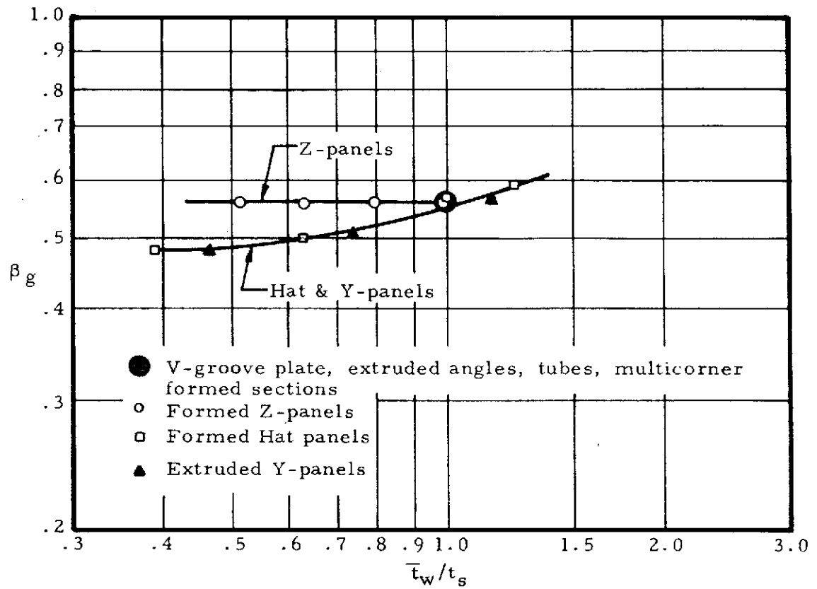
Figure 6-18. Crippling Coefficients for Angle-Type Elements
