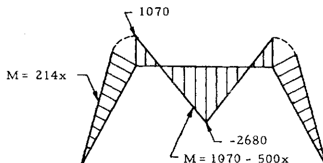
Figure 5-17. Moment Diagram for Trapezoidal Frame
