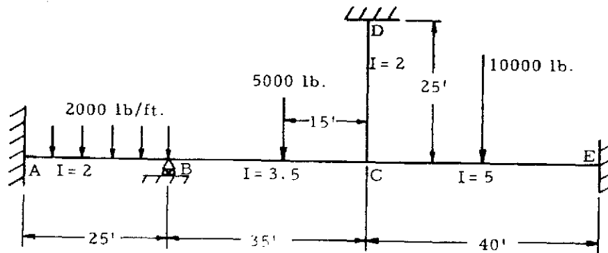
Figure 5-4. Frame
