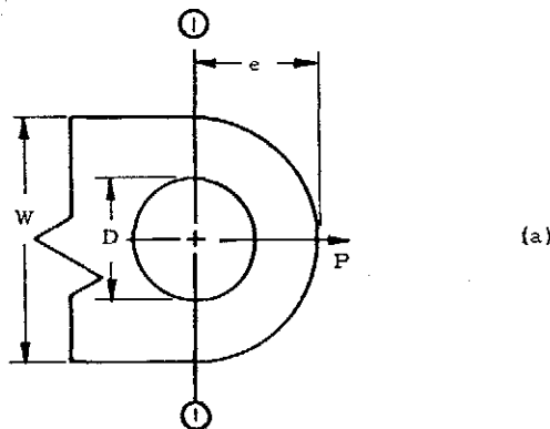
Figure 9-4. Net Tension Stress Coefficient
