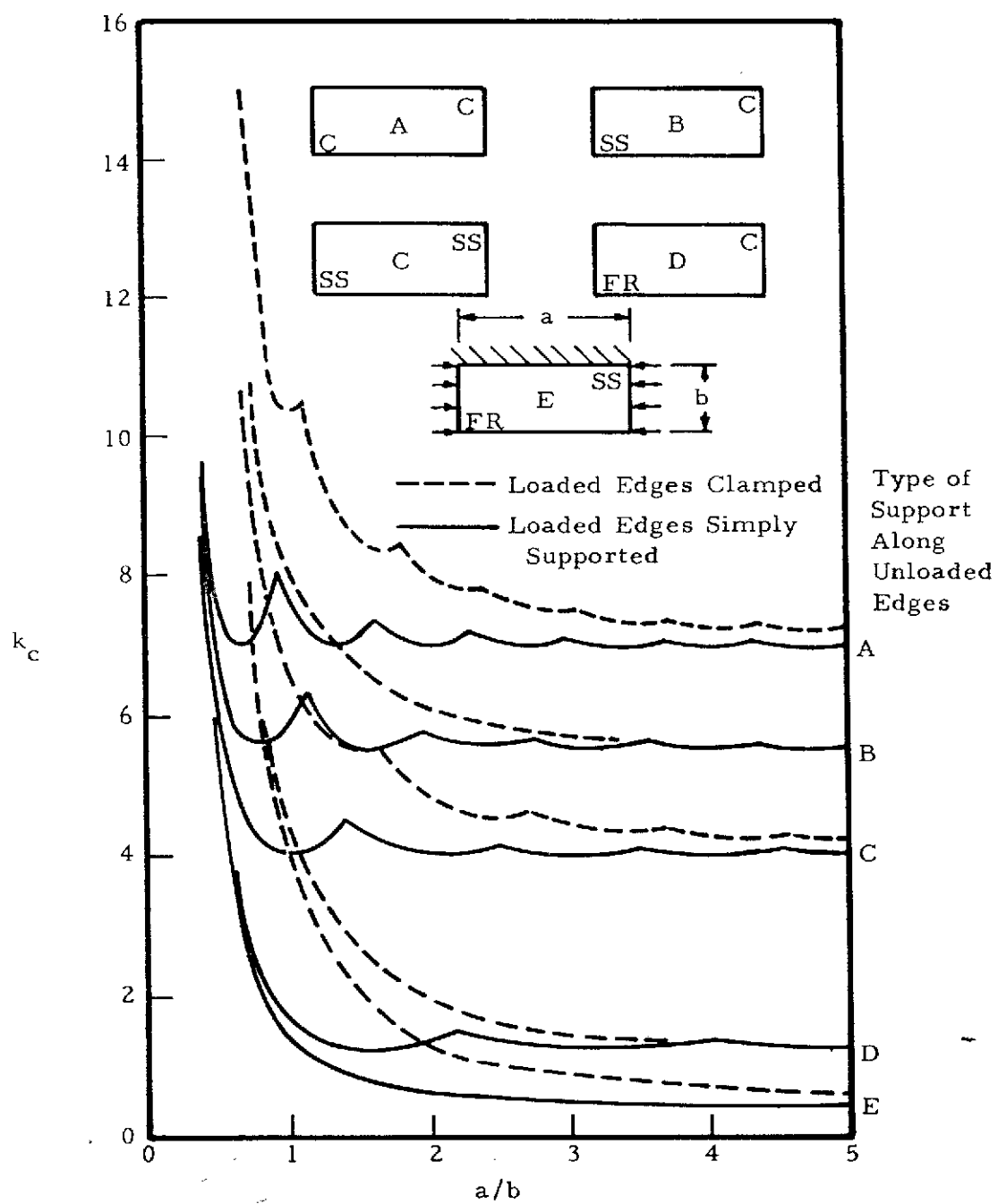
Figure 6-1, Compressive-Buckling Coefficients for Flat Rectangular Plates
