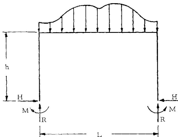
Figure 5-9. Free-Body Diagram of the Frame in Figure 5-8
