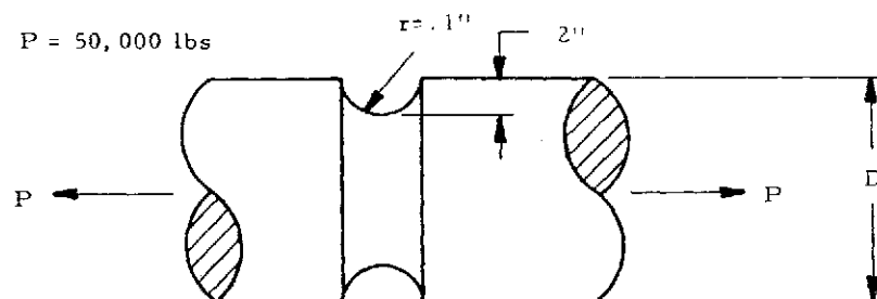
Figure 3-13. Bar with U-Notch under Static Tensile Load
