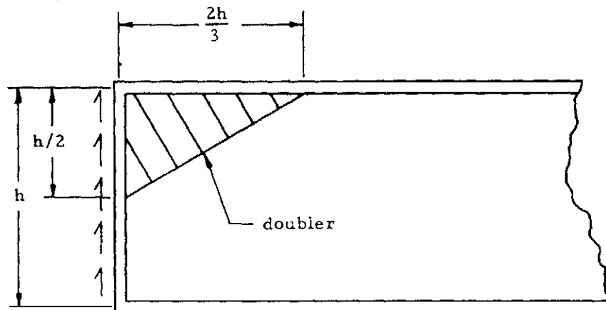
Figure 1-26. Doubler at the End of a Partial Tension Field Beam
