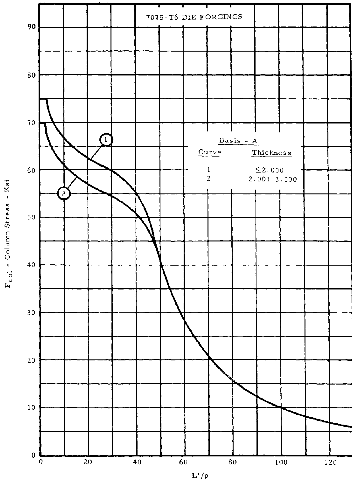
Figure 2-9. Column Allowable Curves
