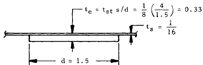
Figure 1-61. Doubler Equivalent to Beam Stiffeners
