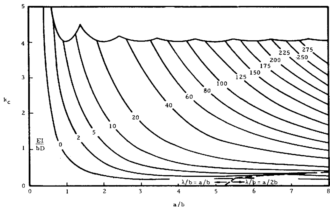
(i) Three Stiffeners A/bt = 0.4
