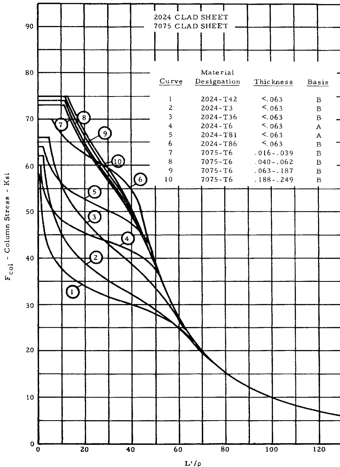
Figure 2-8. Column Allowable Curves
