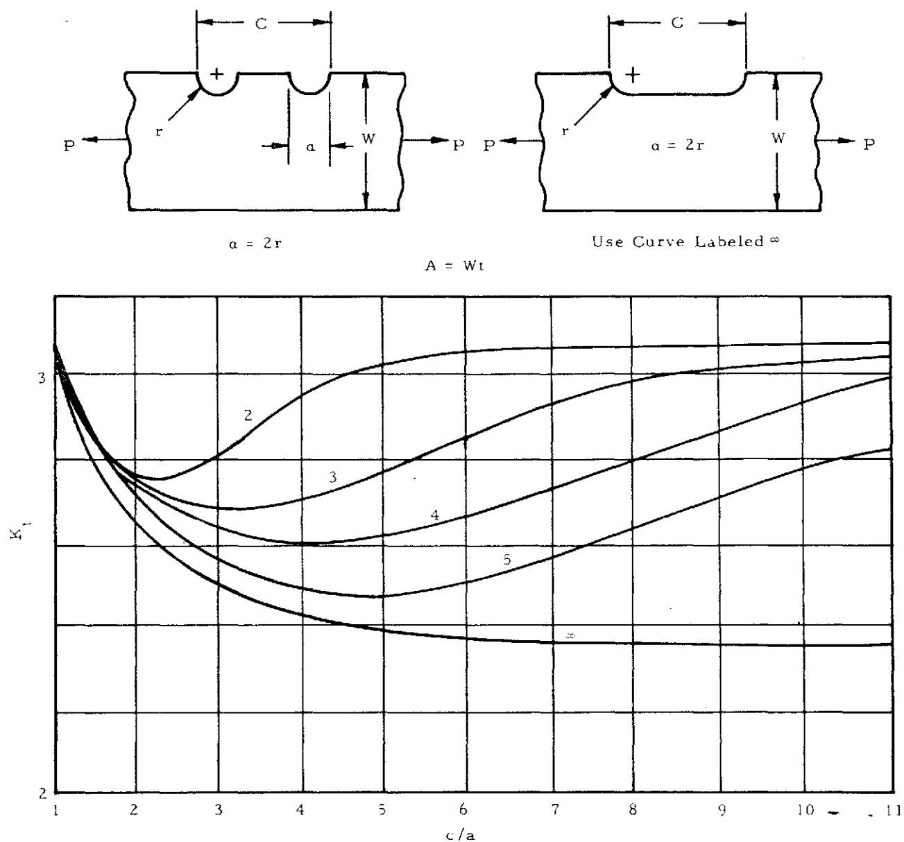
Figure 3-8. Rectangular Bar with Multiple Semicircular Notches on One Side
