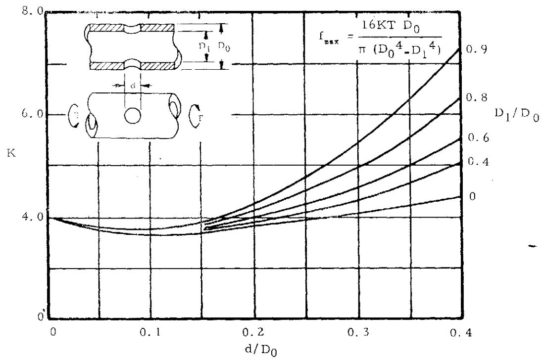
b. Shaft in Torsion
