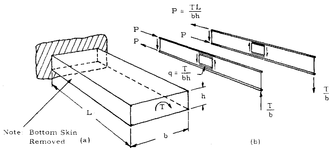
Figure 1-62. Illustration of the Effect of a Cutout
