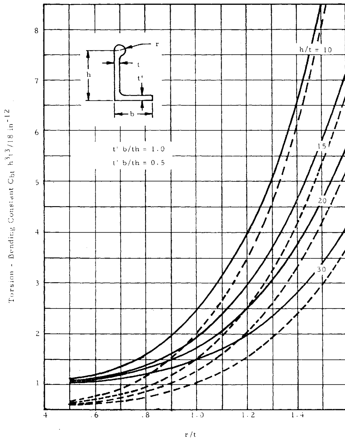
Figure 2-58. Torsion - Bending Constant of Bulb Angle - About Shear Center
