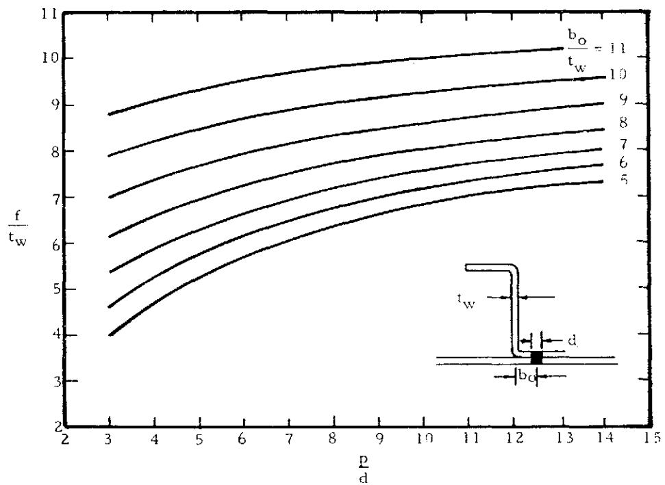
Figure 6-20. Experimentally Determined Values of Effective Rivet Offset
