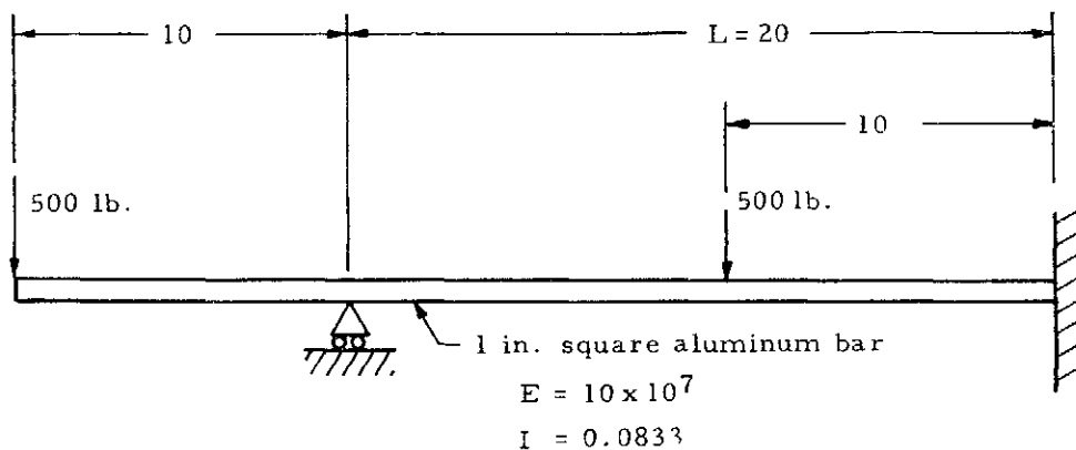
Figure 1-32. Beam with One Fixed End and One Pinned Support
