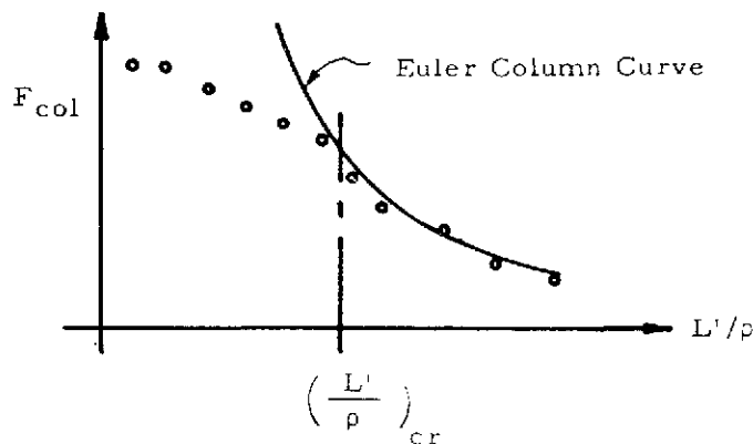
Figure 2-2. Typical Column Failure Curve
