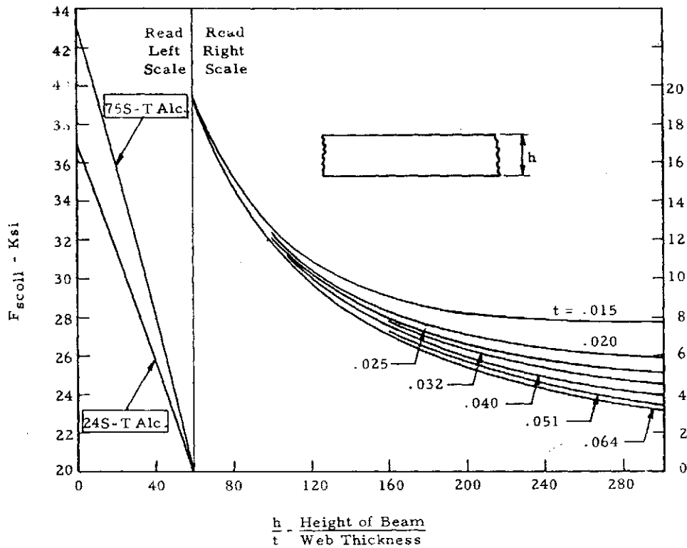
Figure 1-9. Collapsing Shear Stress, F_{scoll} , for Solid Webs of 24S-T and 75S-T Alclad Sheet
