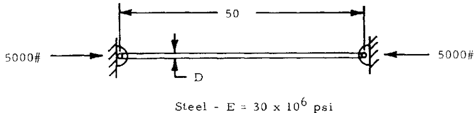
Figure 2-47. Column Loading for Study of Eccentricity
