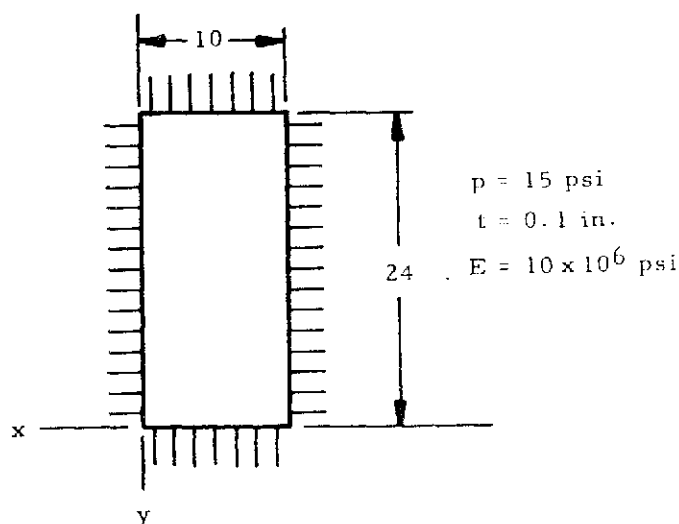
Figure 7-12. Short Rectangular Membranes
