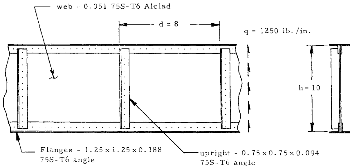
Figure 1-27. Partial Tension Field Beam with Single Uprights
