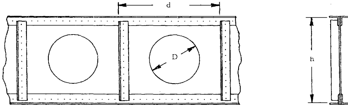
Figure 1-28. Partial Tension Field Beam with Access Holes
