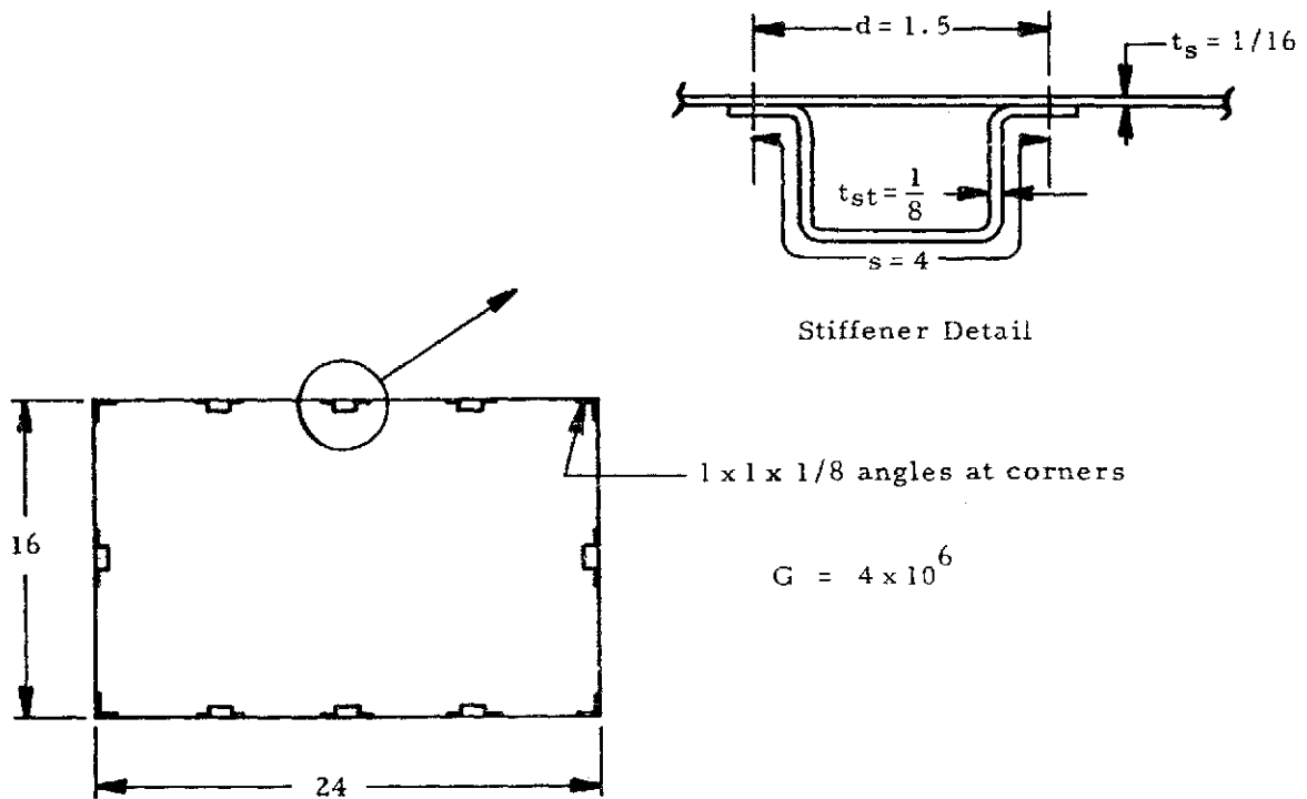
Figure 1-60. Cross Section of Stiffened Single Cell Open Beam
