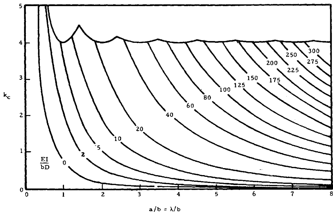
(l) Infinite number of stiffeners A/bt = 0.4
