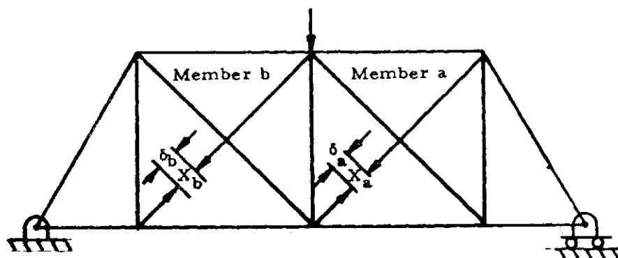
Figure 4-8. Statically Indeterminate Truss With Two Redundancies
