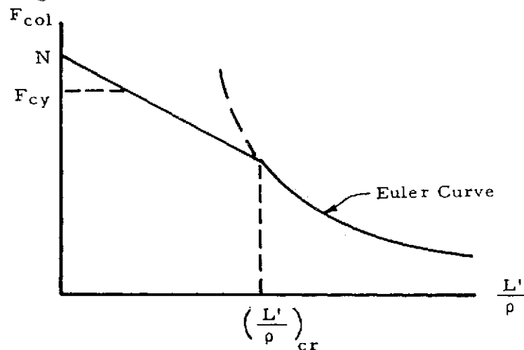
Figure 2-51. Typical Straight Line for Short Columns
