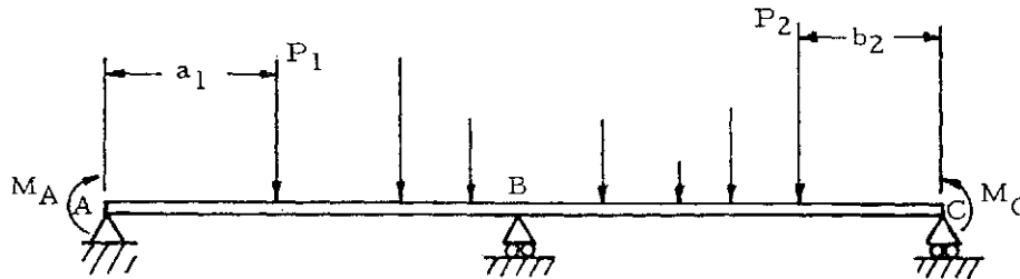
Figure 1-36. Continuous Beam Under Several Concentrated Loads
