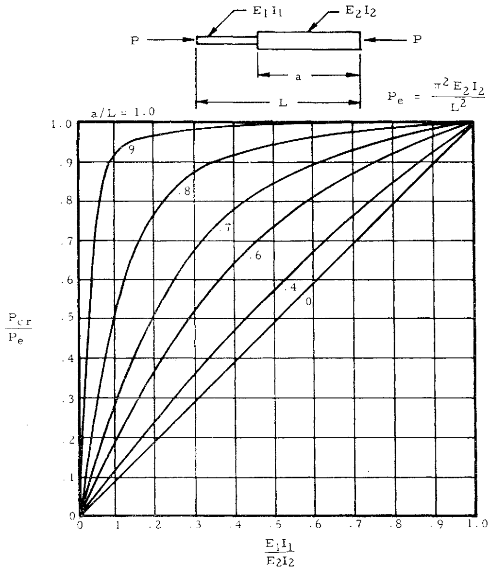
Figure 2-79. Critical Loads for Unsymmetrical Stepped Columns
