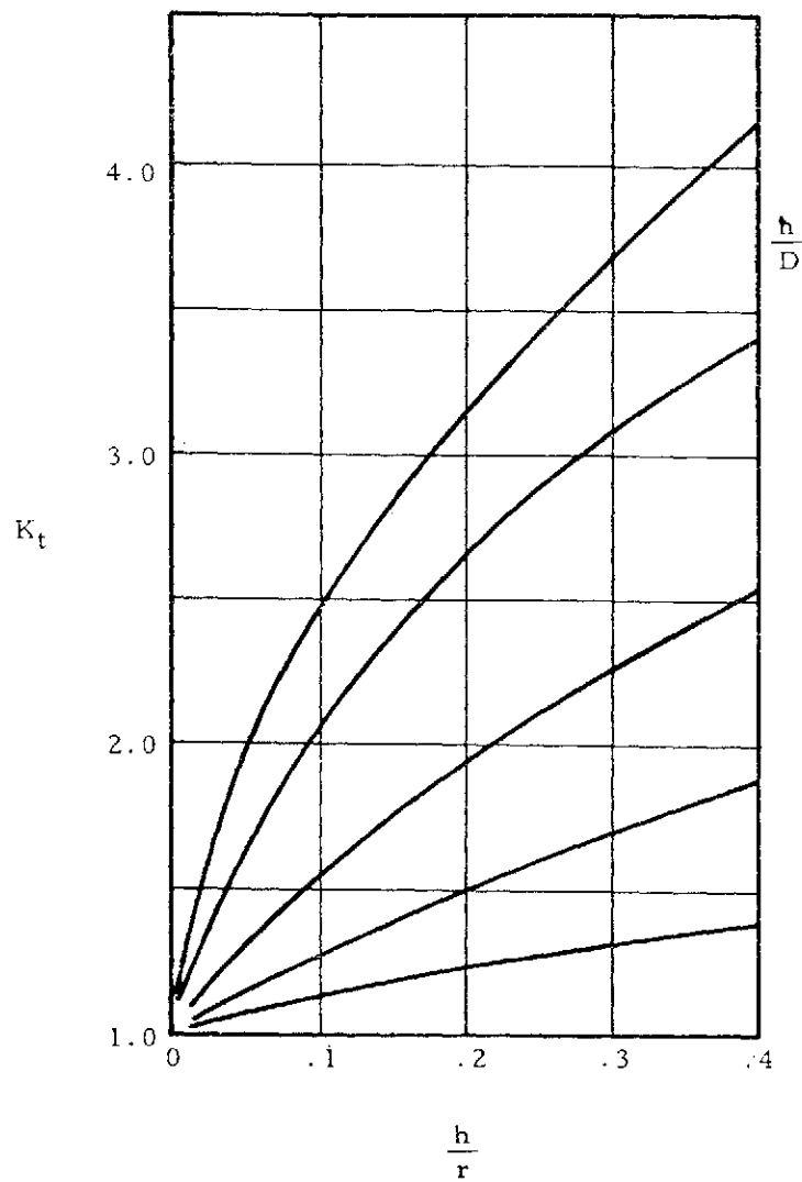
Figure 3-2. Round Bar with U Notch
