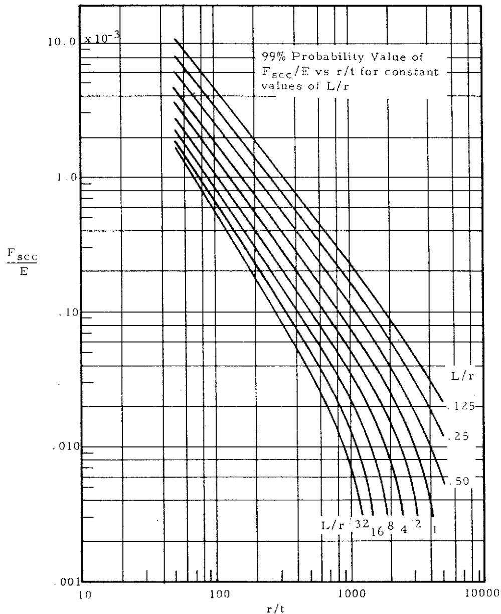
Figure 8-33. Torsional Buckling of Unpressurized Circular Cylinders
